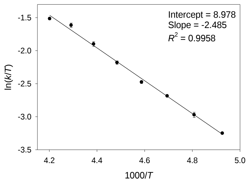
Figure 2.9. Eyring plot of the Me_E Me_F exchange in 1 yielding activation parameters for the exchange.
