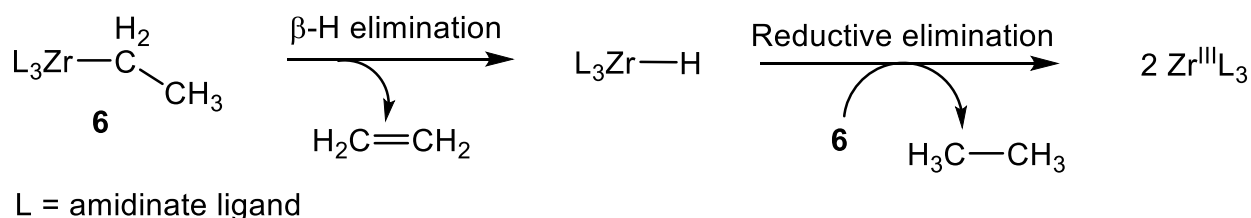
Scheme 3.4. \beta -hydrogen elimination in 6 releasing ethylene followed by the formation of ethane via reductive elimination between an additional molecule of 6 and Zr[MeC(N^iPr)_2]_3H .
