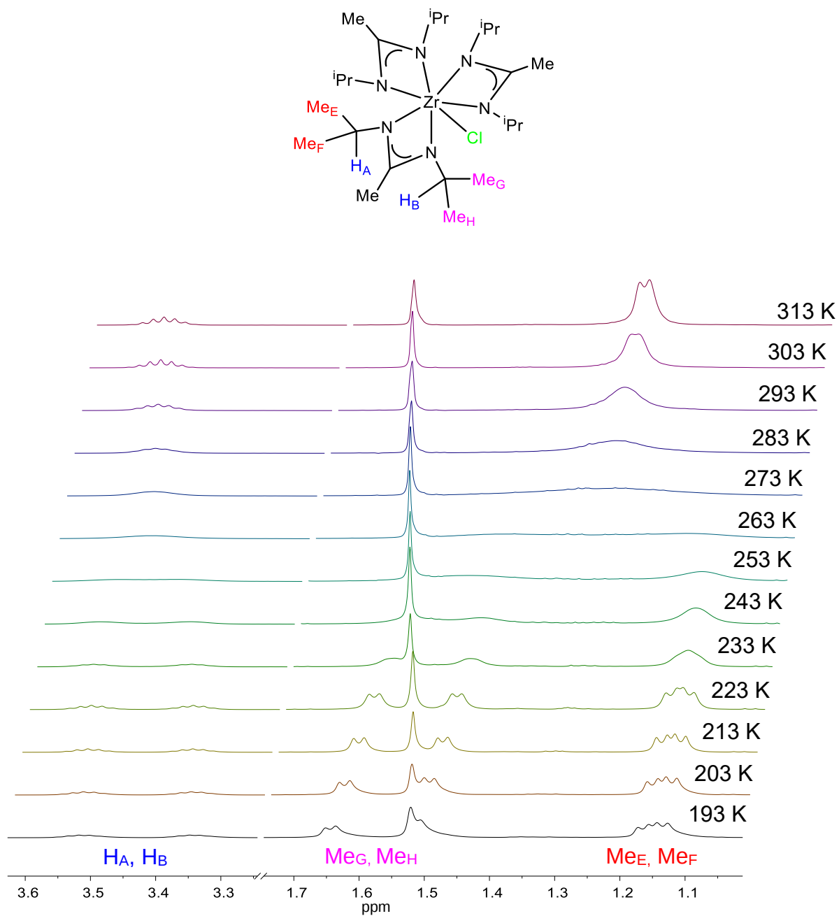
Figure 2.7. Partial 1 H NMR spectra of 1 at several temperatures showing the de-coalesce of the methyl and H atom peaks pertaining to the CHMe 2 groups as the temperature is lowered from room temperature to 193 K. As the temperature is raised to 313 K, the broad peak for the CHMe 2 groups becomes a doublet.
