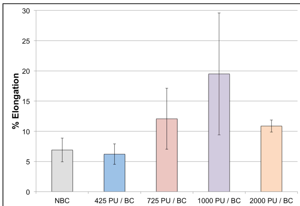
Figure 57: Percent Elongation at Fracture of BC and PU/BC Composites
