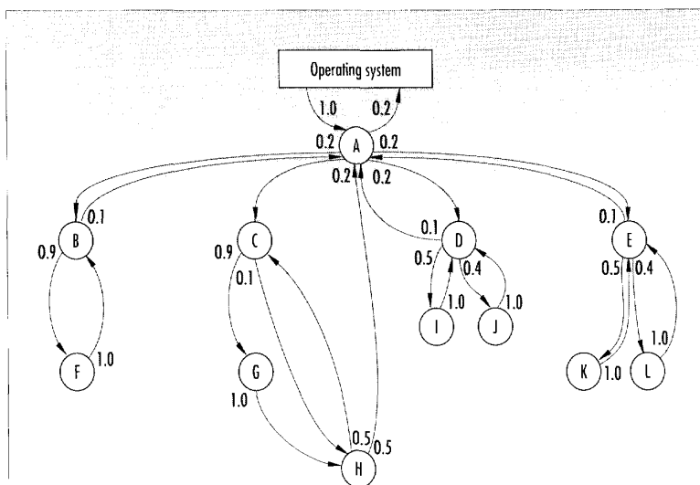
Figure 1. A software system as a network of components. Each directed arc, labeled with its transition probability, indicates that control passes from one component to another in the direction of the arrow.
