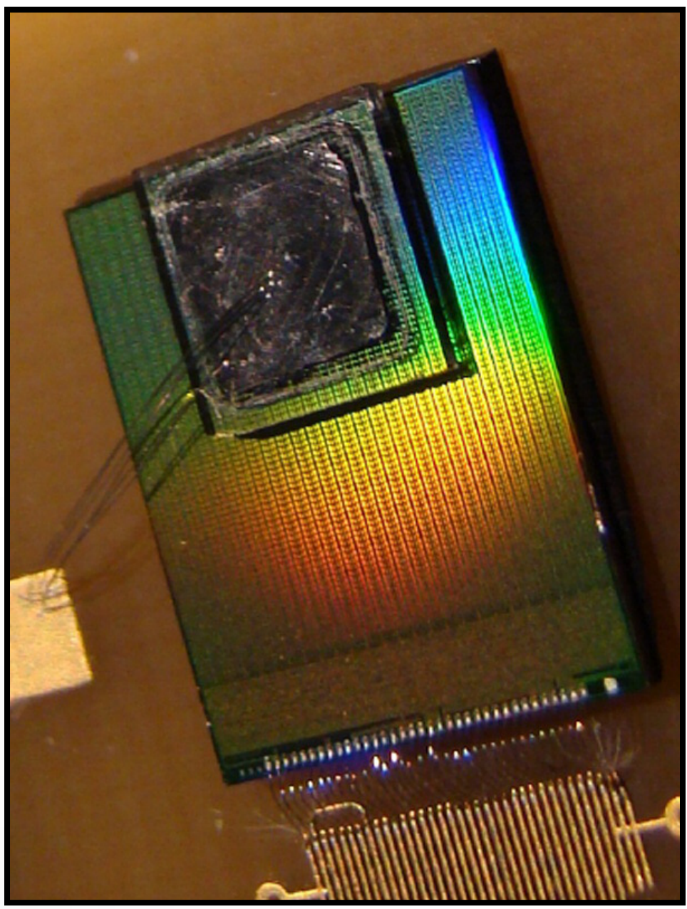
A Fully Assembled Detector Plane.
