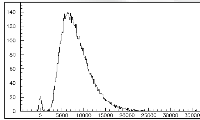
Charge deposit from Sr90 for Poly-Crystal CVD Diamond
