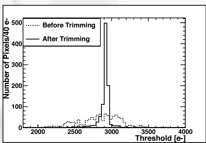
Typical threshold settings for the PSI46 readout chip. The threshold of 3000 e- is well separated from the Single-Crystal MPV of ~18000 e-.
