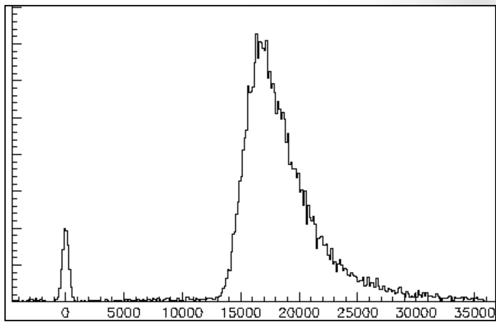
Single-Crystal CVD diamond charge deposit from a Sr90 source (~minimum ionizing)
