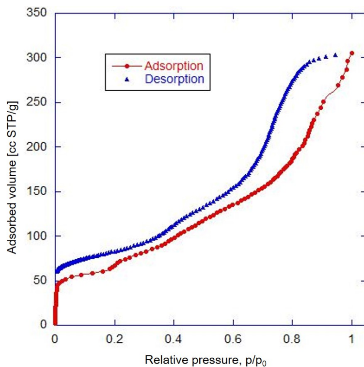
Figure D.45: Adsorption and desorption isotherms of \text{CH}_4/\text{CNT} at 77 K. The interpolating line is meant to guide the eye.
