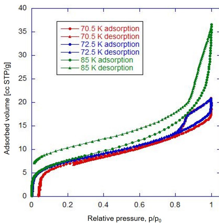
Figure D.40: Compilation of CH 4 isotherms (adsorption and desorption) on 100 nm size silica for several temperature values.
