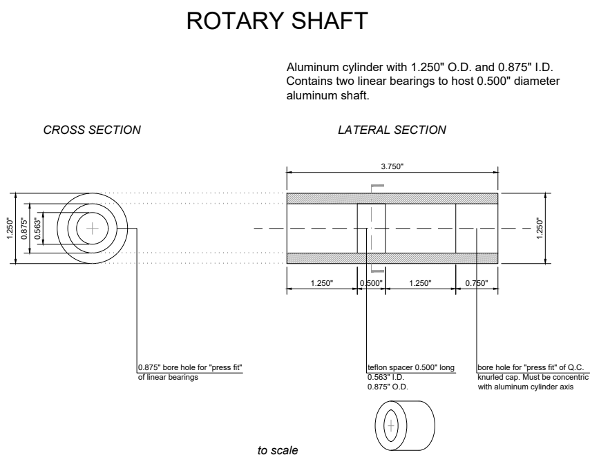
Figure A.1: Schematic drawing of the rotary shaft assembly to house the aluminum shaft that connects dc-motor for spinning of the SS tumbler.
