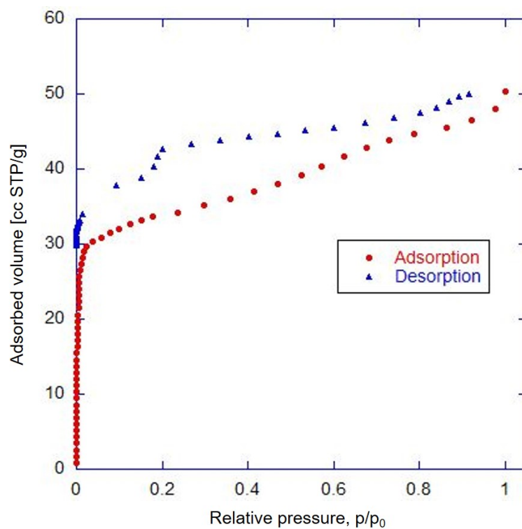
Figure 5.8: Adsorption and desorption isotherms of \text{CH}_4/\text{IV} dipeptide at 90 K. The adsorption curve has the characteristic shape which is common to the other dipeptide-based materials.
