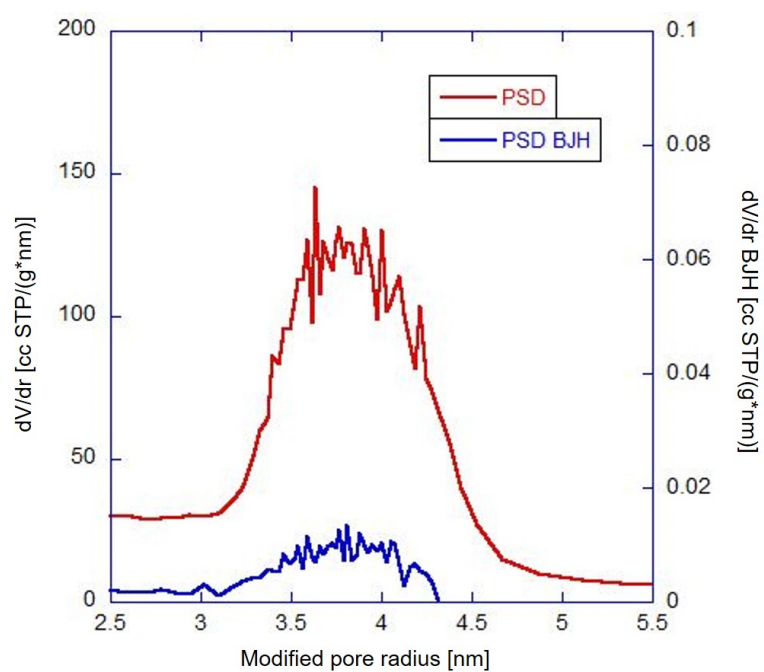
Figure D.57: PSD from adsorbed volume and BJH volume calculated from the desorption isotherm of Fig. D.54 ( \text{CH}_4/\text{SBA-15} ).
