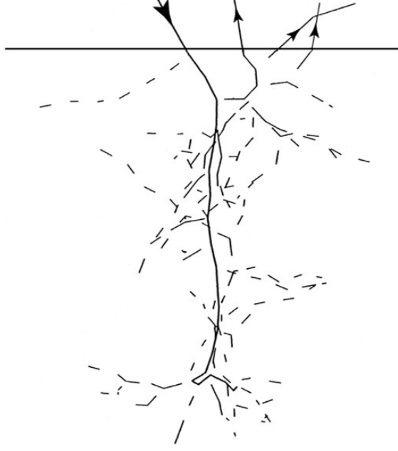
Figure 2.3: Simulation of a collision cascade initiated by a 1 keV Ar ion at 30^\circ incidence on a Ni substrate leading to three sputtered atoms [5].
