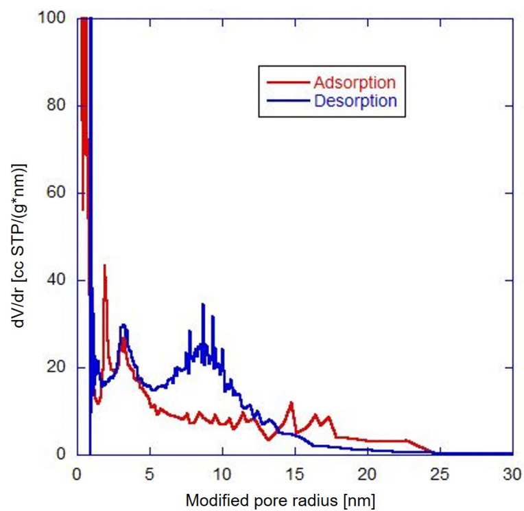
Figure D.46: PSD plot for the isotherms reported in Fig. D.45.
