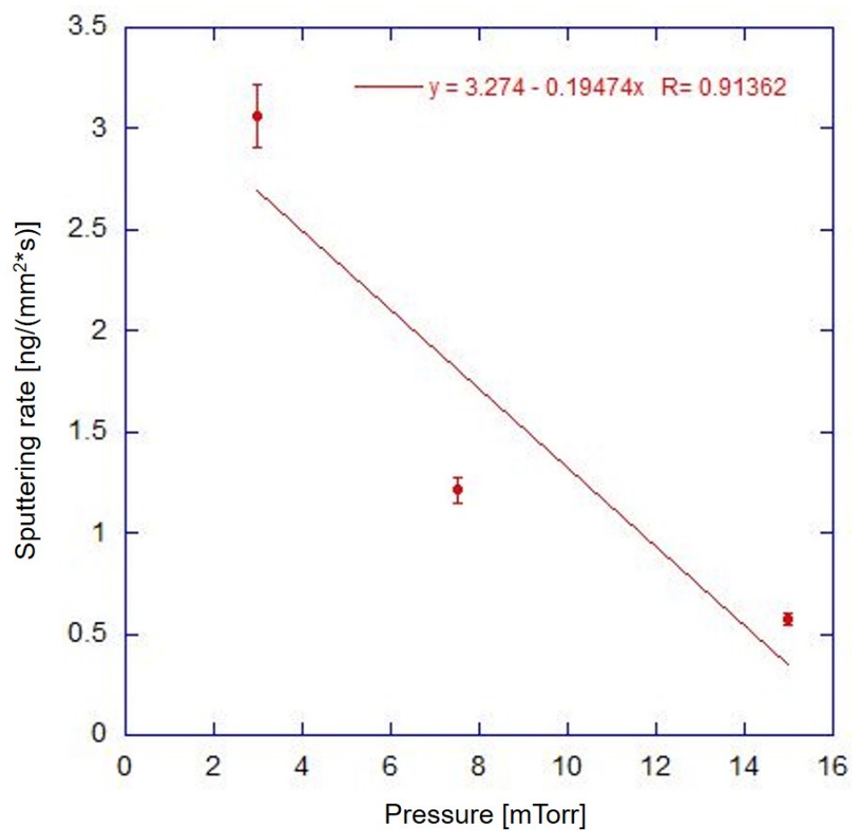
Figure A.11: Sputtering rate as a function of pressure at 100 W for Cu.
