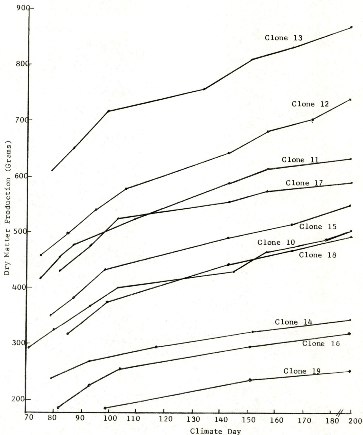
Figure 2. Cumulated dry matter yields (grams) of 10 orchardgrass clones grown in 1964.
