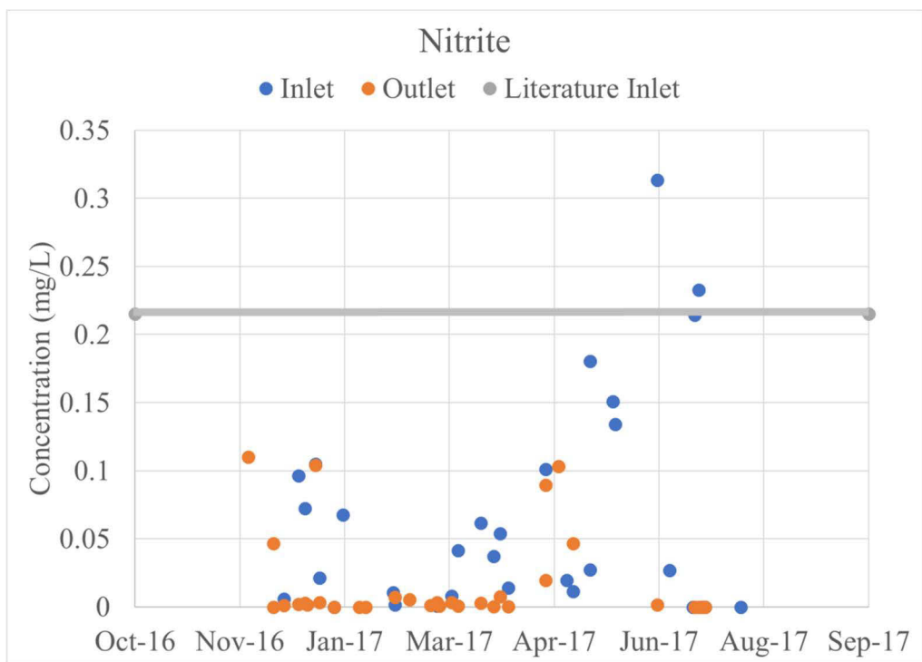
Figure 3.13 Inlet and Outlet Nitrite Concentrations
