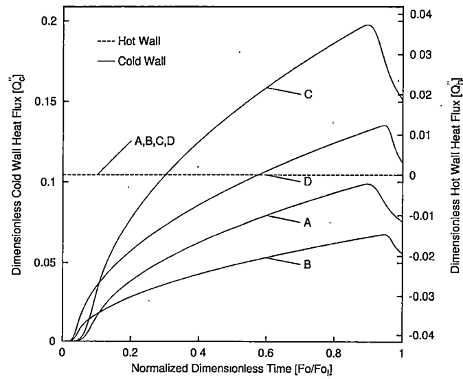
(b) Heat flux histories, Q_c''(Fo/Fo_l) , Q_h''(Fo/Fo_l) .
