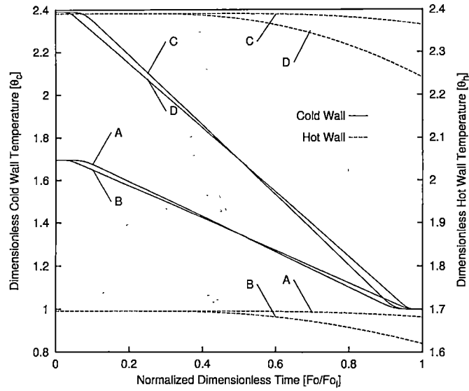
(a) Boundary temperature histories, \theta_c(Fo/Fo_l) and \theta_h(Fo/Fo_l) .
