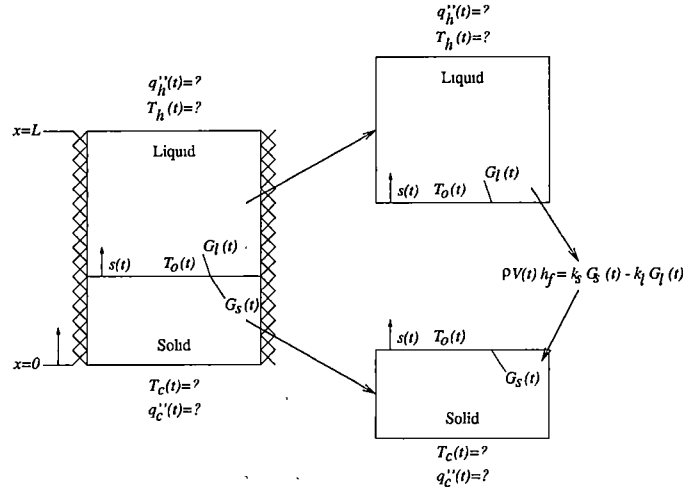
Figure B.1: Schematic of the pure melt solidification design problem illustrating the splitting of the solid and liquid domains.
