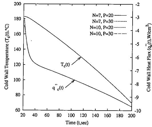
(b) Cold wall predictions: T_c(t) , q''_c(t) .
