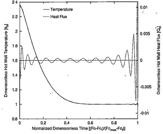
(b) \theta_i = 2.391 , For_l = 0.124 , G_{l_d}^L = 1.400 .
