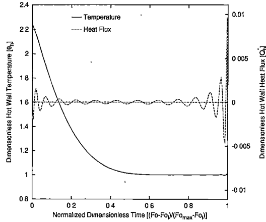
(c) \theta_i = 2.391 , For_l = 0.247 , G_{l_d}^L = 1.247 .
