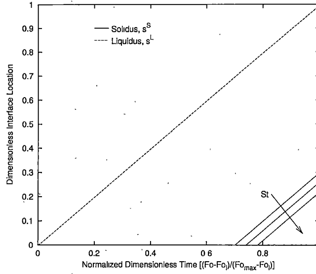
(a) \theta_i = 2.391 , Fo_l = 0.124 , and G_{l_d}^L = 1.241 .
