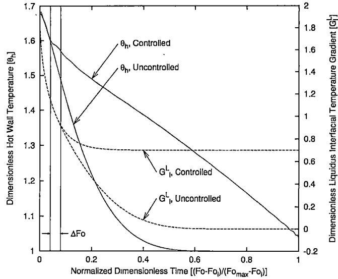
Figure 5.9: Illustration of the diffusion induced lag time encountered in the resolution of the inverse liquid solidification sub-problem for dimensionless values \theta_i = 1.695 , Fo_i = 0.124 , V_d^L = 0.424 , G_{l_d}^L = 0.700 .
