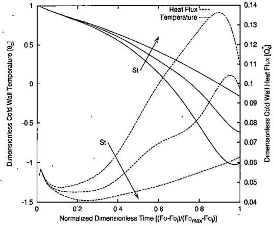
(b) \theta_i = 1.695 , Fo_i = 0.247 , and G_{l_d}^L = 0.779 .
