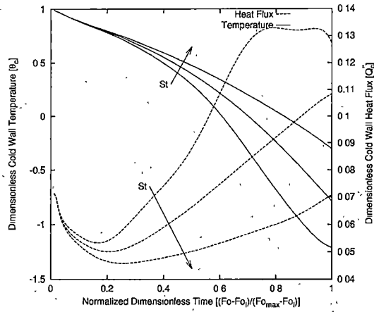
(a) \theta_i = 1.695 , Fo_i = 0.124 , and G_{l_d}^L = 0.871 .
