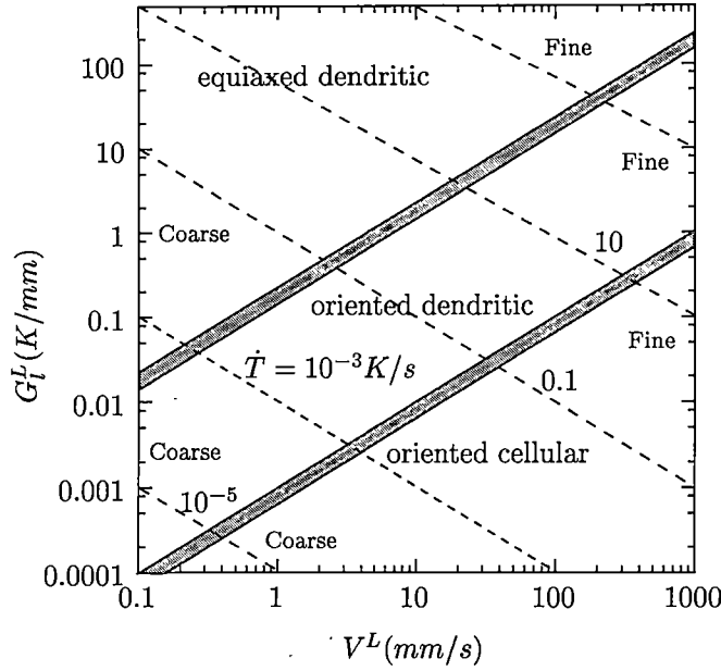
Figure 1.1: VG map for a typical alloy undergoing unidirectional solidification. Adapted from [1].
