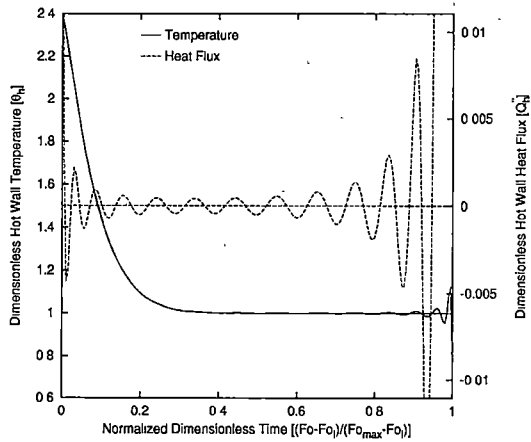
(c) \theta_i = 2.391 , Fo_i = 0.124 , G_{L_d}^L = 1.241 .
