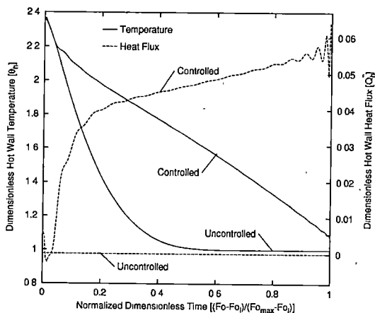
(c) \theta_i = 2.391 , Fo_l = 0.124 , and G_{ld}^L = 1.400 .
