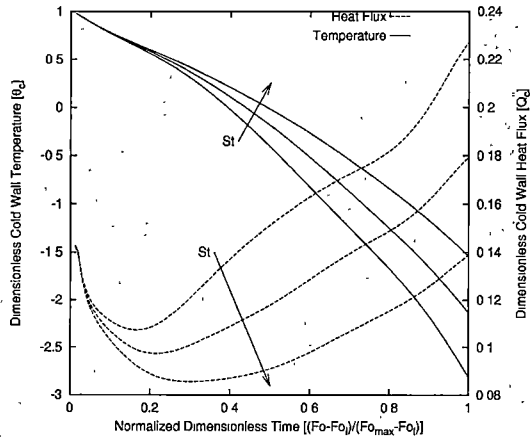
(c) \theta_i = 2.391 , Fo_i = 0.124 , and G_{l_d}^L = 1.742 .
