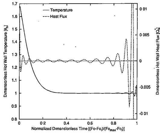
(a) \theta_i = 1.695 , Fo_i = 0.124 , G_{L_d}^L = 0.621 .
