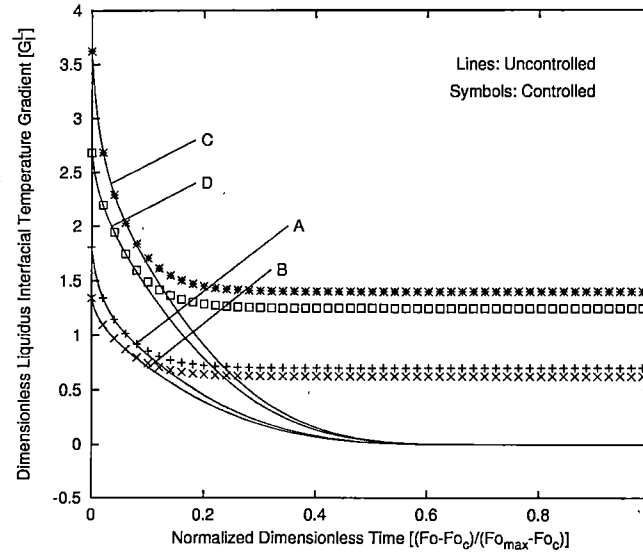
Figure 5.5: Comparison of direct (uncontrolled) and design (controlled) liquidus interfacial temperature gradients, G_L^L((Fo - Fo_l)/(Fo_{max} - Fo_l)) for a dimensionless liquidus interfacial velocity of V_d^L = 0.424 .
