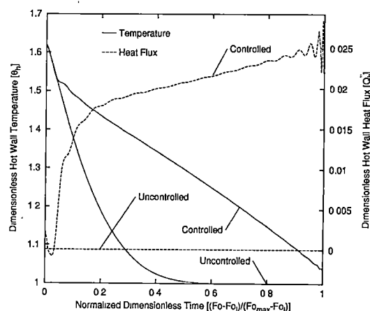
(b) \theta_i = 1.695 , Fo_l = 0.247 , and G_{ld}^L = 0.623 .
