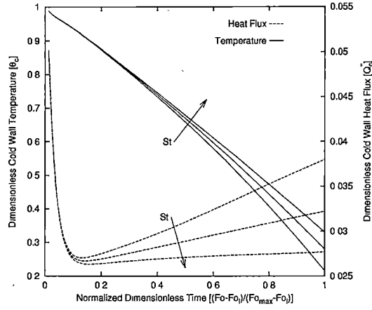
(a) \theta_i = 1.695 , Fo_l = 0.124 , and G_{ld}^L = 0.621 .
