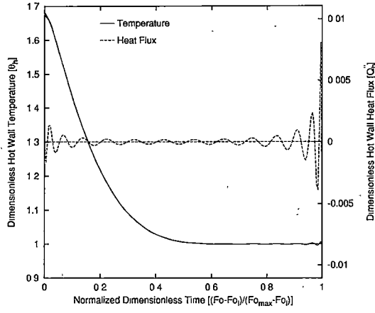
(a) \theta_i = 1.695 , For_l = 0.124 , G_{l_d}^L = 0.700 .
