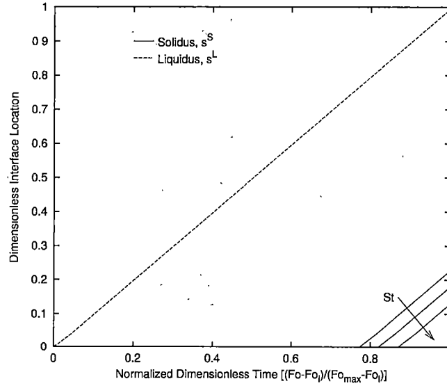
(b) \theta_i = 2.391 , Fo_l = 0.247 , and G_{l_d}^L = 1.103 .
