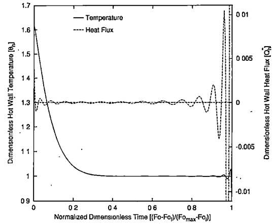
(b) \theta_i = 1.695 , Fo_i = 0.247 , G_{L_d}^L = 0.551 .
