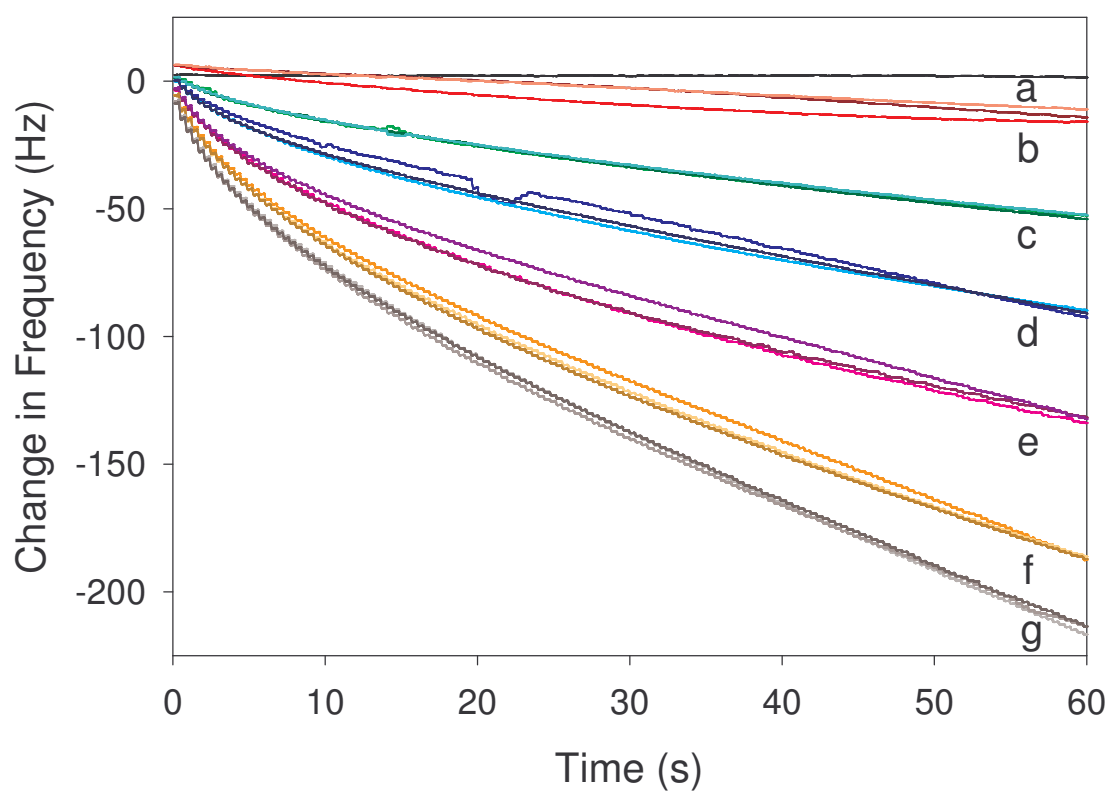
Figure 4.3. Frequency changes for the deposition of Pd from various \text{PdCl}_2 concentrations: (a) baseline; (b) 0.0156 mM; (c) 0.0780 mM; (d) 0.156 mM; (e) 0.234 mM; (f) 0.312 mM; (g) 0.390 mM. Three separate deposition measurements were run for each concentration.
