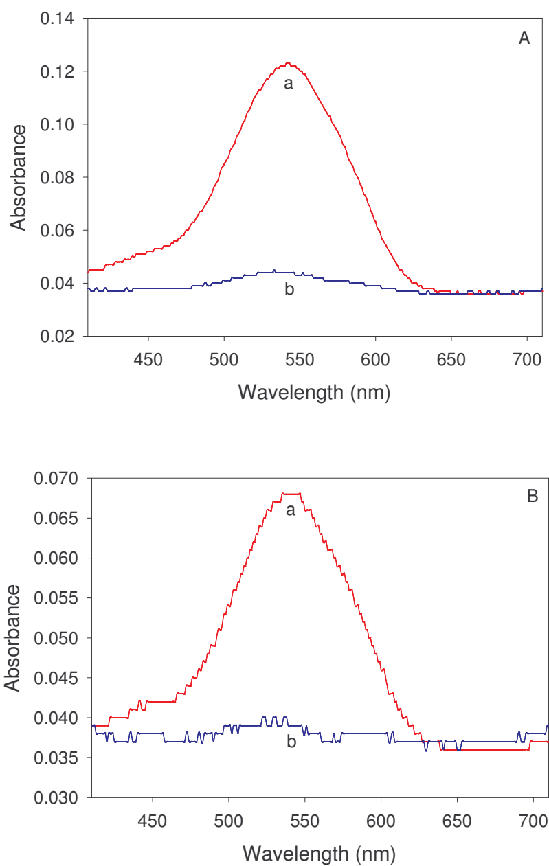
Figure B.7. (A) Spectra of a 156 ppb Cr(VI) solution before (a) and after (b) exposure to a pyridine-functionalized monolith. (B) Spectra of a 59 ppb Cr(VI) solution before (a) and after (b) exposure to a pyridine-functionalized monolith.
