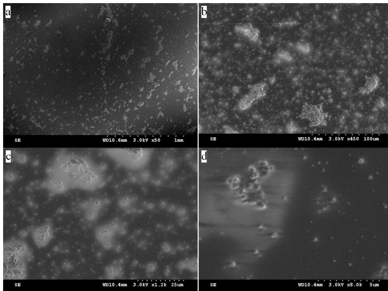
Figure 2.3. SEM images of a pyridine-functionalized sol-gel deposited on a gold QCM surface. Images taken are at magnifications of: (a) 1 mm; (b) 100 \mu m; (c) 25 \mu m; (d) 5 \mu m.
