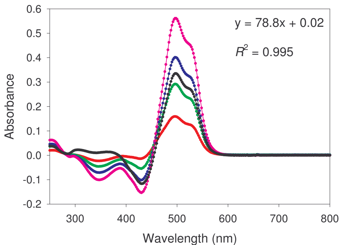
Figure C.2. UV-vis absorption spectra for \text{Pd}^{2+} determination using N,N-dimethyl-4-nitrosoaniline. The spectra were obtained from: (●) 0.00167 mM \text{Pd}^{2+} ; (●) 0.00334 mM \text{Pd}^{2+} ; (●) 0.00501 mM \text{Pd}^{2+} ; (●) 0.00668 mM \text{Pd}^{2+} ; (●) \text{Pd}^{2+} sample.
