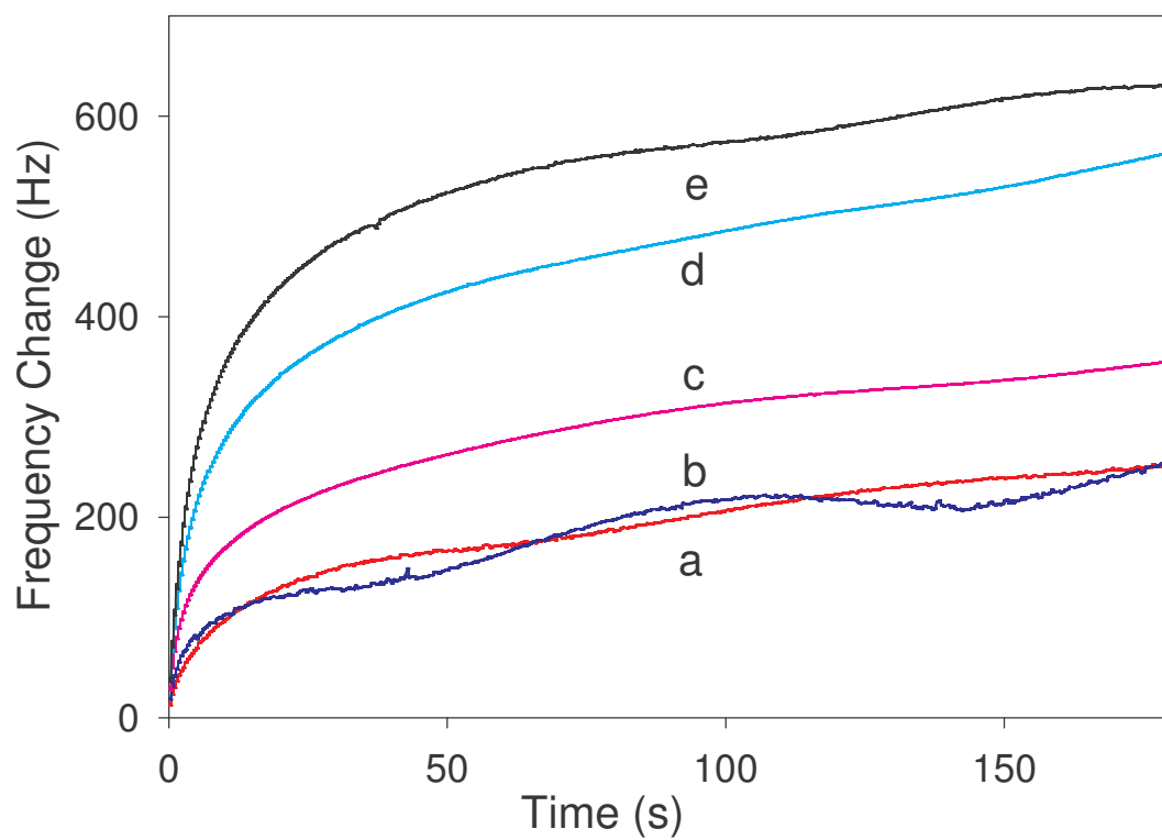
Figure 4.5. Frequency changes for Pd stripping after deposition from PdCl 2 solutions of varying concentrations: (a) 0.0780 mM; (b) 0.156 mM; (c) 0.234 mM; (d) 0.312 mM; (e) 0.390 mM.
