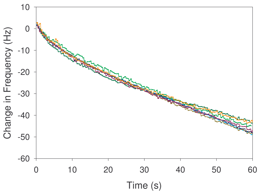
Figure C.1. Seven deposition measurements carried out involving 0.0780 mM \text{Pd}^{2+} solution. The relative standard deviation for the measurements is 4.15%.
