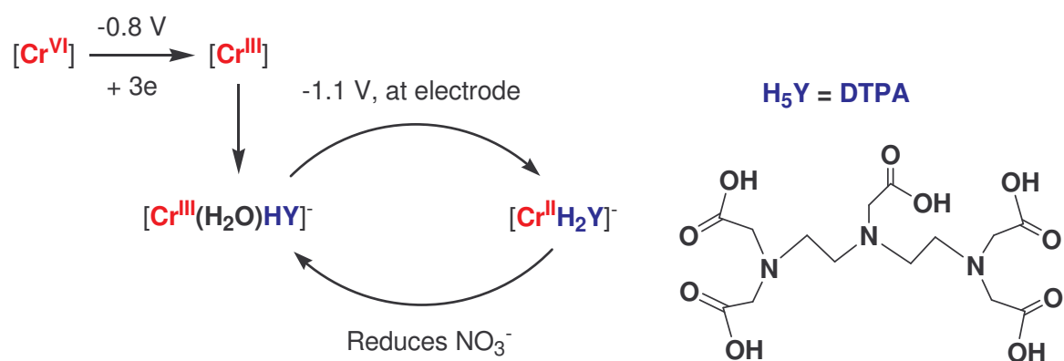
Figure 6.1. CAdSV process for the analysis of Cr(VI) at a bismuth film electrode. 3,4
