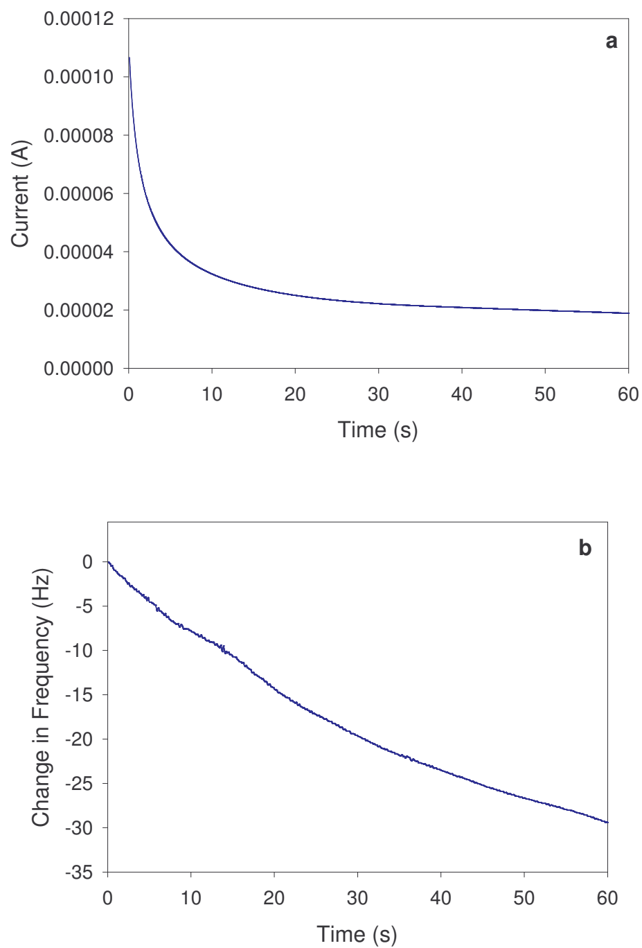
Figure 2.2. (a) Current-time and (b) frequency-time plots at a gold QCM electrode in a TMOS/2-[2-(trimethoxysilyl)ethyl]-pyridine sol solution when a potential of -0.9 V is applied.
