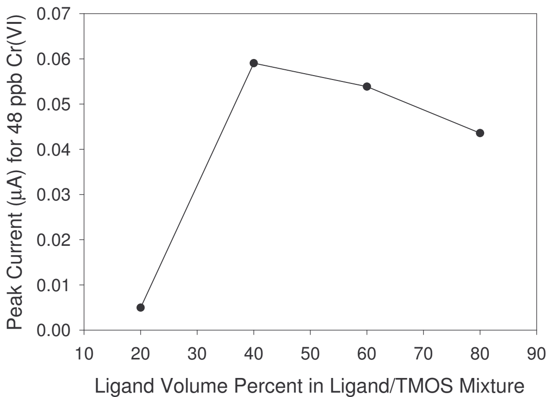
Figure A.5. Plot of the optimal volume percentage of 4-[2-(trimethoxysilyl)ethyl]-pyridine in the sol solutions used for electrode coating versus the peak current obtained using each coated electrode for the analysis of a 48 ppb Cr(VI) solution.
