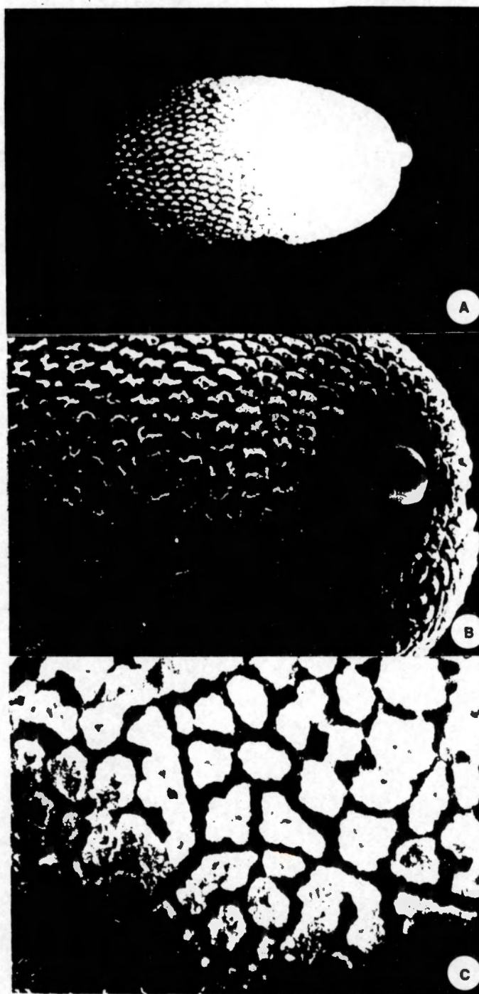
Figure 1. Egg of Hemerobius stigma Stephens. A, Egg of Hemerobius stigma (116 \times ); B, Surface of anterior pole showing waxlike projections and micropylar process (144 \times ); C, Tubercles and fissures on the micropylar surface (1200 \times ).
