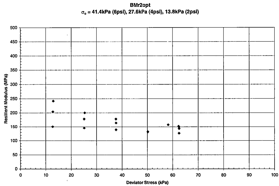
Graph B - 2 Resilient Modulus vs. Deviator Stress for Blount County – BMr2opt
