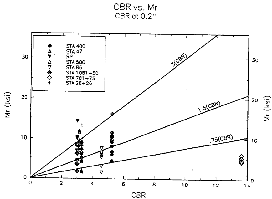
Figure 3. Relationship between M_r and CBR at 0.2".
