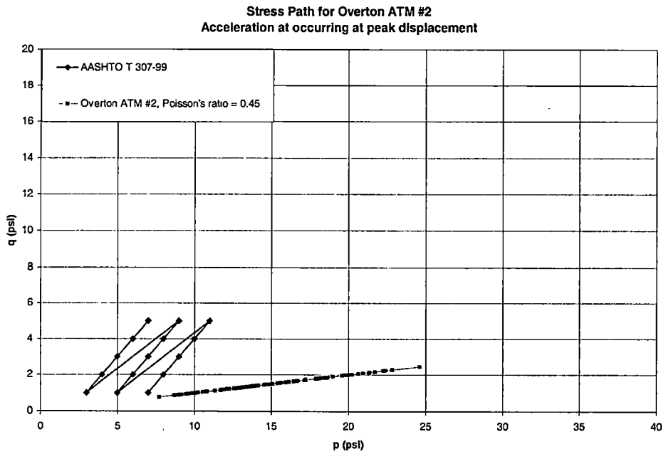
Graph C – 22 Stress Path for Overton ATM #2
