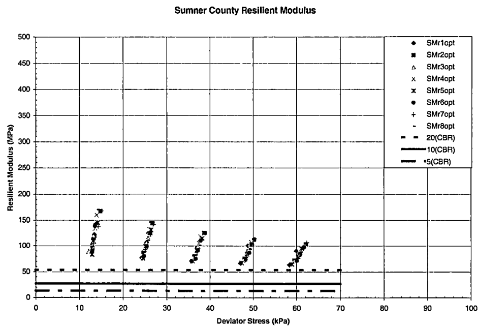
Figure 3-6 CBR Correlation with Sumner County
