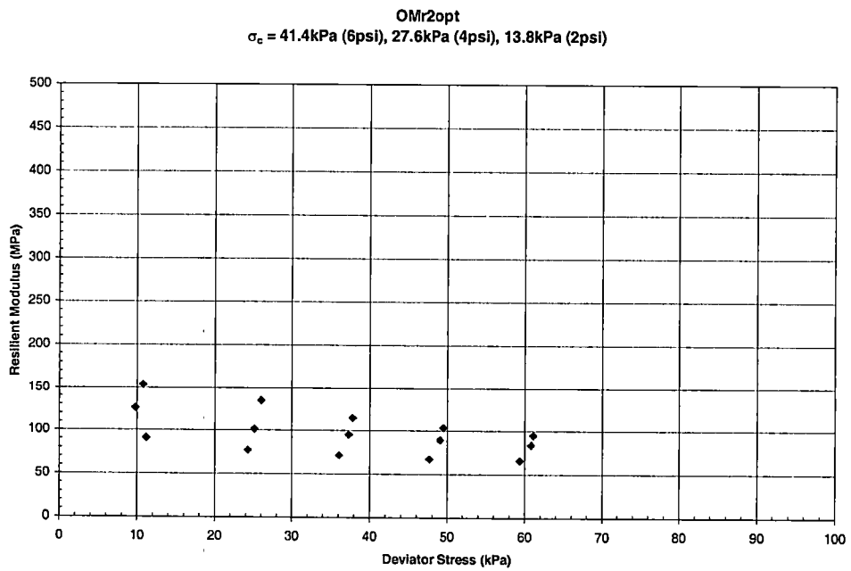
Graph B - 29 Resilient Modulus vs. Deviator Stress for Overton County – OMr2opt
