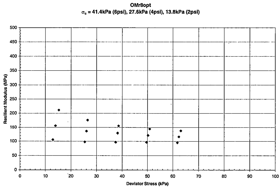
Graph B - 35 Resilient Modulus vs. Deviator Stress for Overton County – OMr8opt
