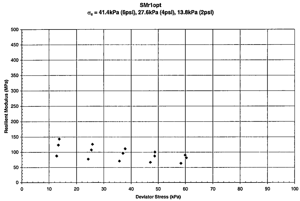
Graph B - 40 Resilient Modulus vs. Deviator Stress for Sumner County – SMr1opt
