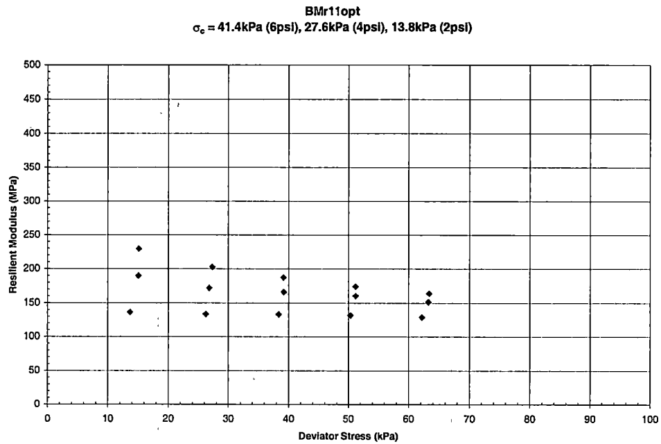
Graph B - 9 Resilient Modulus vs. Deviator Stress for Blount County - BMr11opt
