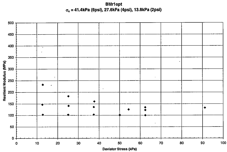
Graph B - 1 Resilient Modulus vs. Deviator Stress for Blount County - BMr1opt
