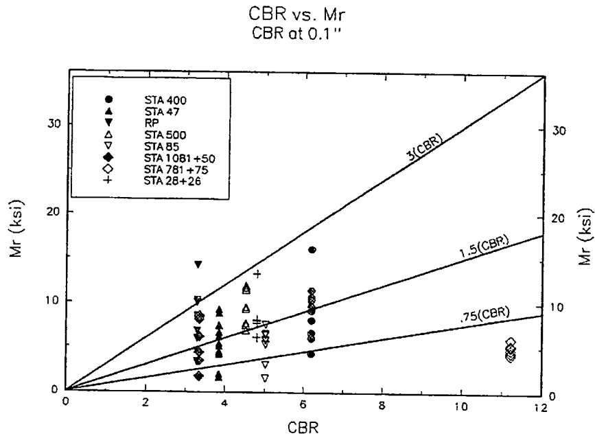
Figure 2. Relationship between M_r and CBR at 0.1".
