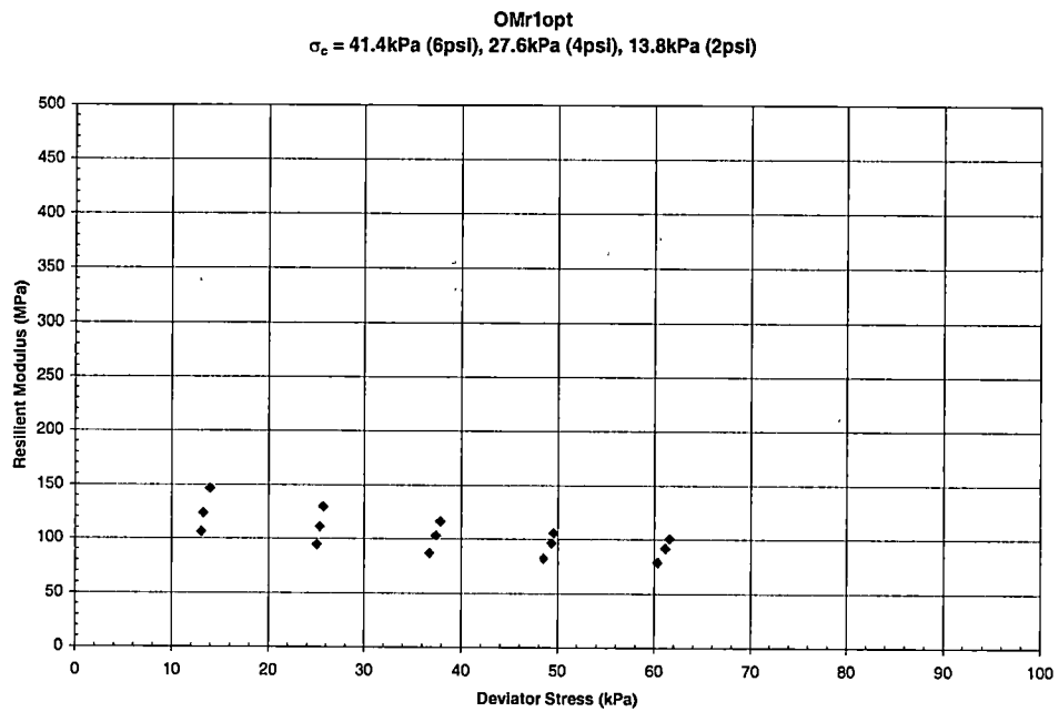
Graph B - 28 Resilient Modulus vs. Deviator Stress for Overton County – OMr1opt
