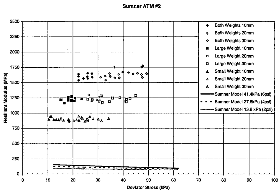
Figure 4-6 Typical ATM Result Using Double Integration Technique
