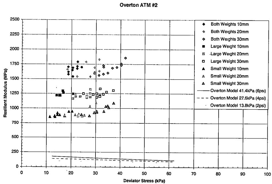
Graph C - 6 Resilient Modulus vs. Deviator Stress for Overton County Overton ATM #2 – Peak Acceleration
