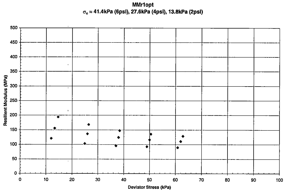
Graph B - 17 Resilient Modulus vs. Deviator Stress for McNairy County - MMr1opt
