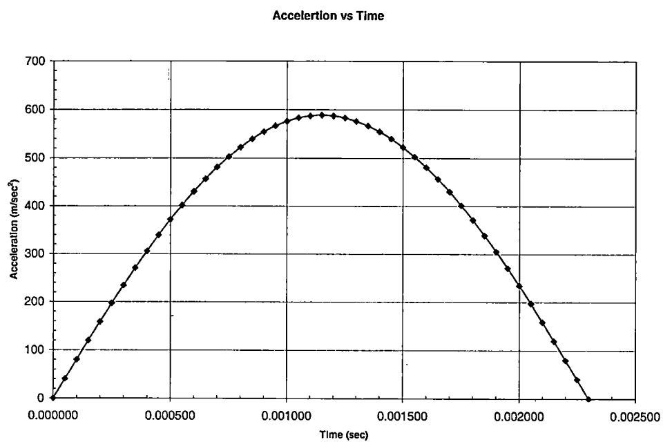
Graph F-1 Artificial Signal Used for Verification
