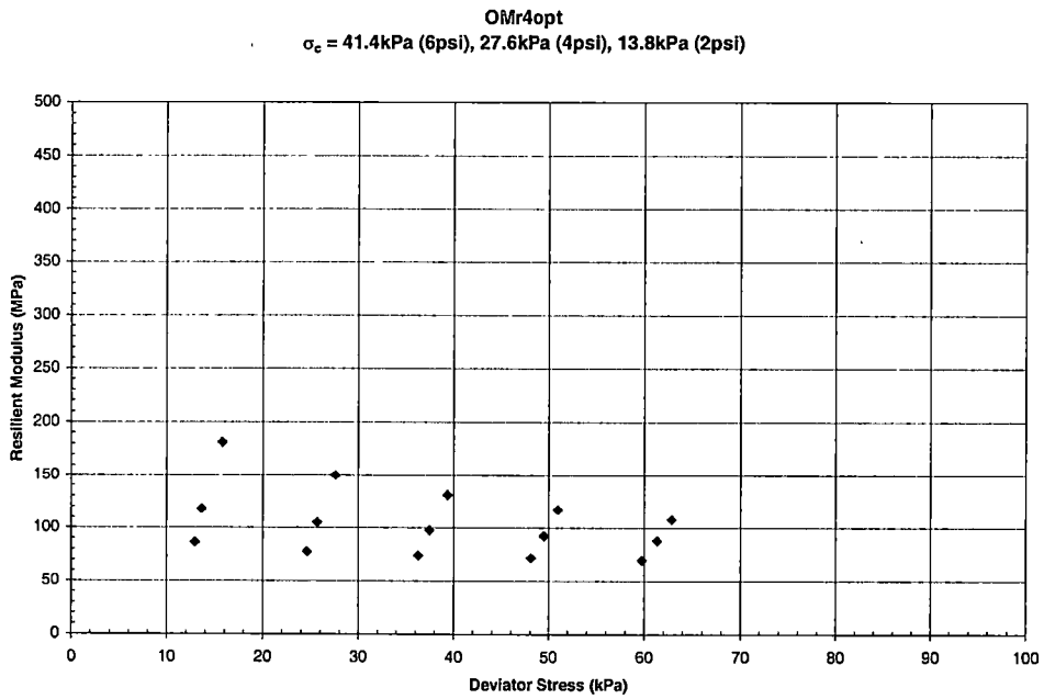
Graph B - 31 Resilient Modulus vs. Deviator Stress for Overton County – OMr4opt
