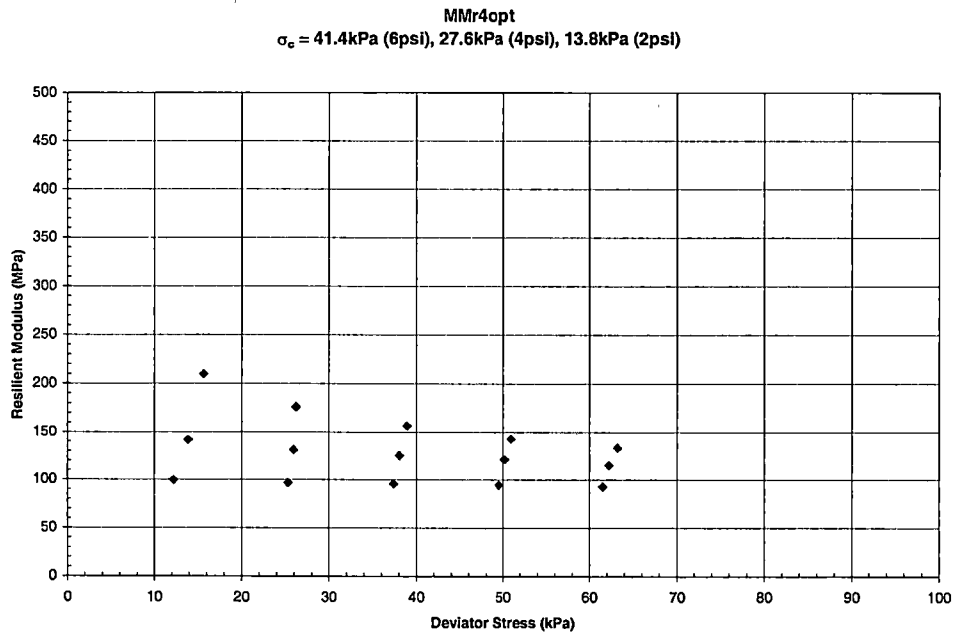
Graph B - 20 Resilient Modulus vs. Deviator Stress for McNairy County – MMr4opt
