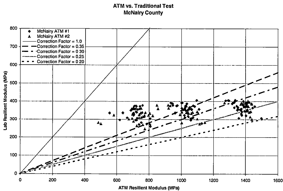
Figure 4-13 ATM Versus Traditional Test for McNairy County
