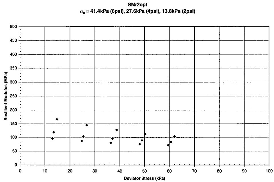
Graph B - 41 Resilient Modulus vs. Deviator Stress for Sumner County – SMr2opt
