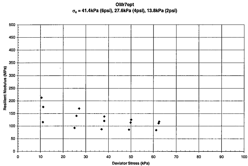
Graph B - 34 Resilient Modulus vs. Deviator Stress for Overton County – OMr7opt
