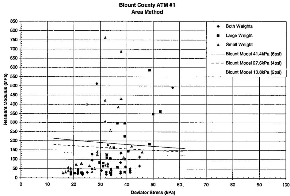
Figure 4-5 Typical ATM Result for Area Method
