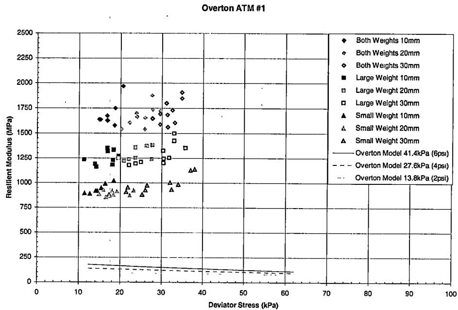
Graph C - 5 Resilient Modulus vs. Deviator Stress for Overton County Overton ATM #1 – Peak Acceleration
