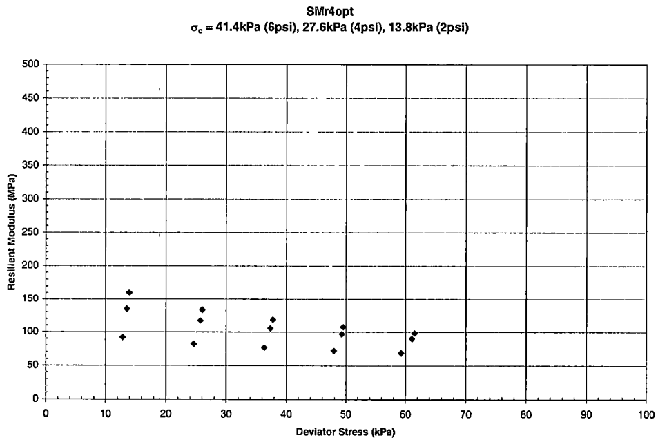
Graph B - 43 Resilient Modulus vs. Deviator Stress for Sumner County – SMr4opt
