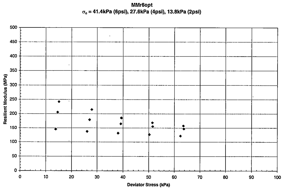
Graph B - 22 Resilient Modulus vs. Deviator Stress for McNairy County – MMr6opt
