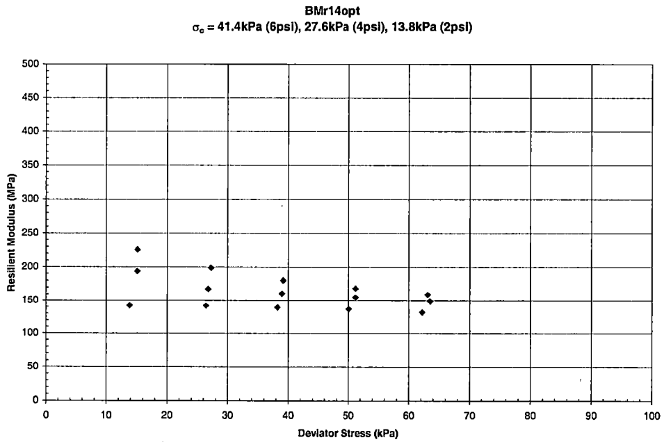
Graph B - 12 Resilient Modulus vs. Deviator Stress for Blount County - BMr14opt
