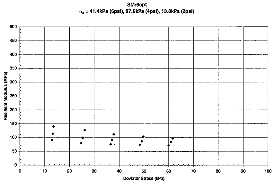
Graph B - 45 Resilient Modulus vs. Deviator Stress for Sumner County – SMr6opt
