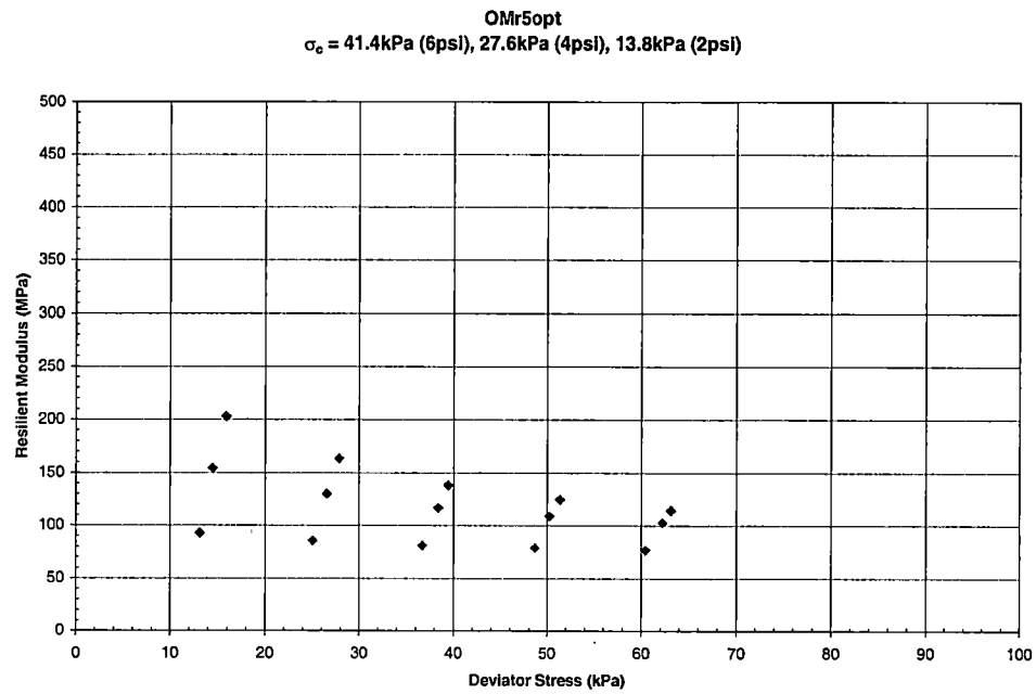
Graph B - 32 Resilient Modulus vs. Deviator Stress for Overton County – OMr5opt
