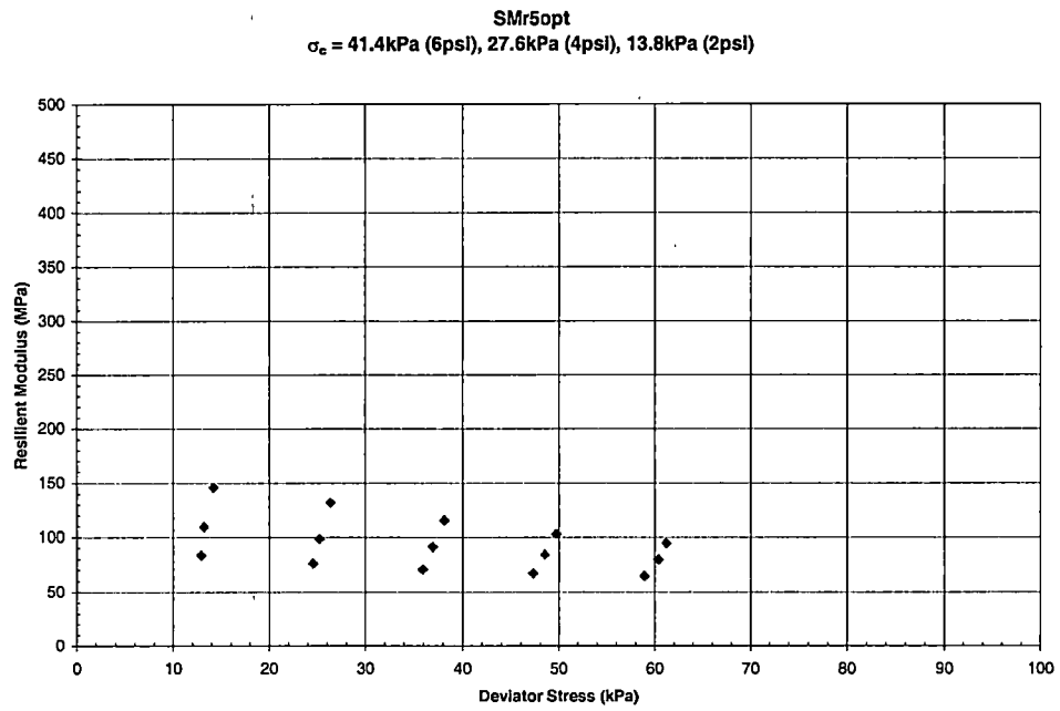
Graph B - 44 Resilient Modulus vs. Deviator Stress for Sumner County – SMr5opt
