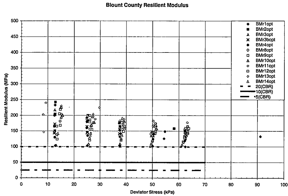
Figure 3-3 CBR Correlation with Blount County
