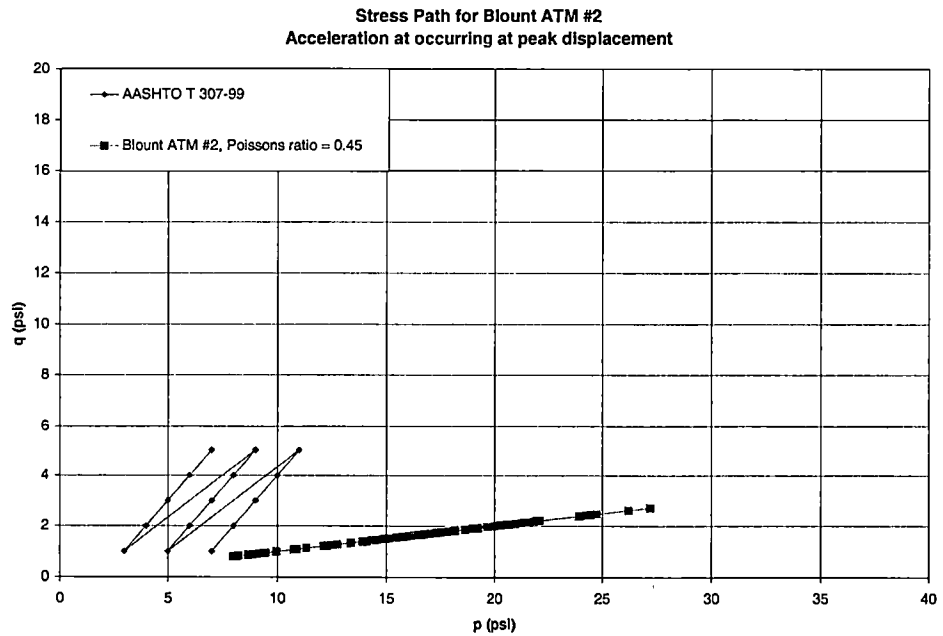
Graph C – 18 Stress Path for Blount ATM #2
