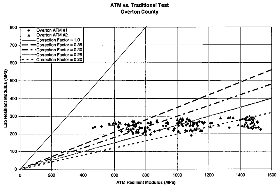
Figure 4-14 ATM Versus Traditional Test for Overton County
