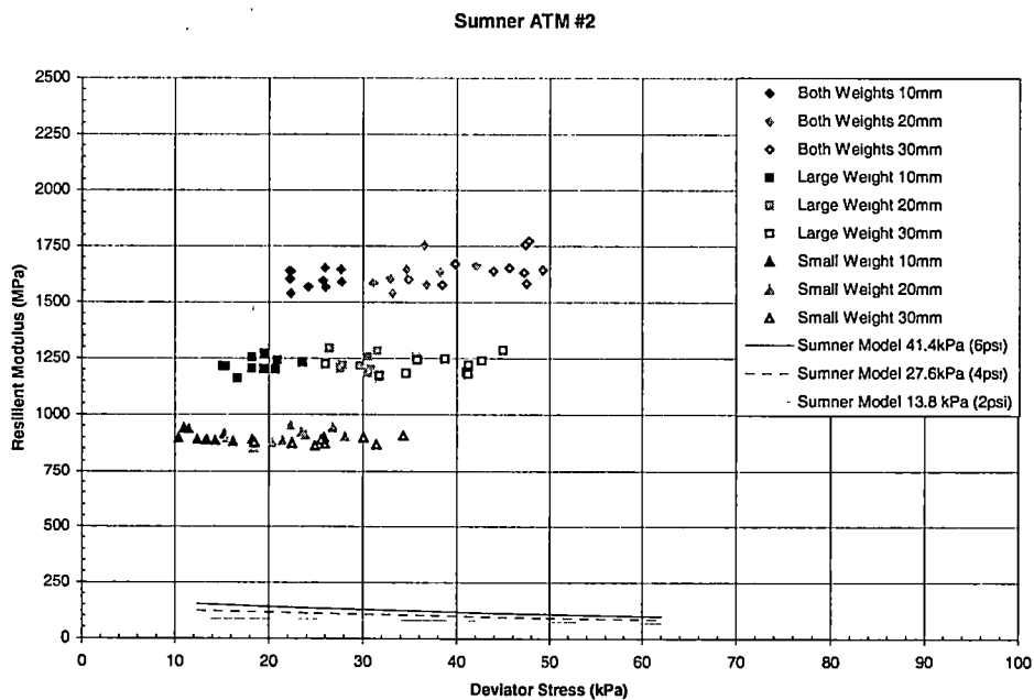
Graph C - 8 Resilient Modulus vs. Deviator Stress for Sumner County Sumner ATM #2 – Peak Acceleration
