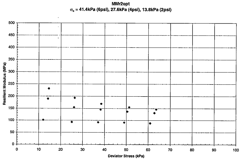
Graph B - 18 Resilient Modulus vs. Deviator Stress for McNairy County - MMr2opt
