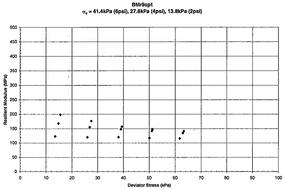
Graph B - 7 Resilient Modulus vs. Deviator Stress for Blount County – BMr9opt
