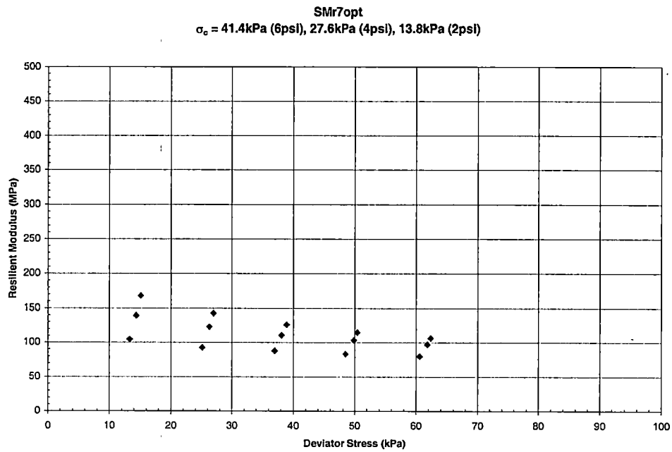
Graph B - 46 Resilient Modulus vs. Deviator Stress for Sumner County – SMr7opt
