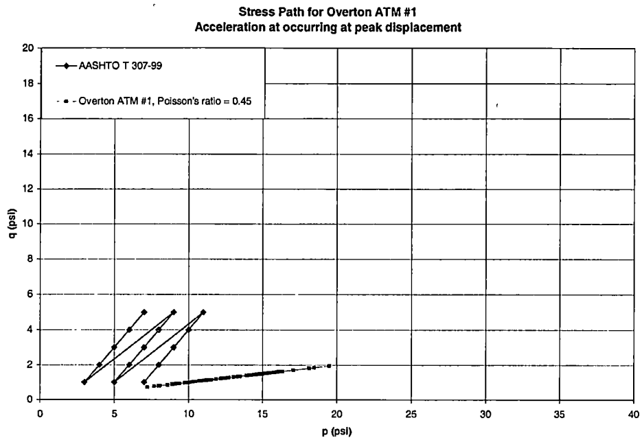
Graph C – 21 Stress Path for Overton ATM #1
