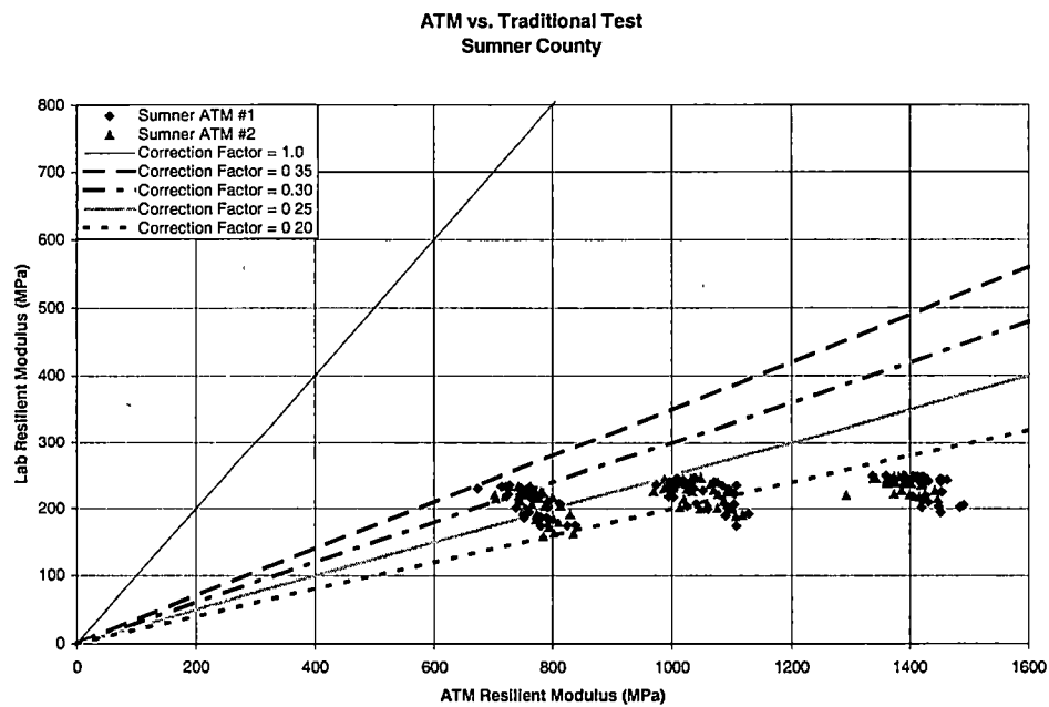
Figure 4-15 ATM Versus Traditional Test for Sumner County
