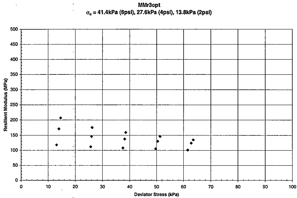
Graph B - 19 Resilient Modulus vs. Deviator Stress for McNairy County – MMr3opt
