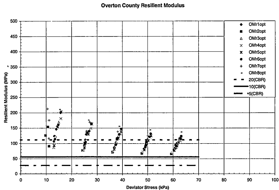
Figure 3-5 CBR Correlation with Overton County
