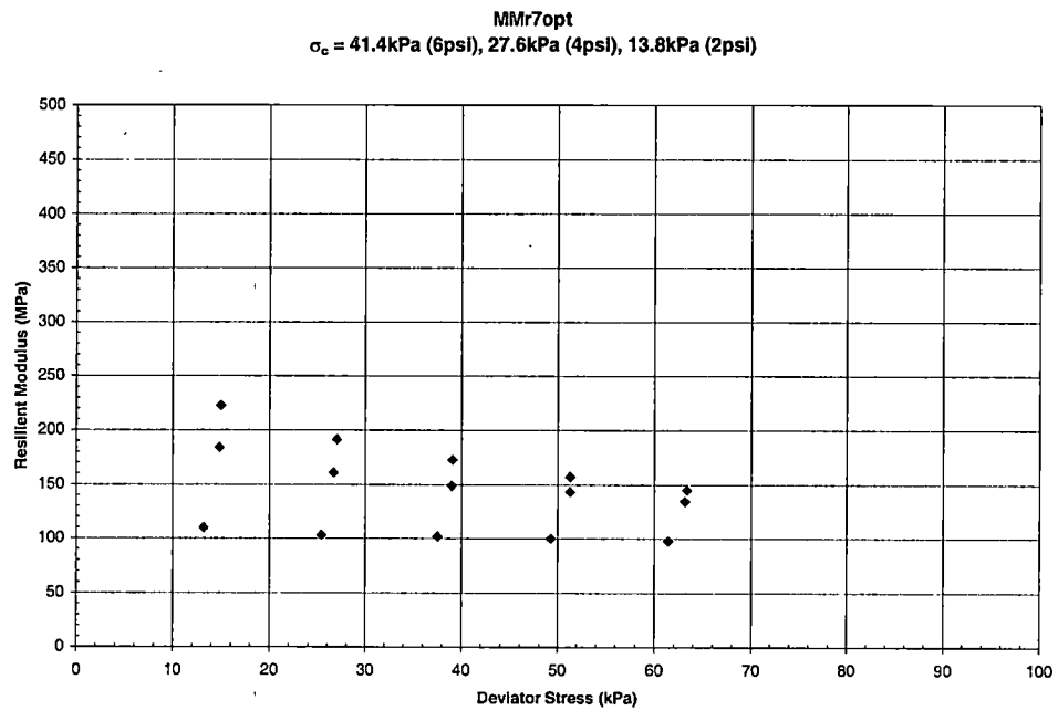
Graph B - 23 Resilient Modulus vs. Deviator Stress for McNairy County – MMr7opt
