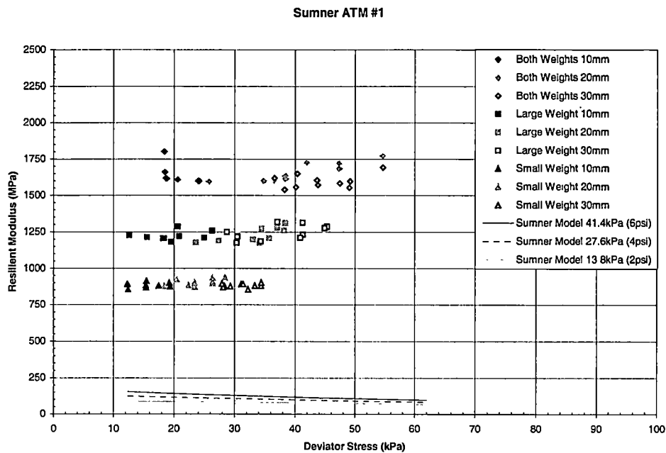
Graph C - 7 Resilient Modulus vs. Deviator Stress for Sumner County – Sumner ATM #1 – Peak Acceleration
