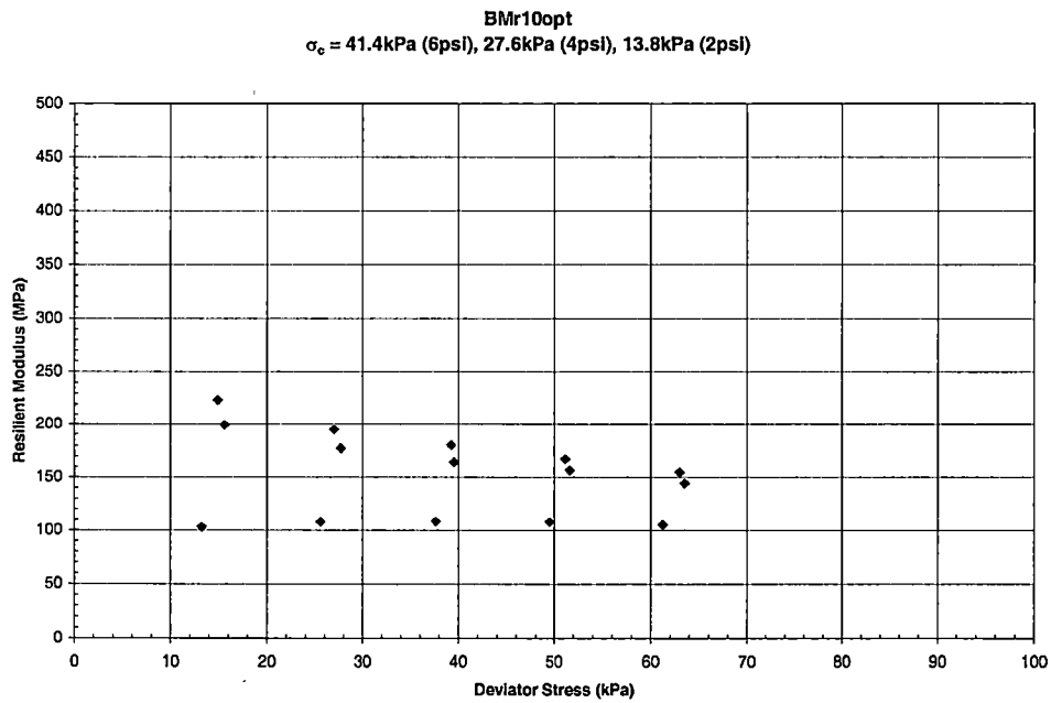
Graph B - 8 Resilient Modulus vs. Deviator Stress for Blount County - BMr10opt
