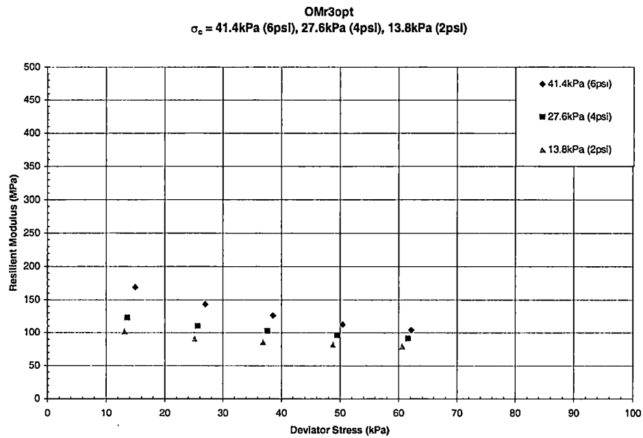
Figure 2-5 Typical Repeated Load Triaxial Test Results
