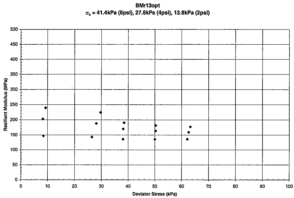
Graph B - 11 Resilient Modulus vs. Deviator Stress for Blount County - BMr13opt
