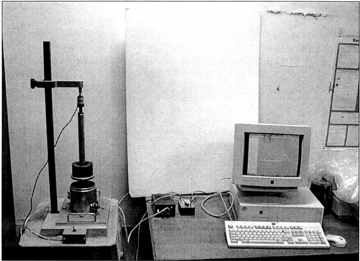
Figure 4-1 ATM Setup
