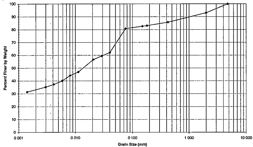
Grain Size Distribution Sumner County
