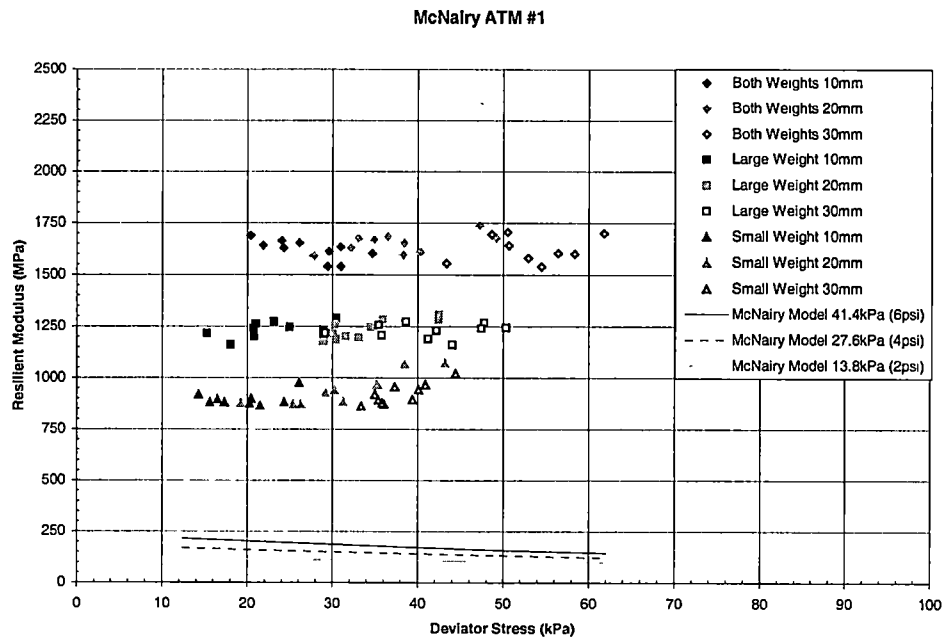
Graph C - 3 Resilient Modulus vs. Deviator Stress for McNairy County McNairy ATM #1 – Peak Acceleration
