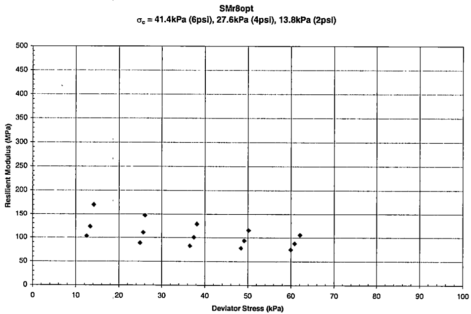
Graph B - 47 Resilient Modulus vs. Deviator Stress for Sumner County – SMr8opt
