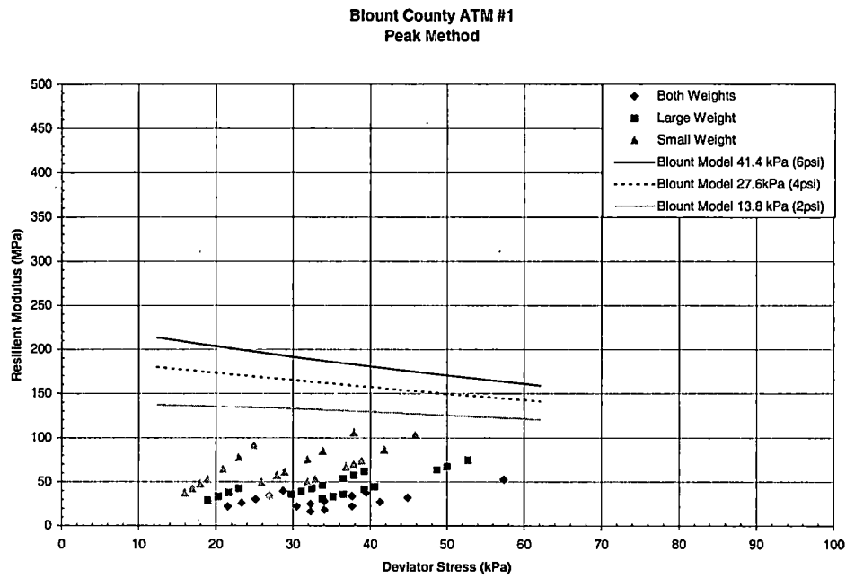
Figure 4-4 Typical ATM Result for Peak Method
