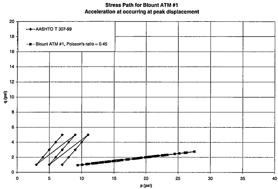
Graph C – 17 Stress Path for Blount ATM #1
