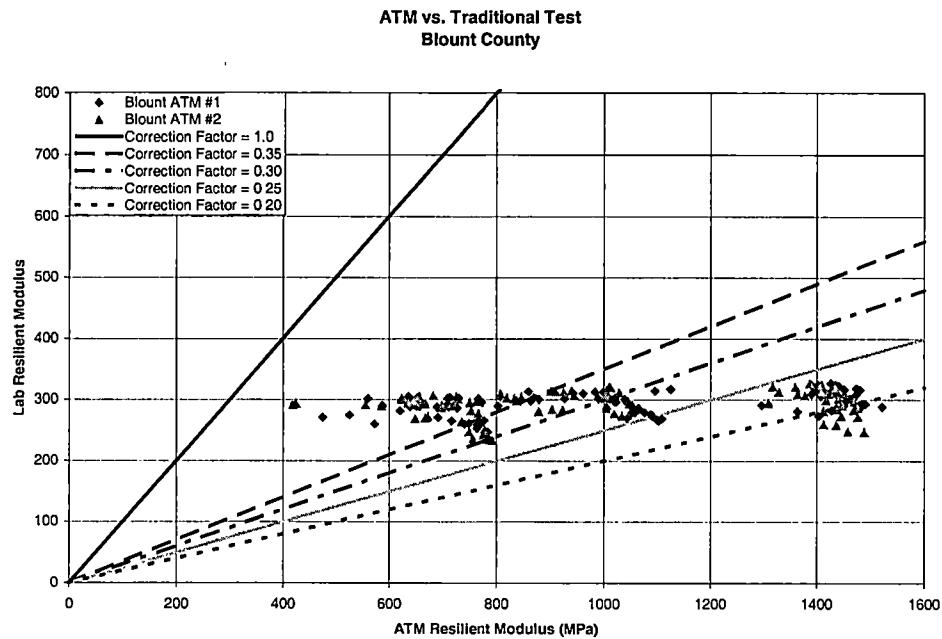
Figure 4-12 ATM Versus Traditional Test for Blount County
