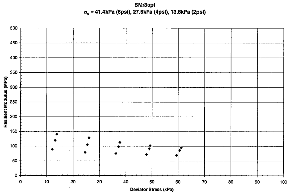
Graph B - 42 Resilient Modulus vs. Deviator Stress for Sumner County – SMr3opt
