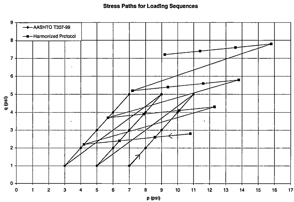
Figure 2-10 Stress Path for Loading Sequences (adopted from Andrei 1999)
