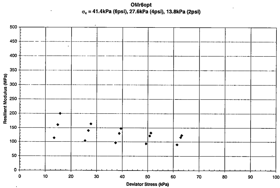
Graph B - 33 Resilient Modulus vs. Deviator Stress for Overton County – OMr6opt
