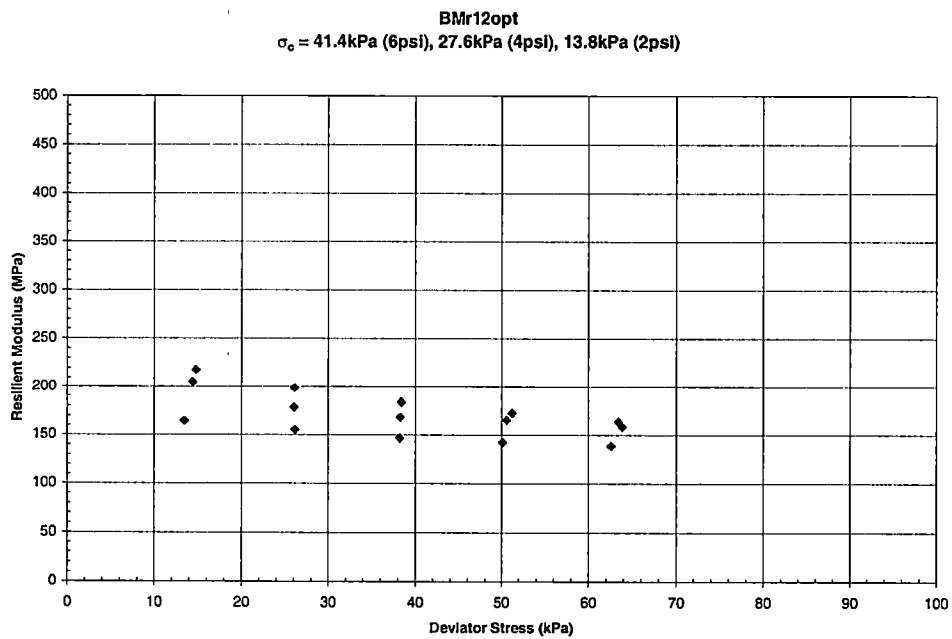
Graph B - 10 Resilient Modulus vs. Deviator Stress for Blount County - BMr12opt
