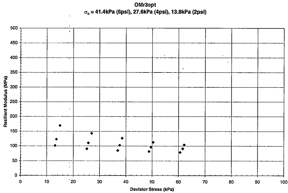
Graph B - 30 Resilient Modulus vs. Deviator Stress for Overton County – OMr3opt
