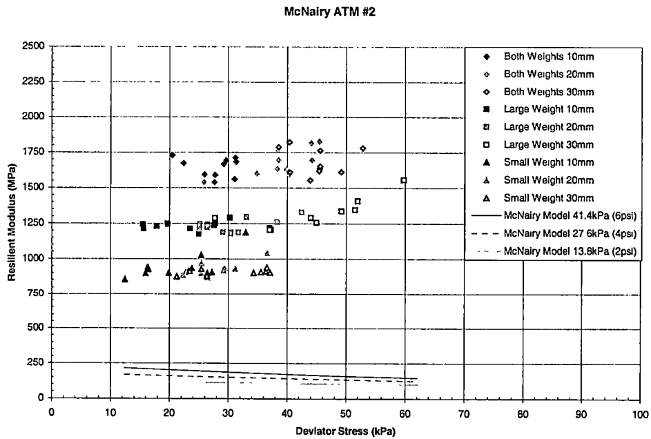
Graph C - 4 Resilient Modulus vs. Deviator Stress for McNairy County McNairy ATM#2 – Peak Acceleration
