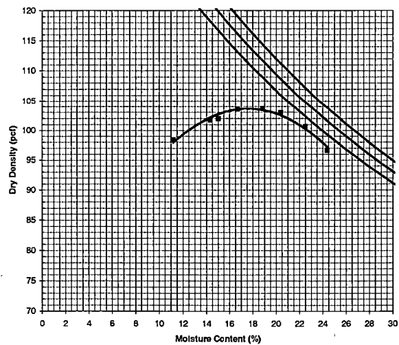
Sumner County Moisture vs. Density
