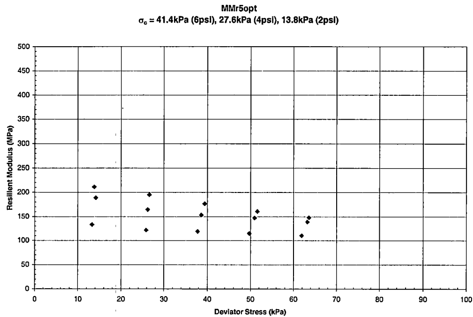
Graph B - 21 Resilient Modulus vs. Deviator Stress for McNairy County – MMr5opt
