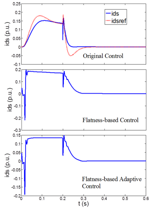
Figure 4.17 Results of I_d with change of transmission network and load.
