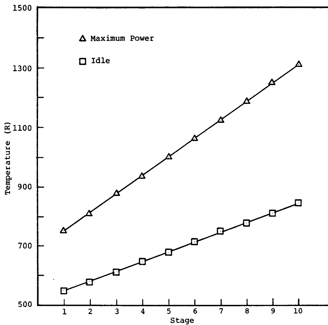
Figure 7. Total Temperature Rise Through HP Compressor.
