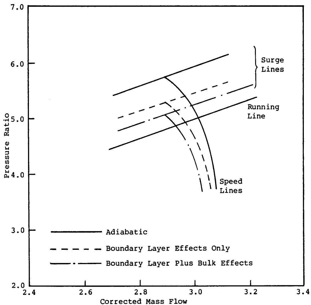
Figure 4. Combined Effects of Heat Transfer on HP Compressor During Deceleration [7].
