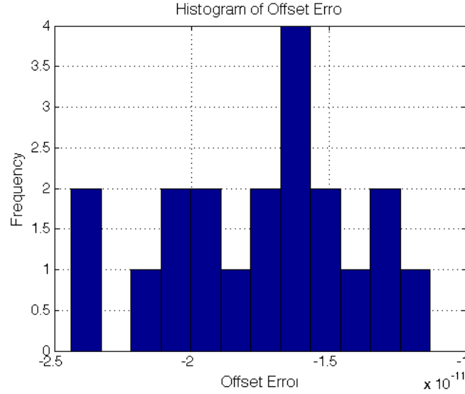
Figure 4.13: DAC Percent Offset Error is 17 \text{ pA} \pm 1.5 \text{ pA} with a confidence of 95%
