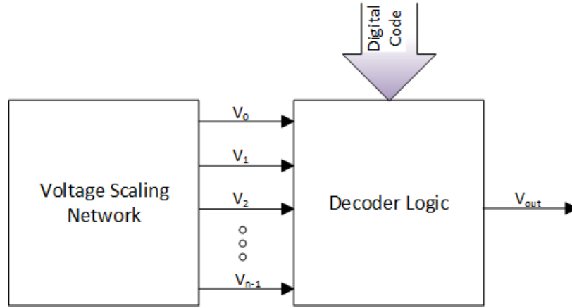
Figure 2.6: Basic Voltage Scaling DAC
