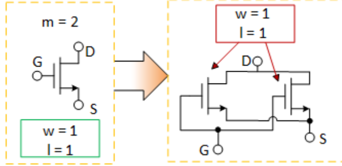
Figure 4.1: Transistor multiplicity
