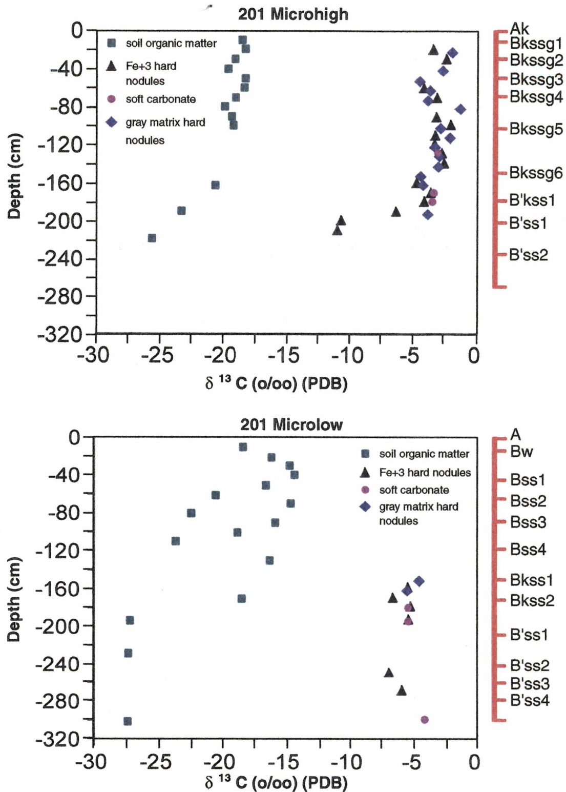
Figure 11. Plot of \delta^{13}\text{C} versus depth for both SOM and pedogenic carbonate for microhigh and microlow profiles of Harris Co. (201), showing climate/ecosystem changes with horization.
