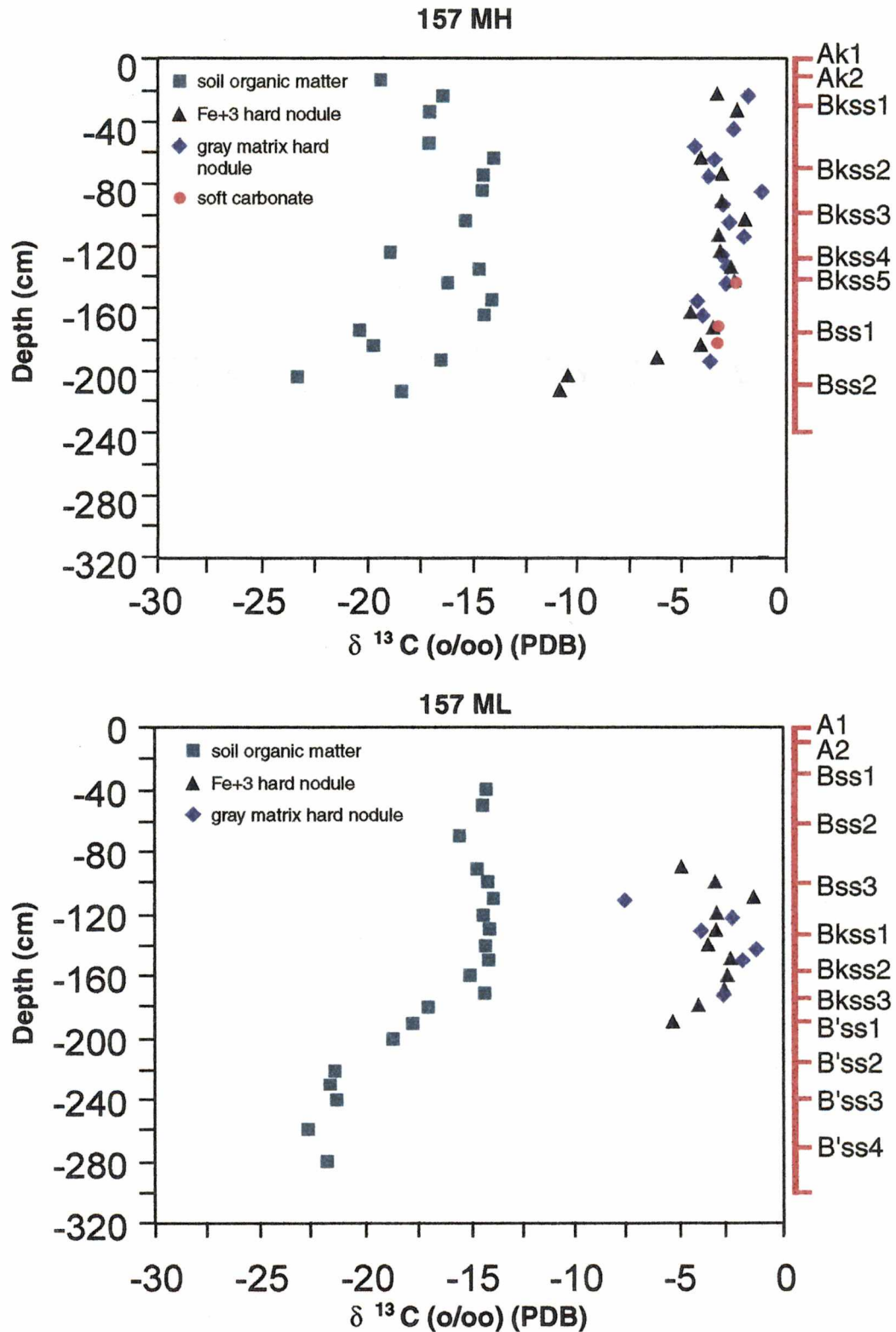
Figure 12. Plots for \delta^{13}\text{C} for both SOM and pedogenic carbonate for microhigh and microlow pedons at Fort Bend Co. (157), showing climate/ecosystem trends with soil horization.
