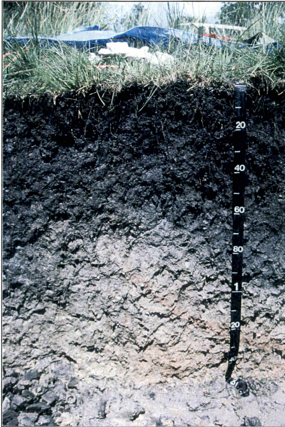
Figure 3. Field shot of Lake Charles microhigh pedon from Harris Co. (Armond Bayou), Texas shows a depth of ~ 1.5m. Slickenside faces are observed concentrating more toward the bottom of the profile and along the edges of the microhigh.
