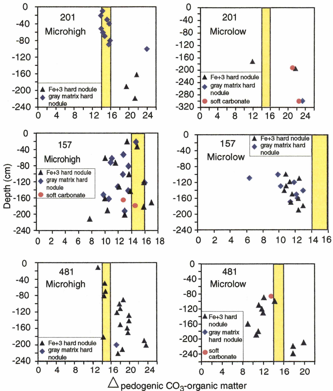
Figure 16. \Delta pedogenic \text{CO}_3 -organic matter show that the majority of values do not fall within the 14-16 o/oo expected if soil carbonate precipitated in equilibrium with SOM found at the same depth in the profile. The lack of correlation suggests that the solution precipitating carbonate derived a portion of its carbon from elsewhere in the soil profile. This discrepancy suggests that soil organic matter and soil carbonate at the same depth are not contemporaneous.
