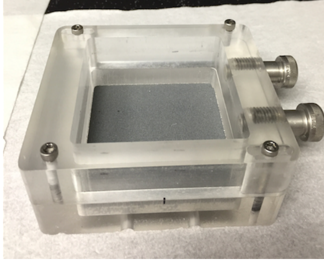
Figure 3.2. Photo of the Direct Shear Box
