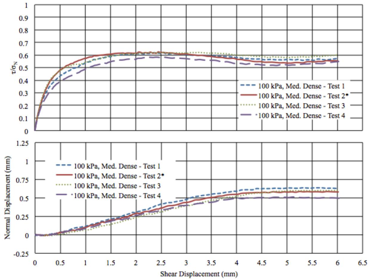
Normalized Shear Stress and Normal Displacement versus Shear Displacement for #1 Dry Glass Sand, 100 kPa, Medium-Dense Specimens
