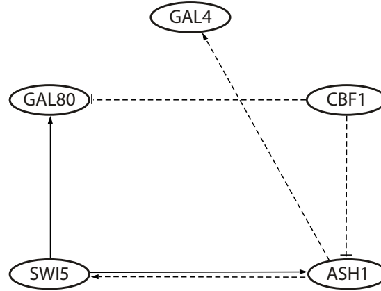
Figure 8.4: Inferred network by BANJO using switch-on data [15]
