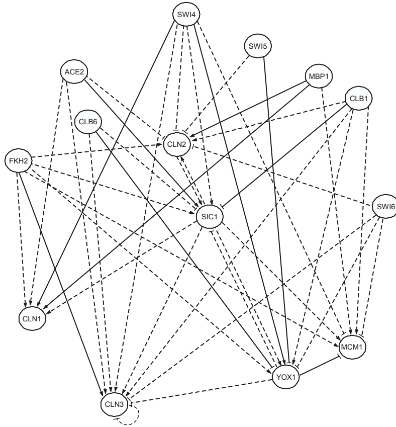
Figure 4.5: Inferred yeast cell cycle network. Solid and dashed lines indicate the correctly inferred and incorrectly inferred edges by CMSM1, respectively. PPV^u=0.42 , Se^u=0.47 , PPV^d=0.37 , Se^d=0.39 , PPV^s=0.21 , Se^s=0.22 .
