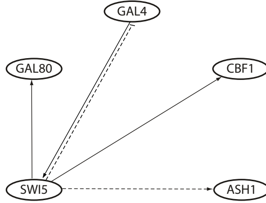
Figure 8.3: Inferred network by TSNI using switch-on data [15]
