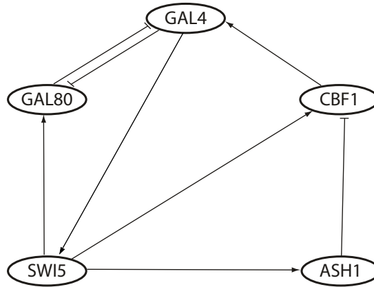
Figure 3.4: Five-gene yeast true network [15]
