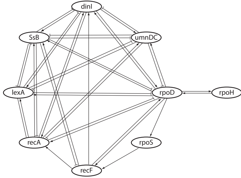
Figure 3.7: Nine-gene true E. coli network [4].
