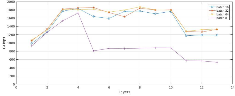
Figure 2.2: SGEMM performance.
