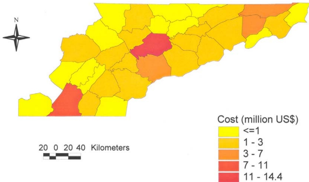
Figure 4-44: Total cost (WTP) distribution in East Tennessee for COPD admissions due to maximum 8-hr ozone exposure for the scenario control of NO x (mobile source 50% and point source 70%).
