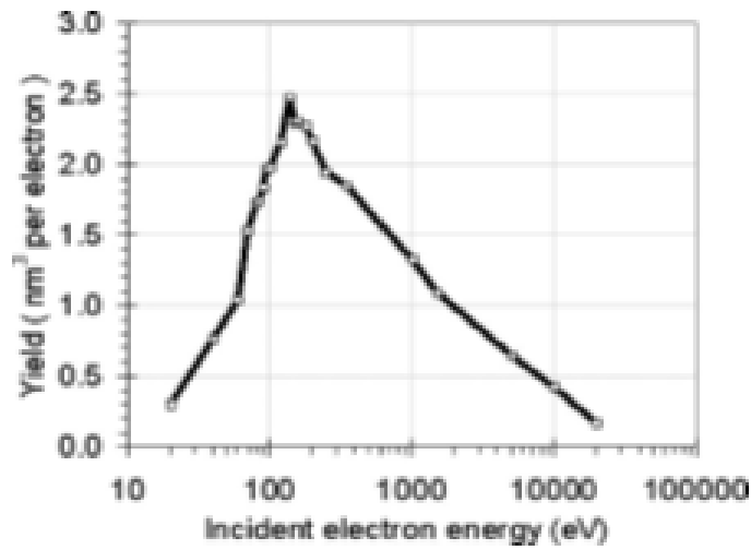
Figure 1.3. Deposition yield as a function of beam energy for the \text{MeCpPt(IV)Me}_3 molecule [6].
