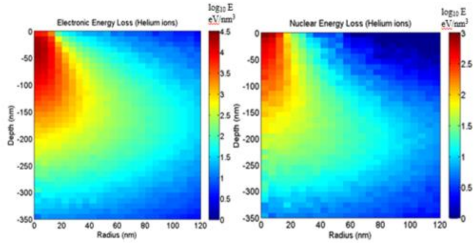
Figure 2.13. Simulated electronic and the nuclear volumetric energy losses for helium ions at 30 keV at a dose of 1 \times 10^{17} ions/cm 2 .
