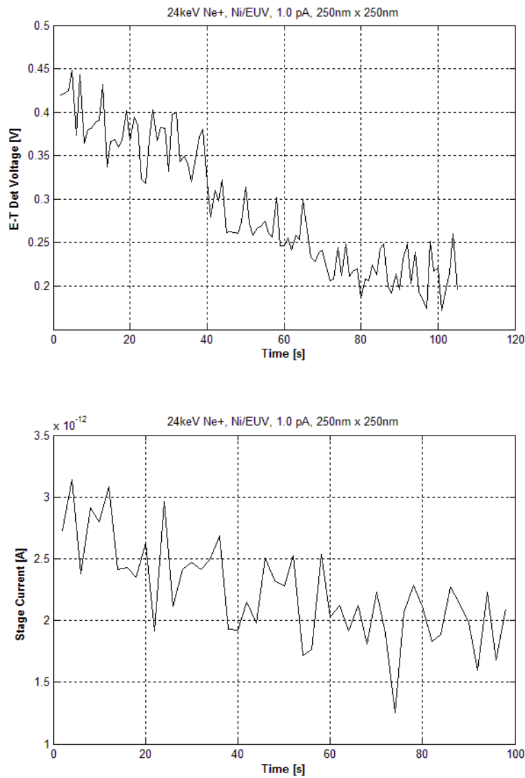
Figure 3.3. E-T detector voltage and the stage current for the electronic profiling of the EUV mask.
