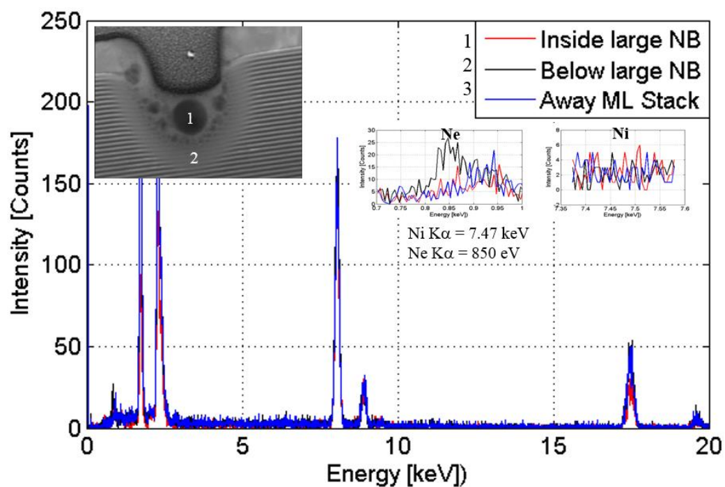
Figure 2.20. High magnification viewgraph while performing EDXS in the TEM around a large neon nanobubble located near the etch zone and directly under the beam trajectory for a dose of 0.7 nC/ \mu\text{m}^2 .
