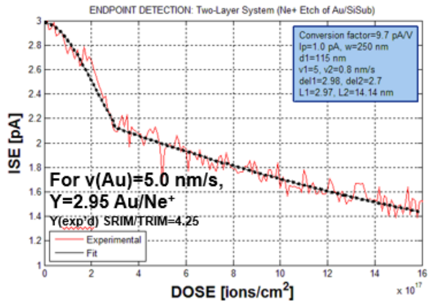
Figure 3.27. Experimental and fit ISE vs. Dose data for \text{Ne}^+ on Au/Si.
