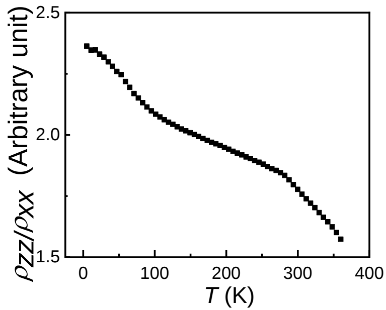
Figure 3.20: Temperature dependent \rho_{zz}/\rho_{xx}
