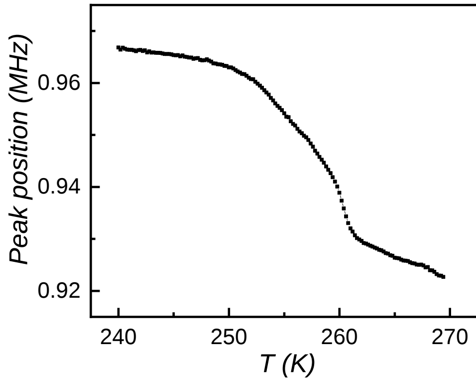
Figure 3.18: One ultrasound resonance position changes with temperature change
