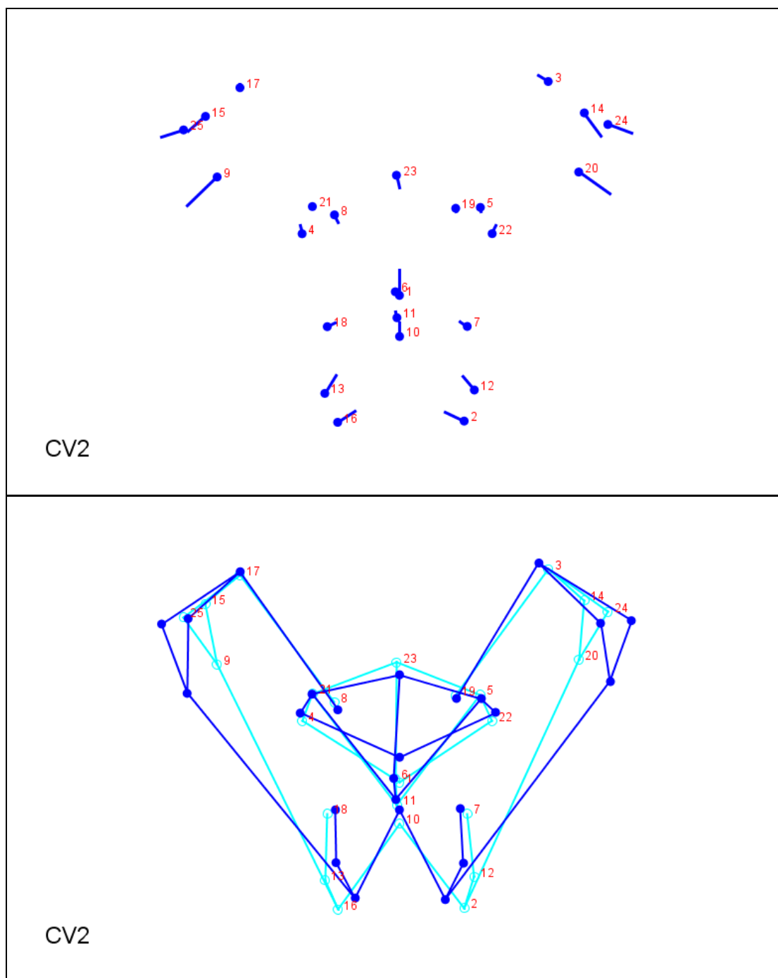
Figure 20: Landmark shifts along second canonical variate in black males. The light blue wireframe represents the starting form while the dark blue wireframe represents change over canonical variate two. Landmark identifications of the numbered points can be found in Table A13 in the appendix.
