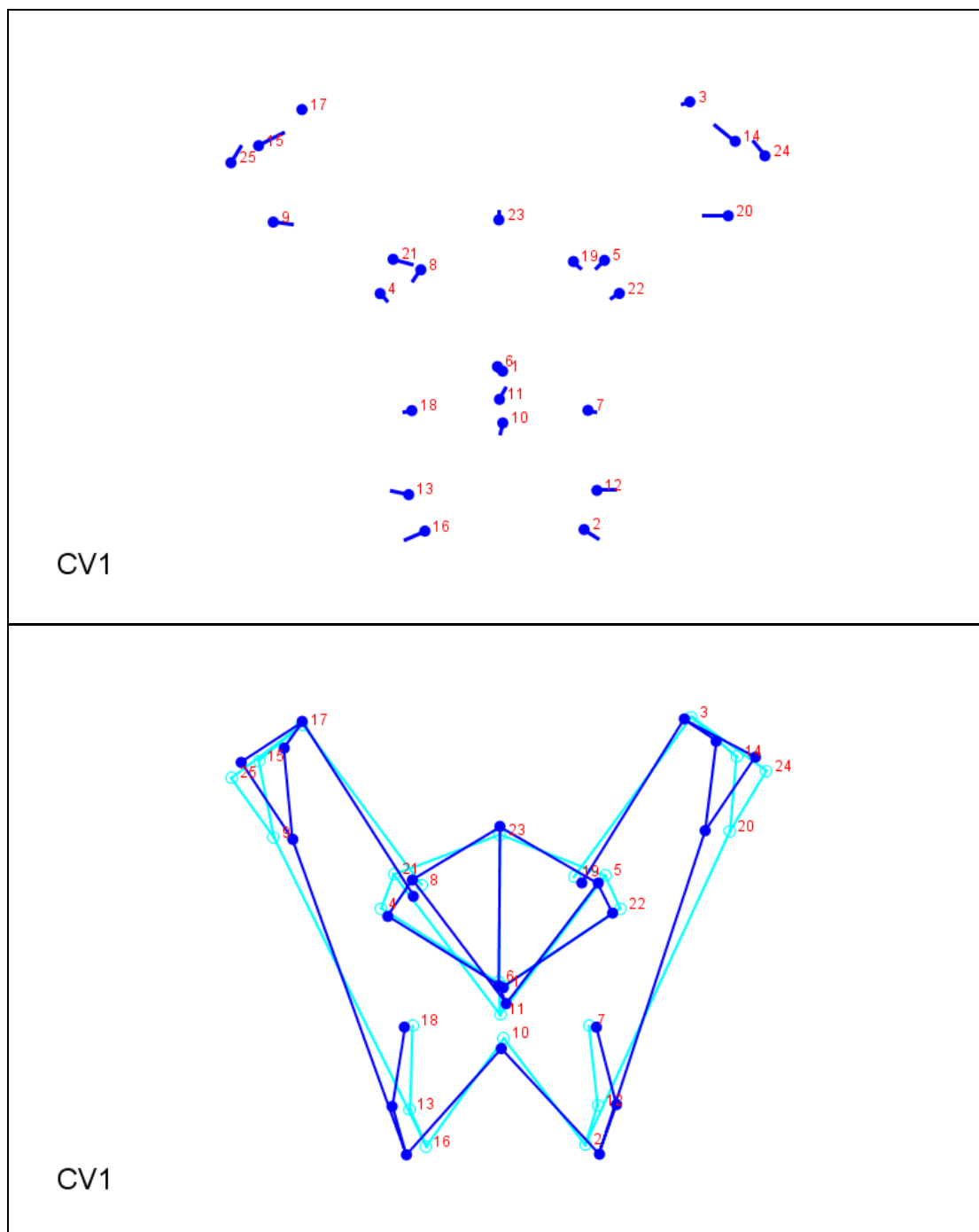
Figure 19: Landmark shifts along first canonical variate in black males. The light blue wireframe represents the starting form while the dark blue wireframe represents change over canonical variate one (later cohorts). Landmark identifications of the numbered points can be found in Table A13 in the appendix.
