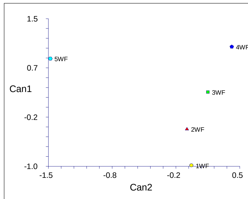
Figure 13b: Canonical plot of cohort means of white females
