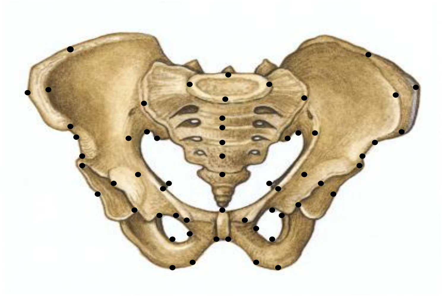
Figure 4a: Illustration of landmarks
