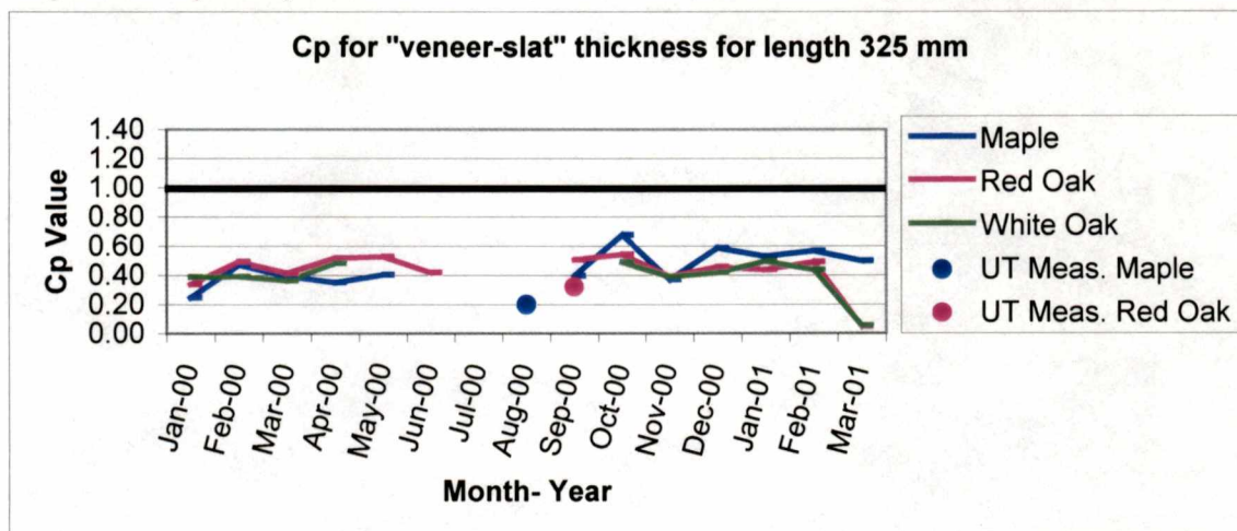
Graph 9c. Capability indices for "veneer-slat" thickness for target length 325 mm.
