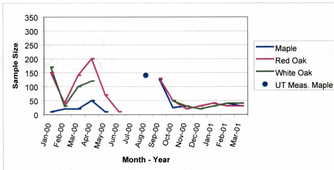
Graph 20a. Sample size for “veneer-slat” thickness for target length 215 mm.
