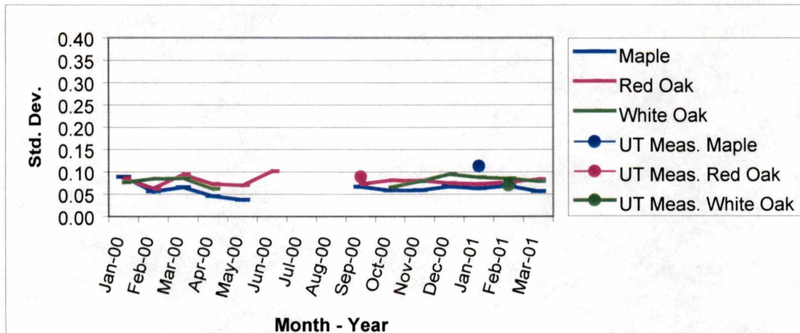
Figure 17. Standard deviation (mm) for "veneers-slat" thickness for target length 270 mm.
