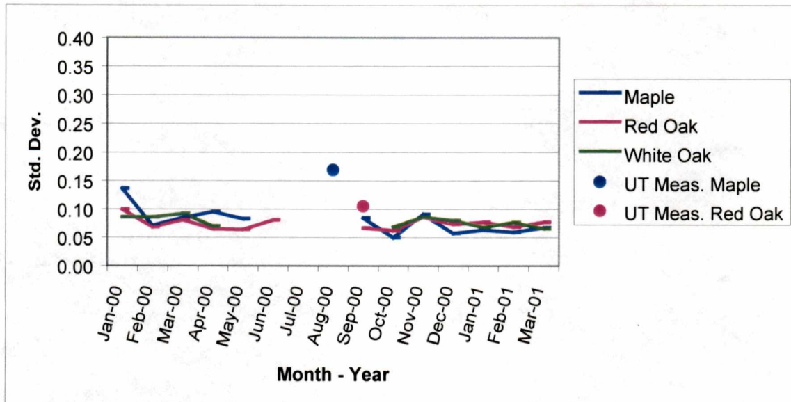
Graph 23a. Standard deviations (mm) for “veneers-slat” thickness for target length 325 mm.
