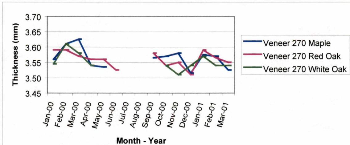
Figure 18. Medians for "veneer-slat" thickness for target length 270 mm.
