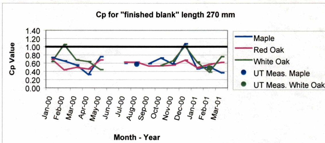
Graph 2c. Capability indices for "finished blank" length for target length 270 mm.
