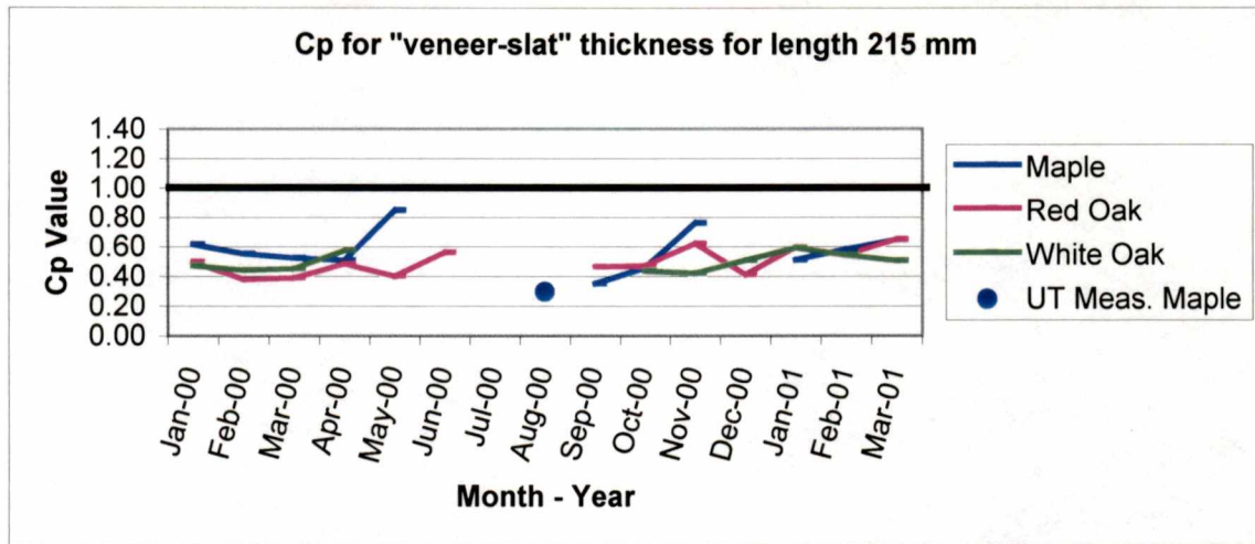
Graph 7c. Capability indices for "veneer-slat" thickness for target length 215 mm.
