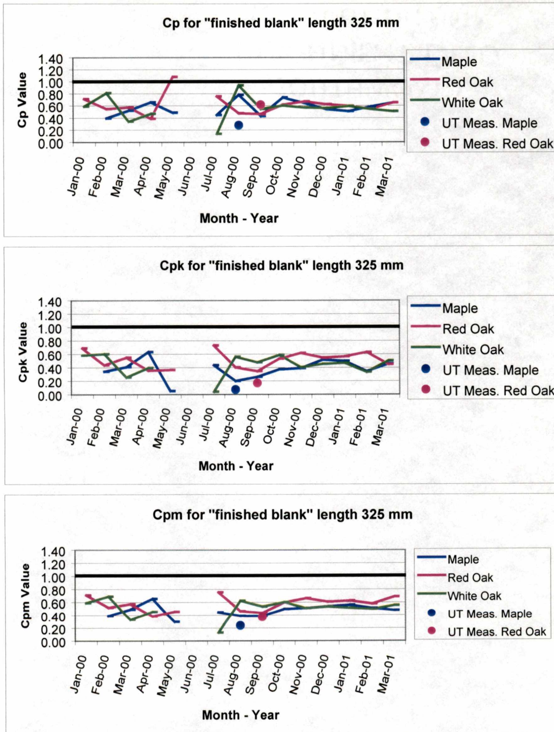
Graph 3c. Capability indices for "finished blank" length for target length 325 mm.
