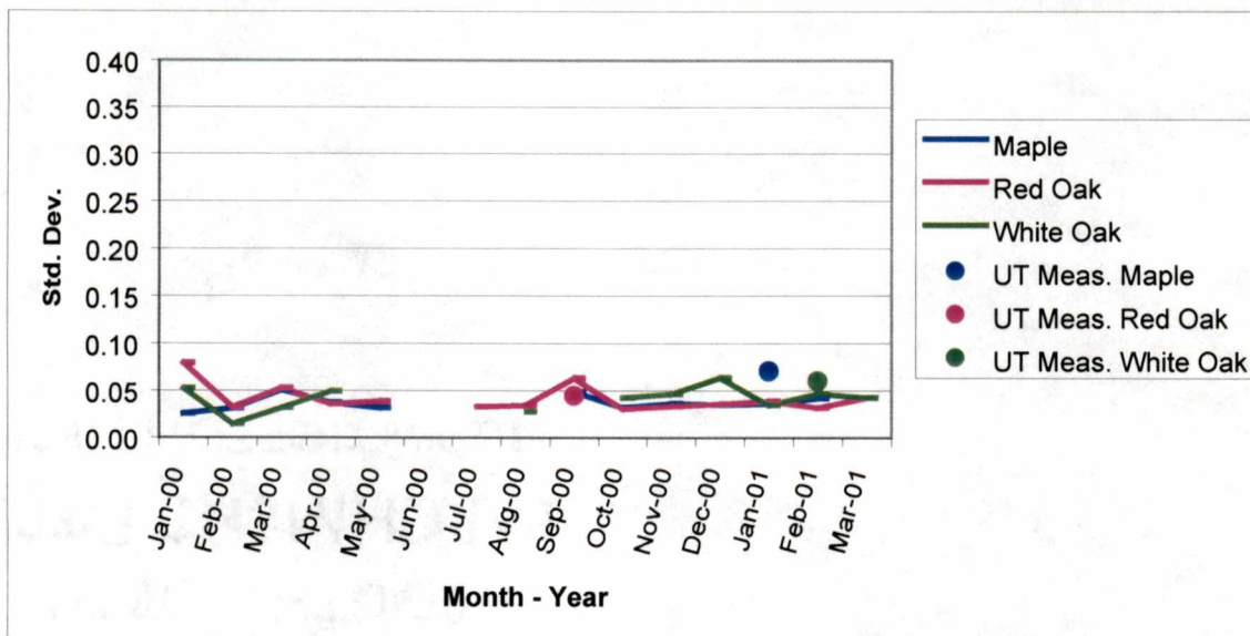
Graph 15a. Standard deviations (mm) for “finished blank” width for target length 270 mm.
