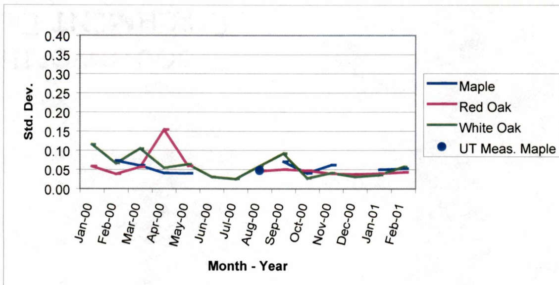
Graph 7a. Standard deviations (mm) for “finished blank” length for target length 215 mm.
