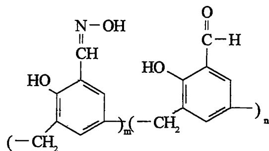
Figure 1.18. Poly(salicylaldoxime-3,5-diylmethylene)
