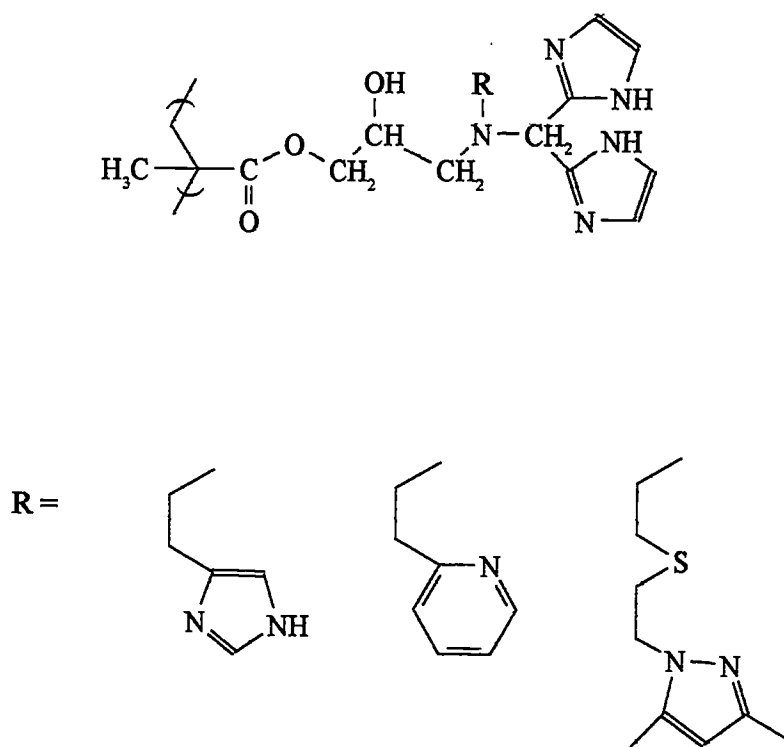
Figure 1.5. Polymer-supported bis(imidazole) ligands
