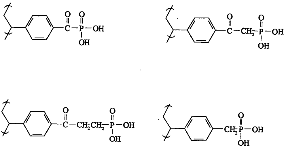
Figure 1.31. Immobilized ketophosphonic acid ligands:
