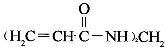
Figure 4.5. N,N'-methylene bisacrylamide
