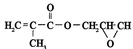
Figure 4.4. Glycidyl methacrylate
