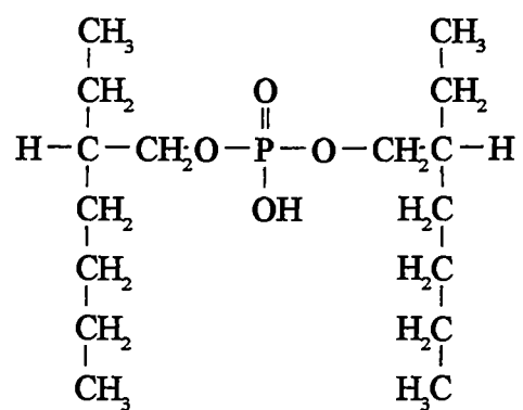
Figure 1.37. Bis(2-ethylhexyl)hydrogen phosphate
