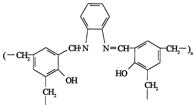
Figure 1.20. Polymeric o-phenylenediamine-salicylaldehyde-formaldehyde
