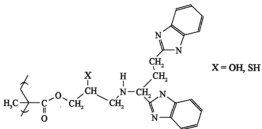
Figure 1.6. Polymer-supported bis(benzimidazole)
