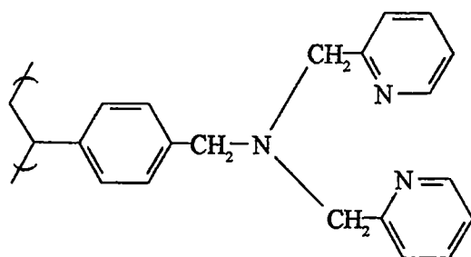
Figure 1.1. Polymer-supported bis-picolylamine
