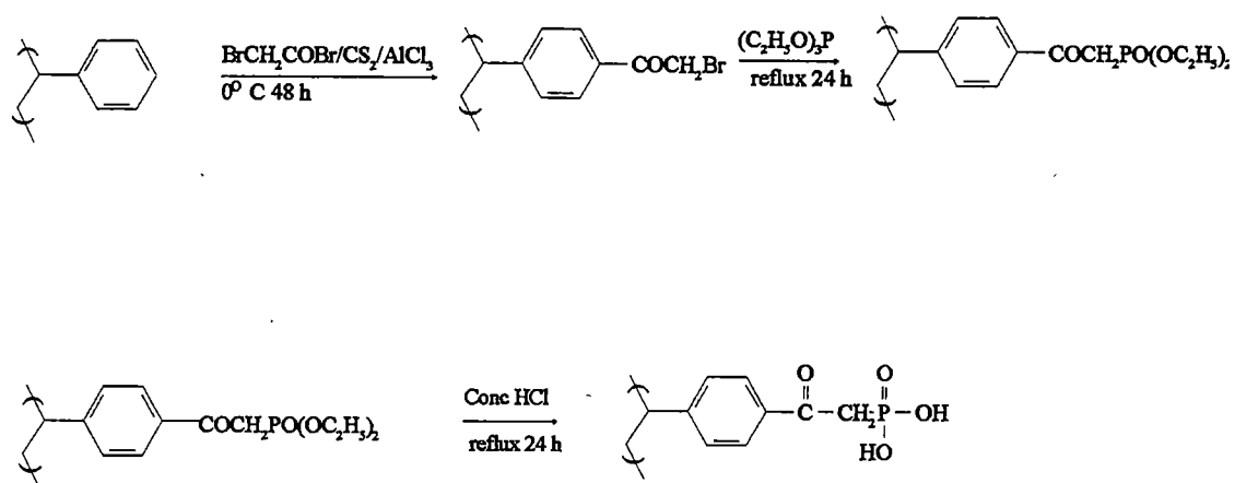
Figure 2.4. Synthesis of \beta -ketophosphonic acid foam
