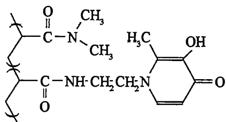
Figure 1.9. Copolymer of 1-( \beta -acrylamidoethyl)-3-hydroxy-2-methyl-4(1H)-pyridinone and N,N -dimethylacrylamide
