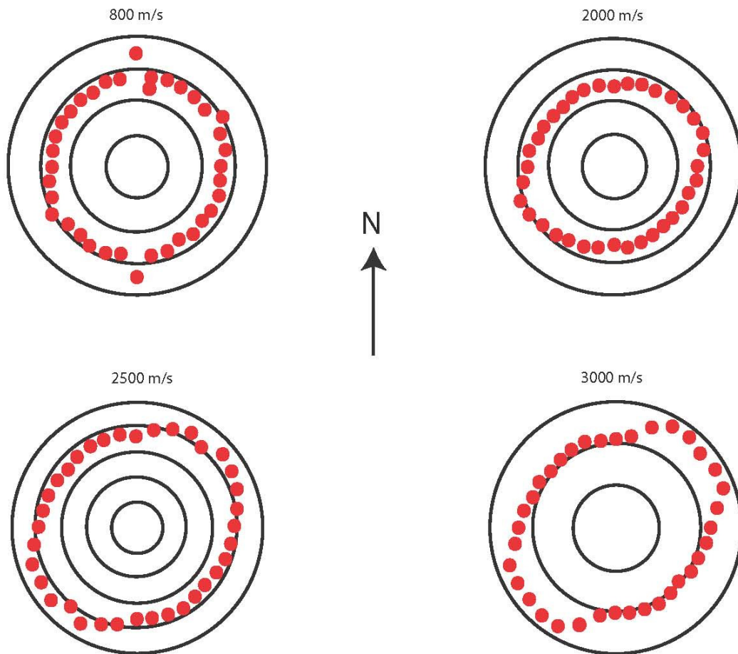
Figure 23: A series of depth slices indicating the magnitude and direction of seismic anisotropy for the NT-2 site. The depths are: 1 m in the top left, 3 m in the top right, 6 m in the bottom left, and 9 m in the bottom right.
