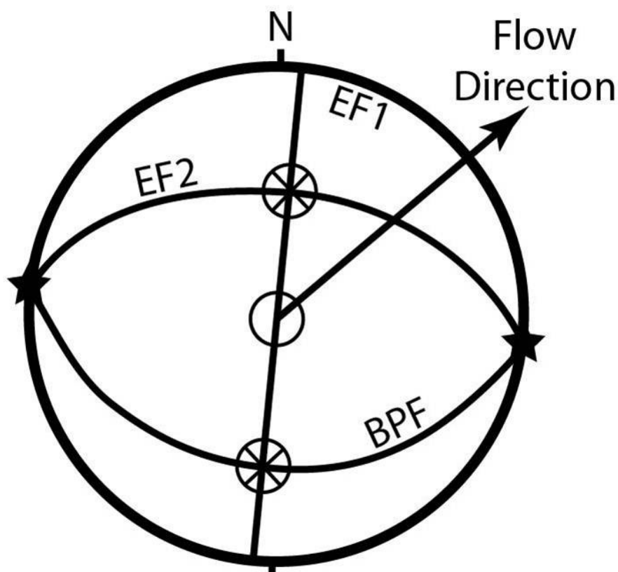
Figure 19: A stereographic image of the primary sets of orthogonal intersecting fractures. Extensonal fracture set intersections are marked with an X and a star marks where extensional fracture sets intersect with bedding plane fractures. The vector sum of the EF1-EF2 intersection and the east trending EF2-BPF intersection is approx.. N60E, while the observed preferred flow direction is N50E. Modified from Dreier, et al., 1988.
