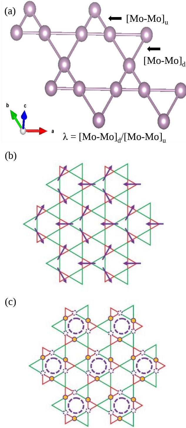
Figure 4.1: (a) The smaller up-triangles and larger down-triangles in the “breathing” Kagome lattice formed by the Mo atoms in the ab -plane. The Mo-Mo bond lengths as well as the breathing parameter \lambda are included. (b) Type-I cluster Mott insulator. (c) Type-II cluster Mott insulator.
