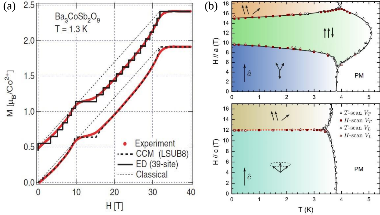
Figure 1.6: a) The magnetization curve corrected for Van Vleck paramagnetism. This figure was taken directly from Ref. 58. b) Magnetic phase diagram for \mu_0 H \parallel a and \mu_0 H \parallel c . This figure was taken from Ref. 62.
