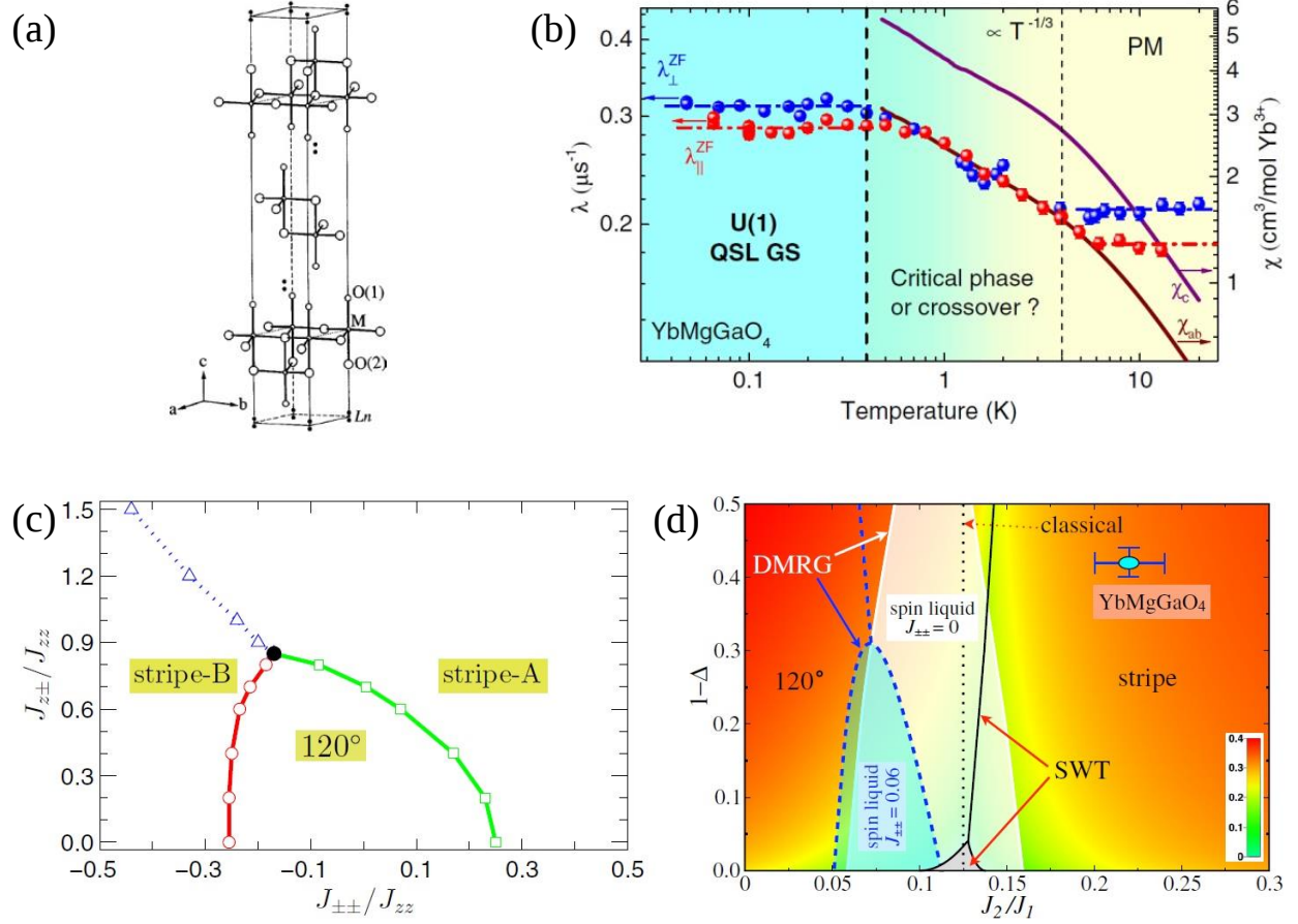
Figure 1.4: a) The crystal structure of the LnM^{2+}M'^{3+}O_4 family. This figure was taken directly from Ref. 18. b) A magnetic phase diagram constructed from \mu SR and bulk susceptibility measurements. This figure was taken directly from Ref. 23. c) A schematic quantum phase diagram constructed from the exact-diagonalization method of an XXZ model Hamiltonian. This figure was taken directly from Ref. 29. d) A phase diagram constructed from an XXZ model modified with pseudodipolar terms. This figure was taken directly from Ref. 30.
