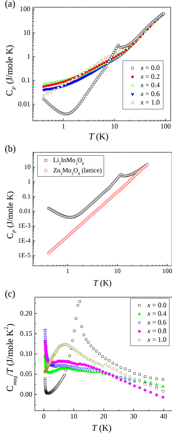
Figure 4.5: (a) The temperature dependence of the specific heat capacity measured at zero field. (b) The specific heat for the x = 0 sample as well as the for nonmagnetic \text{Zn}_2\text{Mo}_3\text{O}_8 which was used to subtract off the lattice contribution. (c) The magnetic specific heat divided by temperature measured at zero field.
