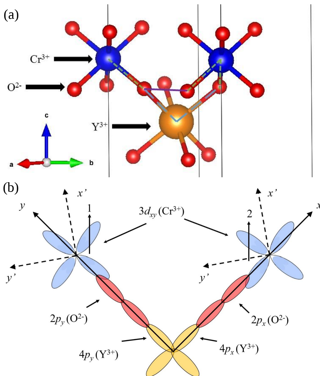
Figure 3.17: (a) The lattice view of the Cr 3+ -O 2- -O 2- -Cr 3+ and the Cr 3+ -O 2- -Y 3+ -O 2- -Cr 3+ superexchange paths; (b) the orbital configurations related to the Cr 3+ -O 2- -Y 3+ -O 2- -Cr 3+ superexchange path. The Cr 3+ ions' frame of reference is denoted with primes. The angle between the unprimed and primed axes is 55°. This figure can be found in Ref. 115.
