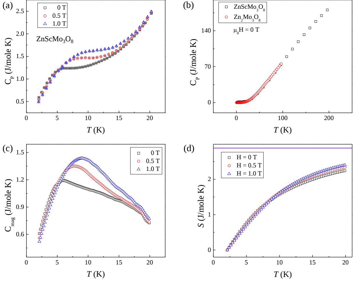
Figure 4.13: For \text{ZnScMo}_3\text{O}_8 , (a) the temperature dependence of the specific heat at various magnetic field strengths; (b) the temperature dependence at zero field of the specific heat of \text{ZnScMo}_3\text{O}_8 and the non-magnetic isostructural compound \text{Zn}_2\text{Mo}_3\text{O}_8 ; (c) the temperature dependence of the magnetic specific heat at various magnetic field strengths; (d) the temperature dependence of the total entropy of the system at various magnetic field strengths. The solid violet line lies at (R \ln 2)/2 .
