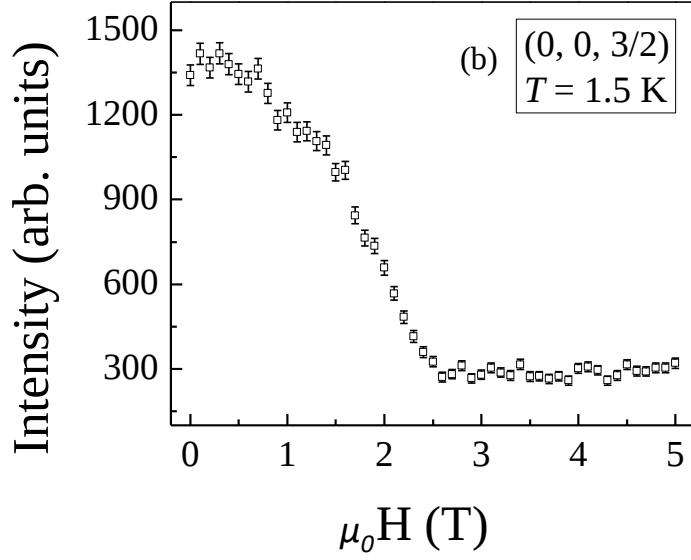
Figure 3.6: For \text{YCr}(\text{BO}_3)_2 , (a) the temperature dependence and (b) the field dependence of the (0,0,3/2) magnetic Bragg reflection, and the magnetic ground state at (c) \mu_0 H = 0 \text{ T} and (d) \mu_0 H = 5.0 \text{ T} . This figure can be found in Ref. 115.
