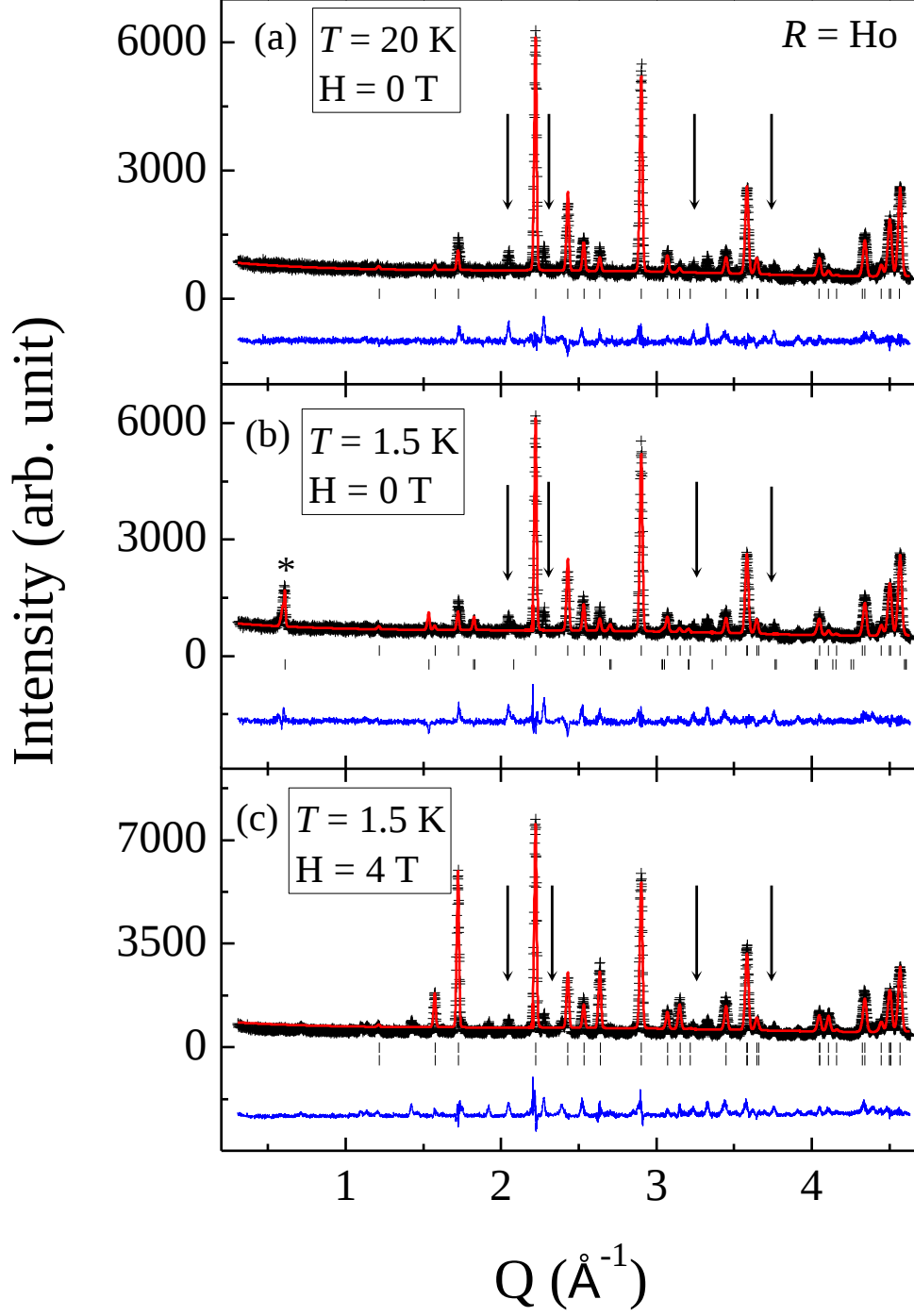
Figure 3.14: The neutron diffraction patterns for polycrystalline \text{HoCr}(\text{BO}_3)_2 (crosses) at (a) T = 20 \text{ K} and \mu_0 H = 0 \text{ T} , (b) T = 1.5 \text{ K} and \mu_0 H = 0 \text{ T} , and (c) T = 1.5 \text{ K} and \mu_0 H = 4.0 \text{ T} using a neutron wavelength of 2.413 \text{ \AA} . The solid curves are the best fits from the Rietveld refinements using FullProf Suite . The vertical marks indicate the position of Bragg reflections, and the bottom curves show the difference between the observed and calculated intensities. The * in (b) marks the location of the (0, 0, 3/2) reflection. The arrows denote \text{HoBO}_3 impurity peaks. This figure can be found in Ref. 115.
