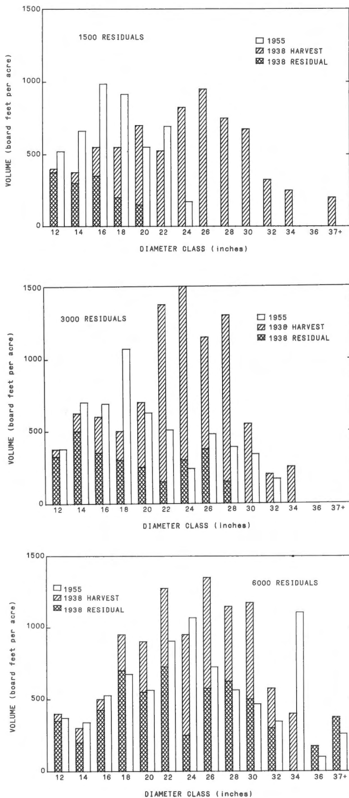
FIGURE 3. Stand structure by volume per acre for the first cutting cycle.
