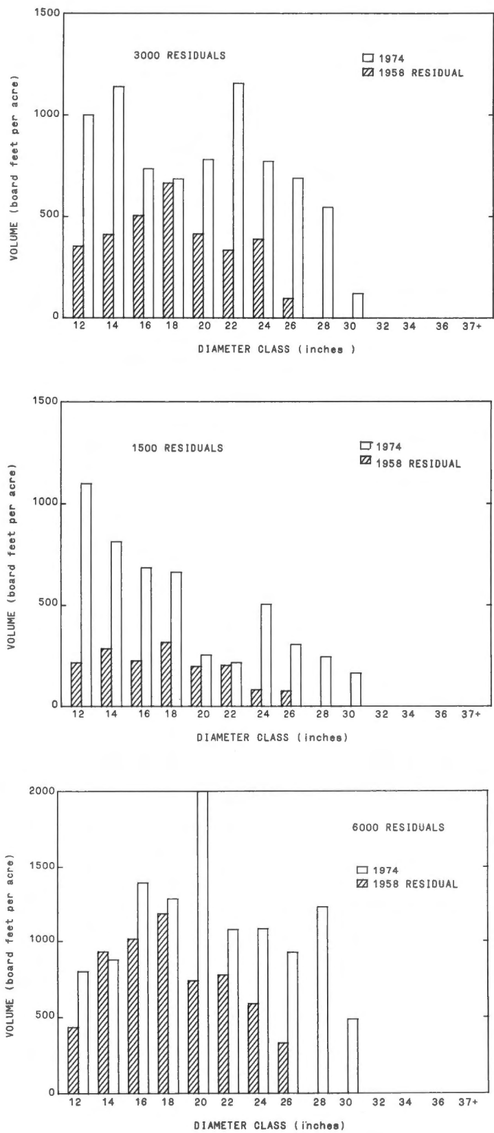
FIGURE 5. Stand structure by volume per acre for the second cutting cycle.
