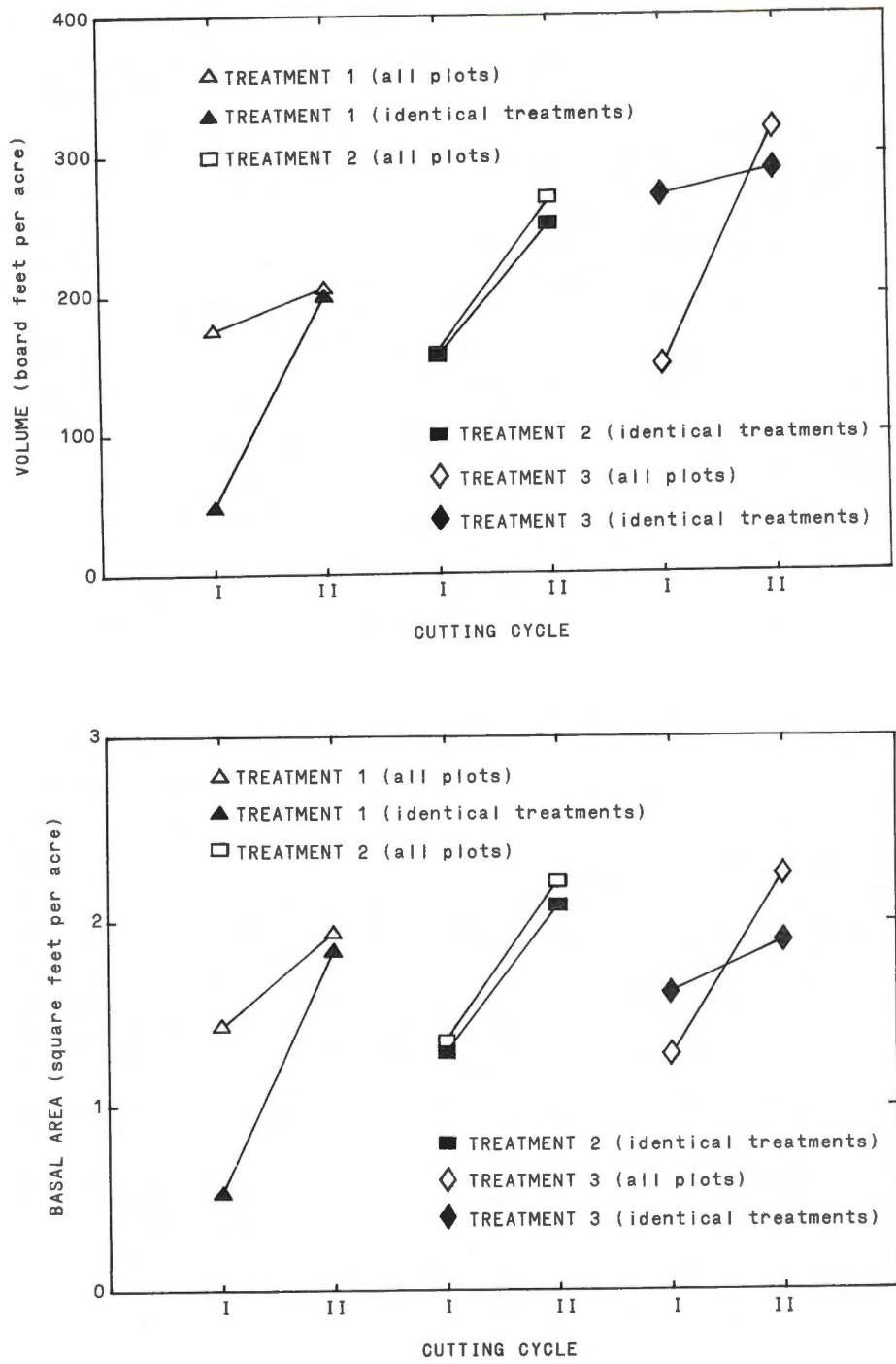
FIGURE 2. Annual volume and basal area increment by treatment for each cutting cycle for all plots and for plots receiving identical treatments during both cutting cycles.
