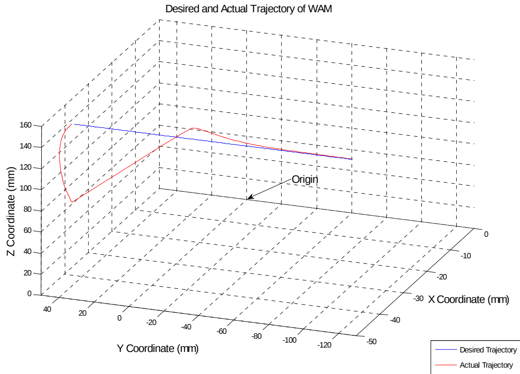
Fig 6.2 Comparison of desired and actual trajectory for WAM
