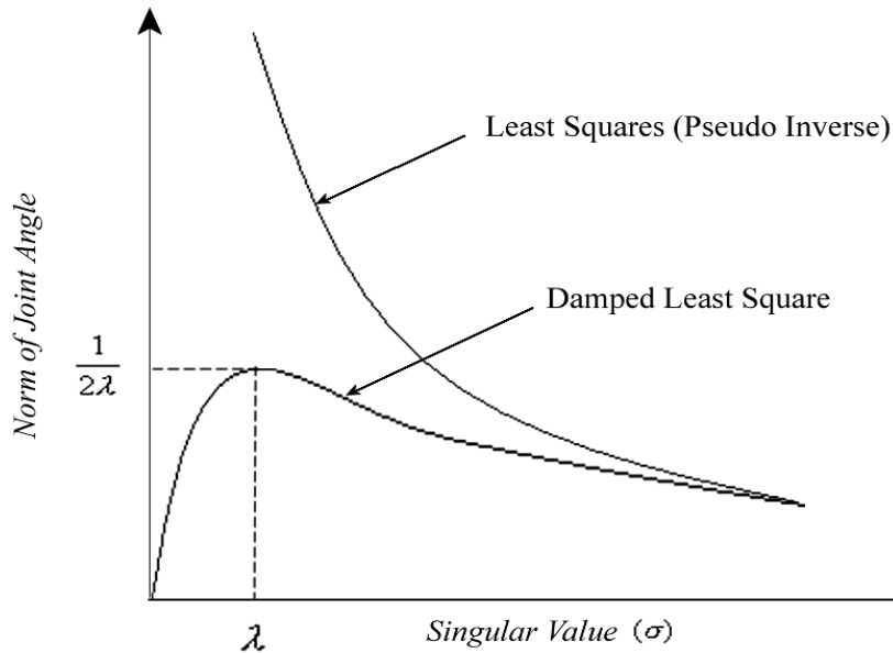
Fig 4.2. Damped Least Square Solution versus Least Square Solution
