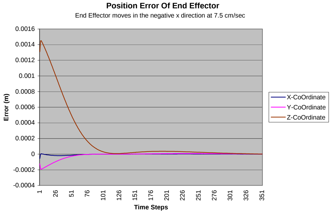
Fig 6.12 End Effector position tracking error for a different trajectory
