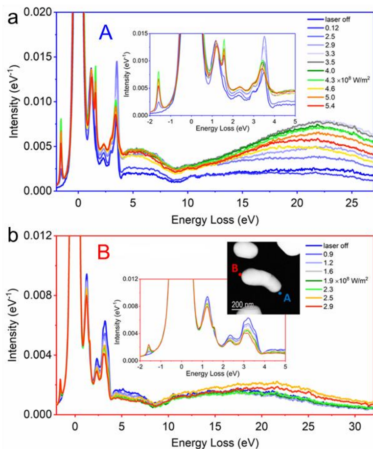
Fig. 5.6 The unprocessed low-loss EEL/EEG point spectra of a photothermally dewet silver nanoparticles as a function of laser irradiance (W/m 2 ) for the Positions A and B in Fig. 5.5 .
