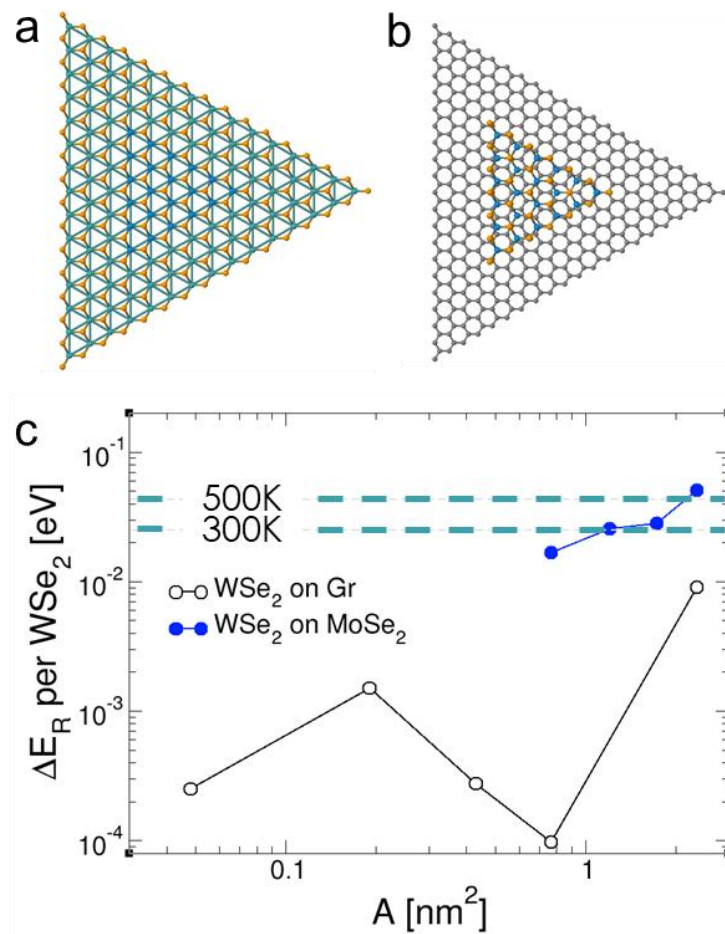
Fig. 3.14 The aligned ( \theta = 0 ) stacking configuration of the heterostructures of \text{WSe}_2/\text{MoSe}_2 (a) and \text{WSe}_2/\text{Gr} (b). (c) Rotational energy barrier ( \Delta E_R ) depending on the size of the \text{WSe}_2 nanoflake, translated to the area ( A ), on graphene and \text{MoSe}_2 . The dash lines indicate thermal energy at room temperature (300 K) and 500 K.
