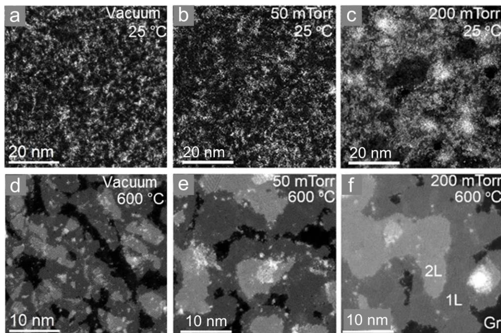
Fig. 3.3. (a-b) HAADF STEM images of amorphous tungsten selenide (a-WSe x ) deposited on graphene at 25 °C by PLD at 1 Hz (a) in vacuum (10 -6 Torr), (b) at 50 mTorr in Ar, and (c) at 200 mTorr in Ar. The number of pulses is 10 for all three conditions; and HAADF STEM images of tungsten selenide deposited at 600 °C by PLD crystallized into 1L-2L WSe 2 domains at 1Hz (d) in vacuum, (e) at 50 mTorr Ar, and (f) at 200 mTorr Ar. The number of pulses is 25 for all three conditions.
