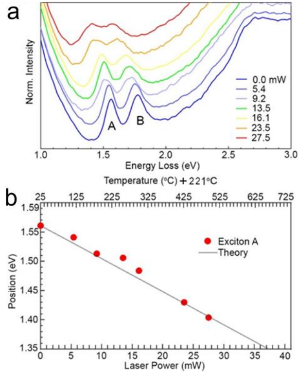
Fig. 2.4 Laser power dependence of EEL spectra measured for suspended 1L MoSe 2 on holey SiN x grid at 77 K in cryo-TEM holder within a Libra 200MC with energy resolution of 0.14 eV. (a) Excitonic band-shifts of MoSe 2 for different laser powers (illuminating tilted 5-mm spot). (b) Laser intensity dependence of the peak positions of exciton A and correlation of temperature with laser power, where the temperature scale has been adjusted for comparison with the in situ laser heating of room temperature (298 K) substrates in our experiments by +221°C (= 298 K – 77 K).
