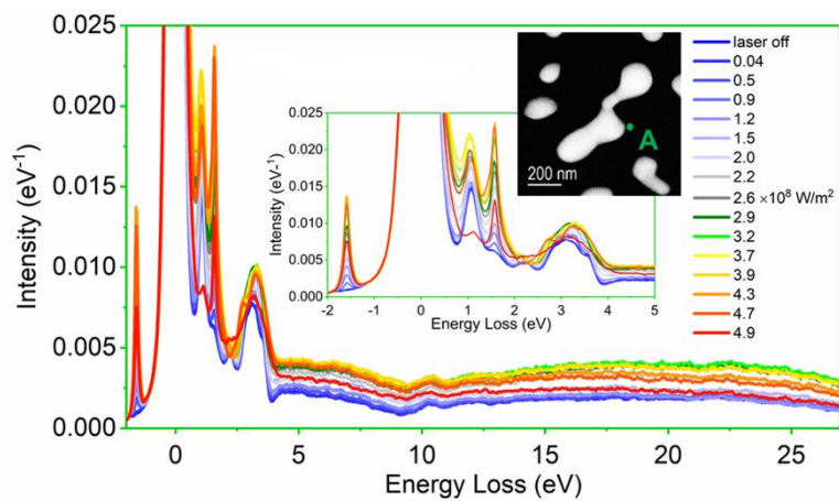
Fig. 5.4 The unprocessed low-loss EEL/EEG point spectra of a photothermally dewet silver nanoparticles as a function of laser irradiance ( \text{W/m}^2 ) for the Position A in Fig. 5.3.
