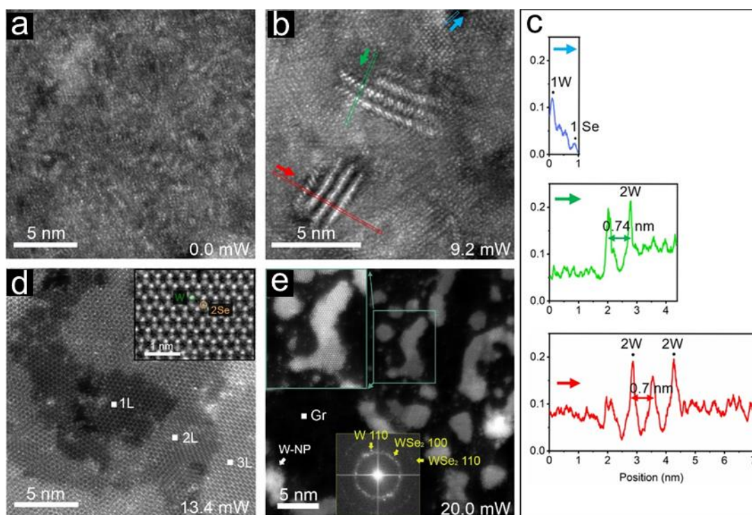
Fig. 3.9 Atomic-resolution ex situ HAADF-STEM characterization of the evolution of PLD-deposited tungsten selenide on graphene grids after sequential in situ laser treatments within a TEM. (a) \text{a-WSe}_x precursor prior to laser exposure. (b) After the laser treatment to 9.2 mW, the Se-rich film is crystallized in a variety of orientations and intermediate phases, including the vertically aligned \text{WSe}_{2+x} domains. (c) Intensity profiles of blue, green and red frames in Fig. 5b, revealing that the vertically aligned domains are only 2-layers tall and have a variety of layer spacings (0.7 and 0.74 nm). (d) After further laser treatment to 13.4 mW, the film has transformed completely into planar \text{WSe}_2 layers. Inset shows an atomically resolved HAADF image of 2H- \text{WSe}_2 monolayer structure on Gr. (e) After further exposure to 20 mW, the 2H- \text{WSe}_2 layered film on graphene decomposed into a Se-deficient network comprised of \text{WSe}_2 and W nanoparticles after being exposed to high-power laser. Inset in the upper left corner shows a dendritic structure with a portion of remaining (001) \text{WSe}_2 structure; Fast Fourier transformation (FFT) of the whole image in the bottom inset shows diffraction spots of \text{WSe}_2 and metallic W.
