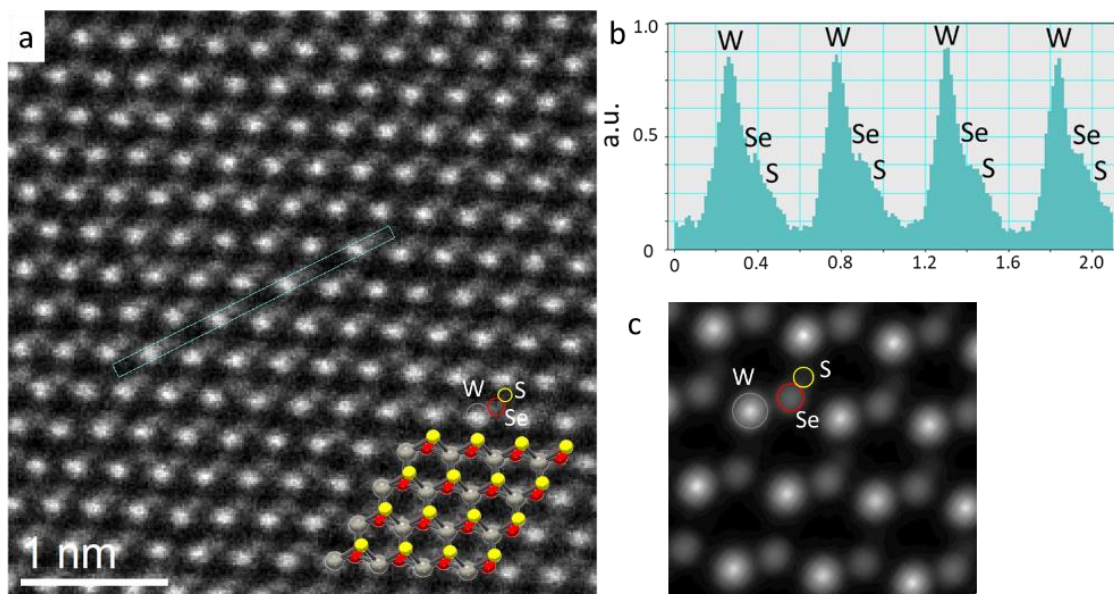
Fig. 4.5 Tilted HAADF-Z-STEM images of ML Janus WSSe (a) Experimental image tilted at x = +15^\circ along with overlaid ball-and-stick model with W atoms (gray), Se atoms (red) and S atoms (yellow). (b) The line intensity profile across the atomic chain highlighted by the green box in (a) shows the relative intensity of detected electrons compared to the W peak, with definable shoulders of Se, then S, in a repeating pattern. (c) The corresponding simulated STEM image for Janus WSSe tilted at x = +15^\circ , confirms the relative intensity ratio measured experimentally.
