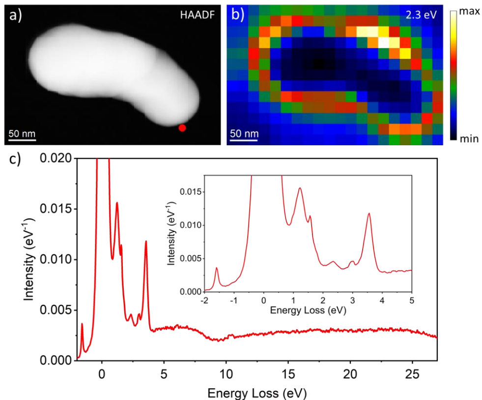
Fig. 5.8 (a), HAADF image of the beam shown in Figure 3b. (b), An EEL map of a 2.3 eV quadrupole mode excited in the beam. Note the SEEL probability map for the internal positions of the relatively thick silver contains a diffraction artifact thus they may be ignored as no modes exist for the internal position at this energy (yellow and white spots in b). (c), A representative single spectrum of red-dot pixel marked in a.
