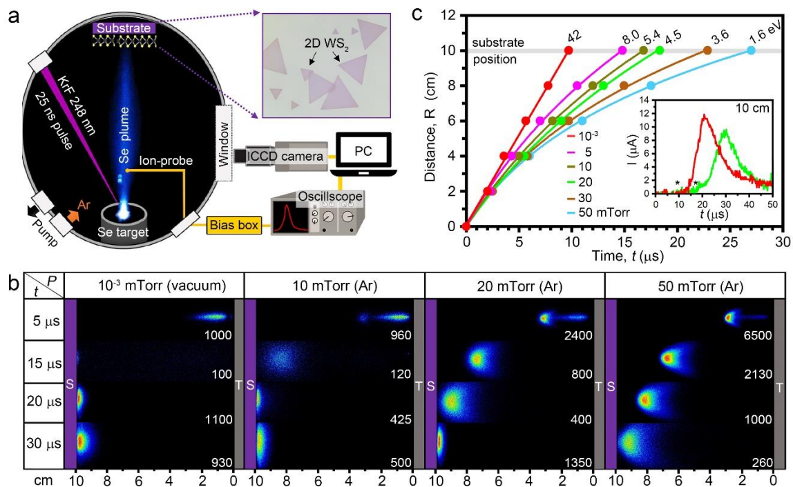
Fig. 4.1 In situ diagnostics of Se plasma plumes. (a) Experimental setup for Se plasma plume generation and impingement on CVD-grown \text{WS}_2 ML within a vacuum chamber equipped with an ICCD camera and a translatable probe for ion-flux measurement. (b) False color, gated-ICCD images of the Se plasma's visible luminescence reveal the plume's propagation dynamics through vacuum and 10, 20, and 50 mTorr argon background gas pressures at the indicated delay times following the laser pulse. (Gate width is 10% of each delay time, maximum intensity is shown for comparison.) (c) R-t plots of the leading edge of the plasma (from ion probe currents, see * in inset) track the propagation and deceleration in different background Ar pressures.
