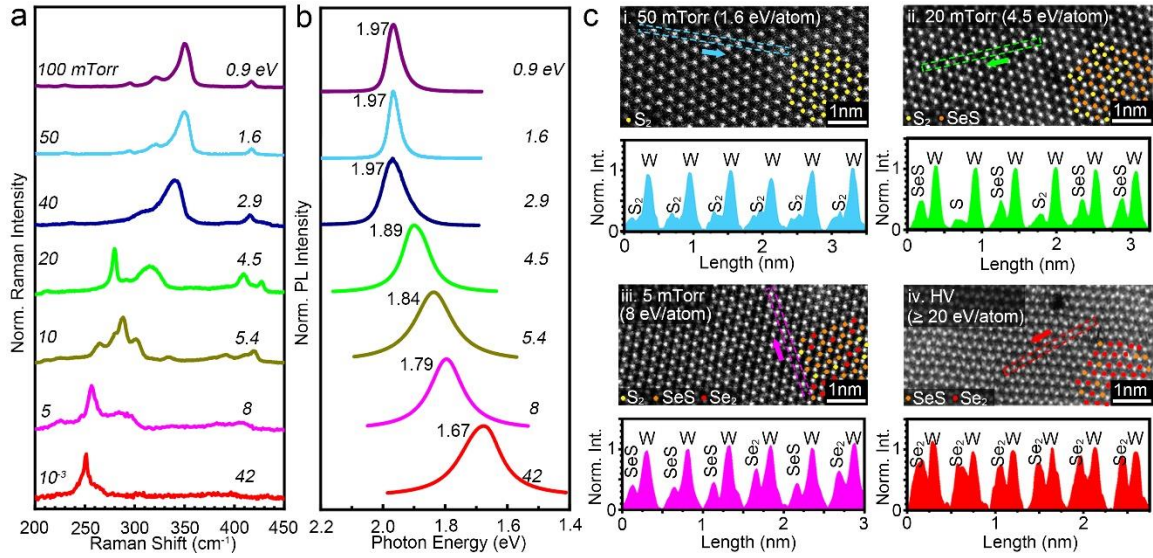
Fig. 4.2 Characterizations of \text{WS}_{2(1-x)}\text{Se}_{2x} ML converted from \text{WS}_2 by Se plasma plumes. (a) Raman spectra of \text{WS}_2 ML on \text{SiO}_2/\text{Si} substrates exposed by 800 Se plasma plume pulses in different background Ar pressures at 250 °C. (b) Corresponding PL spectra and peak energy positions of the irradiated \text{WS}_2 MLs measured in (a). (c) HAADF Z-contrast STEM images of \text{WS}_2 ML suspended on TEM grids and irradiated by Se plasma plumes arriving through Ar pressures with maximum KEs: i) 50 mTorr (1.6 eV/atom, 800 pulses), ii) 20 mTorr (4.5 eV/atom, 800 pulses), iii) 5 mTorr (8 eV/atom, 600 pulses), and iv) 10^{-6} Torr ( \geq 20 eV/atom, 600 pulses). Chalcogen columns containing S-S, Se-S, and Se-Se pairs in the images are labeled with yellow, orange, and red balls based on their Z-contrast intensity (based on Z^{1.9} scaling) with respect to W. The line profiles below each panel compare the relative Z-contrast intensity between W and dichalcogenide sites.
