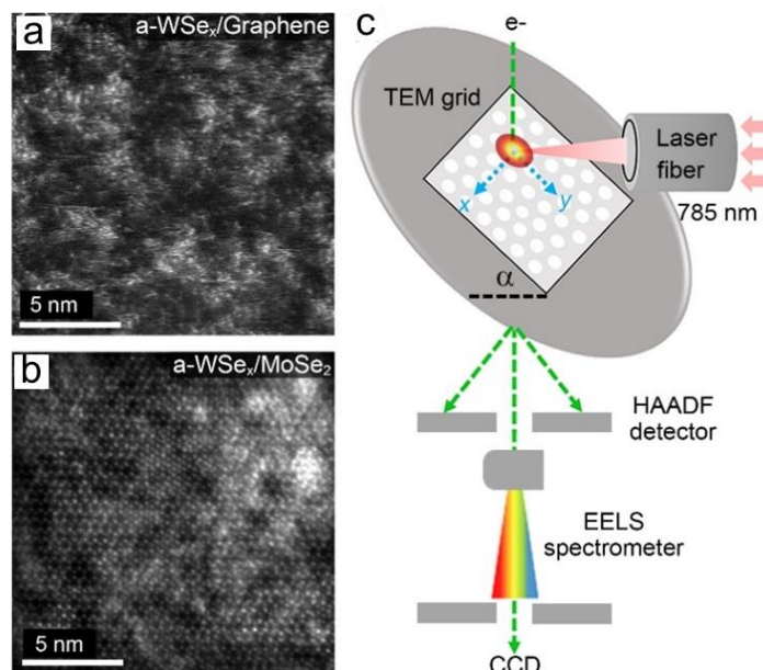
Fig. 3.5 Setup for the laser crystallization experiments within a TEM. (a-b) HAADF-STEM images showing the \text{WSe}_x precursors deposited from 40 PLD shots from a \text{WSe}_2 target in vacuum onto 1L Gr (a) and \text{MoSe}_2 (b) crystals transferred onto holey silicon nitride grids. The precursors are amorphous, consist of enough material to form a continuous monolayer, and are comprised of atomic clusters and chains. The underlying crystalline \text{MoSe}_2 substrate is evident in (b). (c) Illustration of the in situ observation arrangement within the HRTEM incorporating laser processing. The grid is tilted at \alpha = 40^\circ , a 785-nm fiber laser is focused to an ellipse ( a = 5.2 \mu\text{m} and b = 3.7 \mu\text{m} ) onto the silicon nitride grid and exposed crystal, and the electron beam is available for EELS, SAED, or HAADF imaging.
