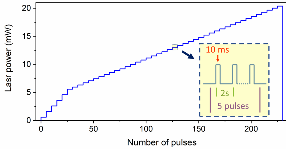
Fig. 3.6 Increment of laser power with number of pulses for both the crystallization experiments of WSe 2 /graphene in Fig. 3.7, and WSe 2 /MoSe 2 in Fig. 3.10.
