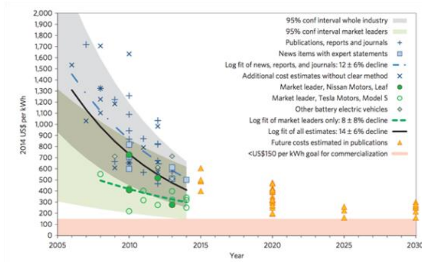
Figure 4 Cost estimates and future projections for electric vehicle battery packs, measured in $US per kilowatt hour of capacity. Each mark on the chart represents a documented estimate reviewed by the study. (Nykqvist and Nilsson 2015)
