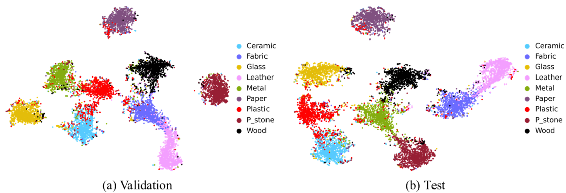
Figure 5.4. The Barnes-Hut t-SNE [33] visualization of CNN features on (a) validate; and (b) test dataset. Note: for Barnes-Hut t-SNE, 1110 images for each material class were randomly selected. The feature map before the classifier was extracted and used for t-SNE visualization
