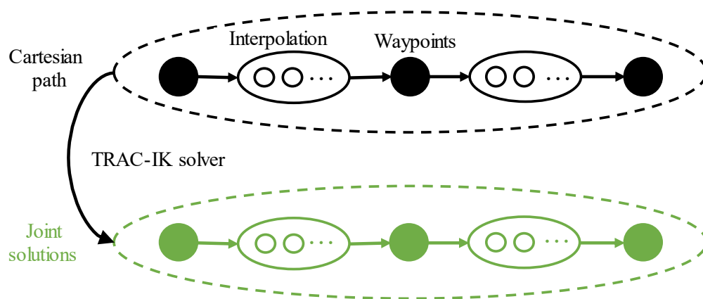
Figure 6.8. Flowchart to generate a trajectory from waypoints
