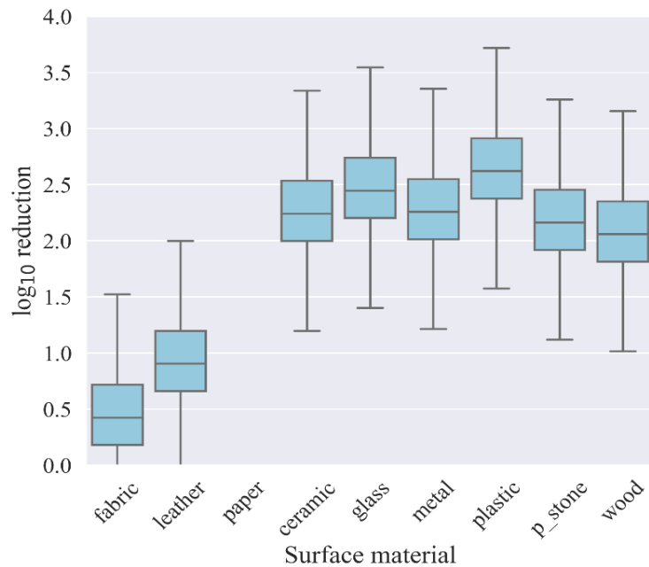
Figure 6.12. Boxplot of log 10 reduction for different surfaces contaminated by SARS-CoV-2
