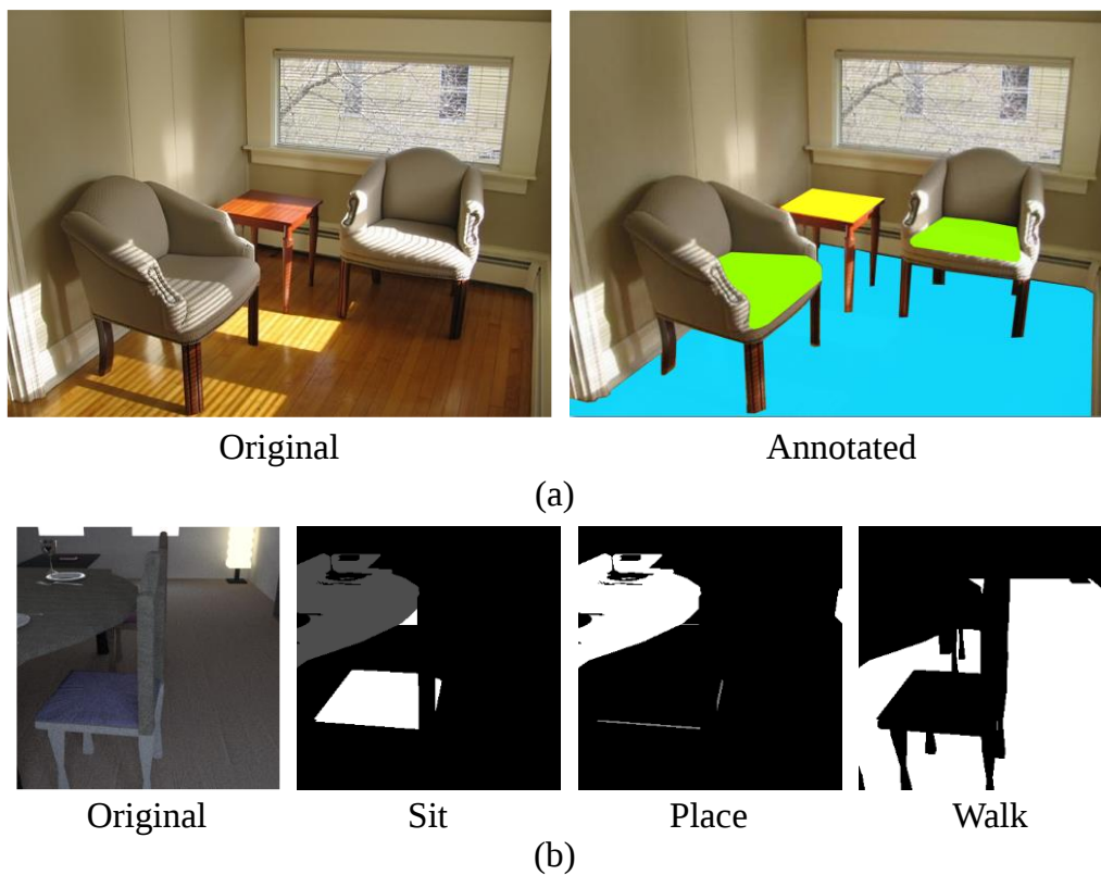
Figure 4.3. Example of annotated dataset. (a) using transfer table to transform original object labels in ADE20K dataset to affordance labels (green (seat base - sit); yellow (tabletop - place); blue (floor - walk)); and (b) annotated simulated image
