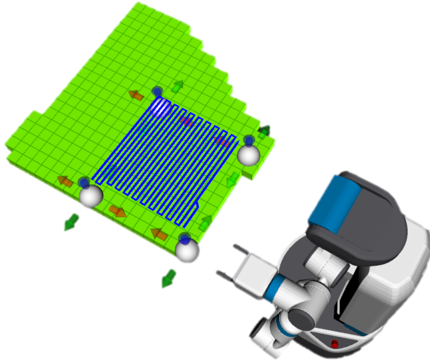
Figure 6.7. RViz interface with markers placed on the 3D map. The blue lines represent the disinfection trajectory with a certain distance to the surface
