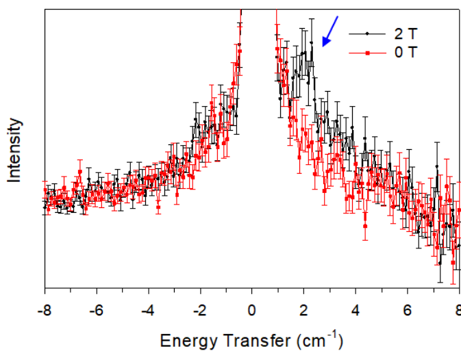
Figure 3.8. INS spectrum of (PPh 4 ) 2 [Co(NO 3 ) 4 ]·CH 2 Cl 2 ( 4 ) at 1.7 K, showing the M_s = -1/2 \rightarrow +1/2 transition at 2 T (indicated by the blue arrow) with the incident neutron energy of E_i = 13.4 cm -1 , |Q| = 0.4 -1.3 Å -1 . The solid lines are for eye guide.
