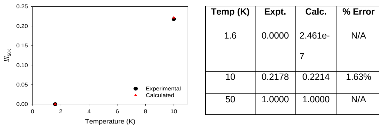
Figure A.13: (Left) Experimental and calculated intensities vs. temperature for the -2D peak in INS spectra of Fe(TPP)Br ( 2 ). At 50 K the peak is most intense. Therefore, it was used to scale the rest of the temperatures. (Right) Table of error calculations comparing the intensities.
