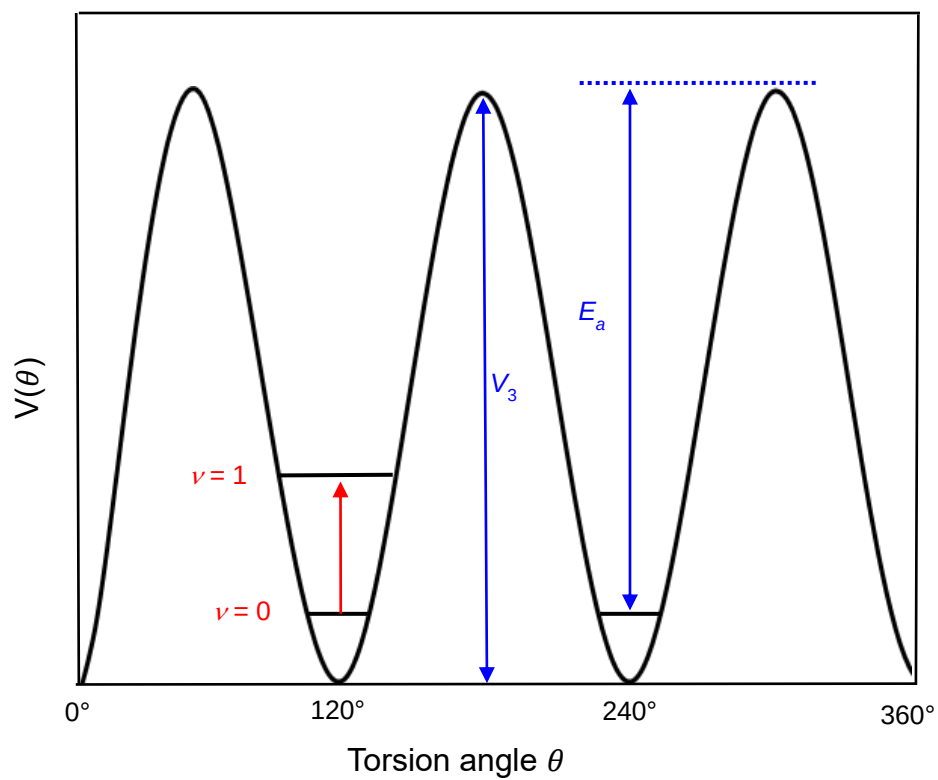
Figure 5.3. Torsion and rotation of a methyl group. E_a is the activation energy of the methyl rotations; \nu = 0 is the ground torsional level; V_3 is the 3-fold barrier height.
