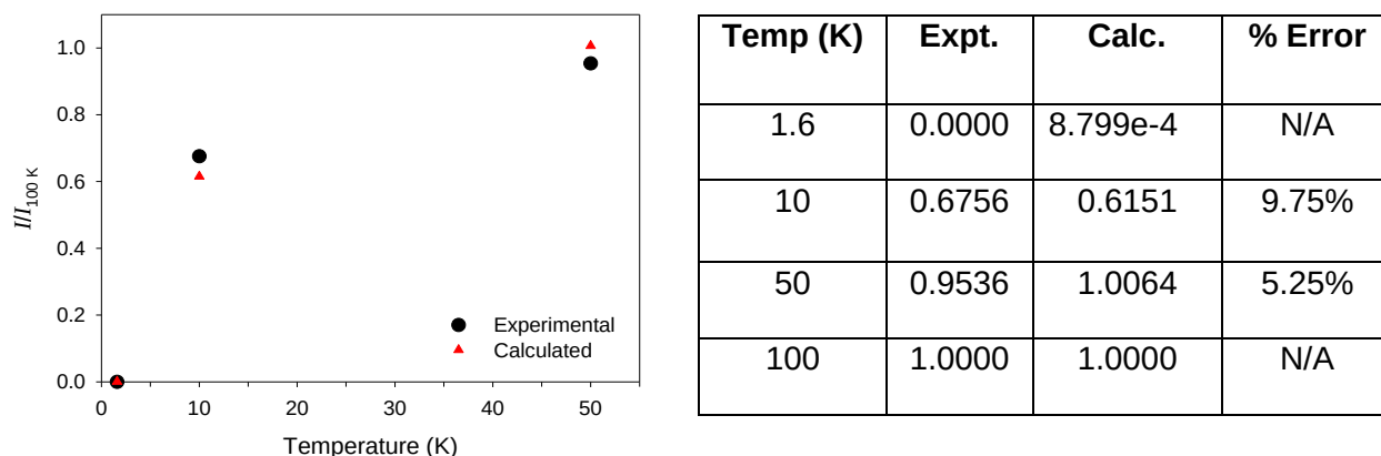
Figure A.7: (Left) Experimental and calculated intensities vs. temperature for the 4D peak in INS spectra of Fe(TPP)F ( 1 ). At 100 K the peak is most intense. Therefore, it was used to scale the rest of the temperatures. (Right) Table of error calculations comparing the intensities.
