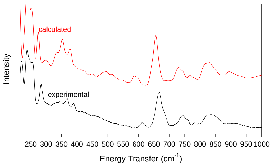
Figure 3.28. Calculated and experimental 5 K INS spectra of 10 . (Top) The 0-250 \text{cm}^{-1} range. (Bottom) The 250-1000 \text{cm}^{-1} range.
