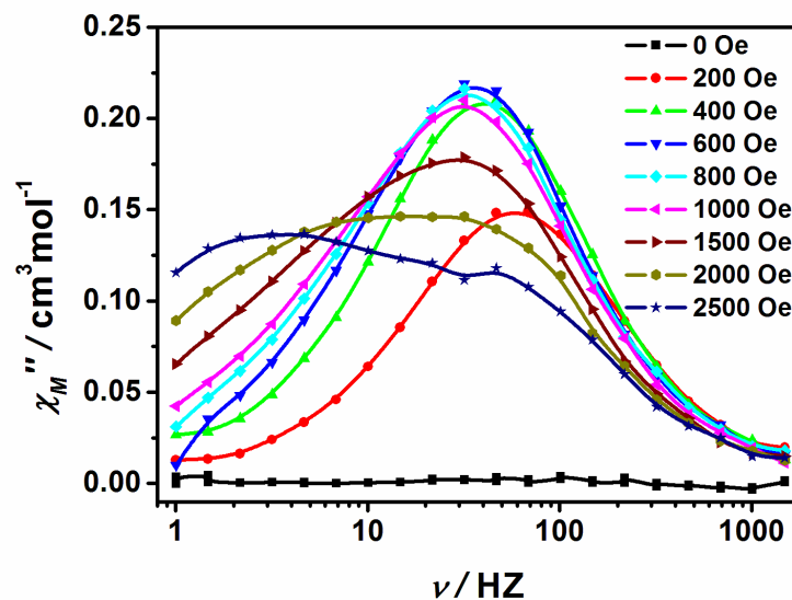
Figure B.13. Frequency dependence of out-of-phase ( \chi_M'' ) AC susceptibility at 1.8 K under the different applied static fields from 0 to 2500 Oe for (\text{MePPh}_3)_2[\text{Co}(\text{NO}_3)_4] (5). The solid lines are for eye guide.
