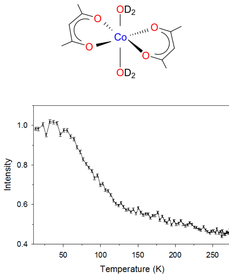
Figure 5.1. (Top) Structure of 8-d 4 . (Bottom) Fixed window elastic scattering neutron intensity scan at |Q| = 0.3 \text{ \AA}^{-1} between 2 and 275 K. |Q| dependence of the fixed window scan is shown in Figure C.1.
