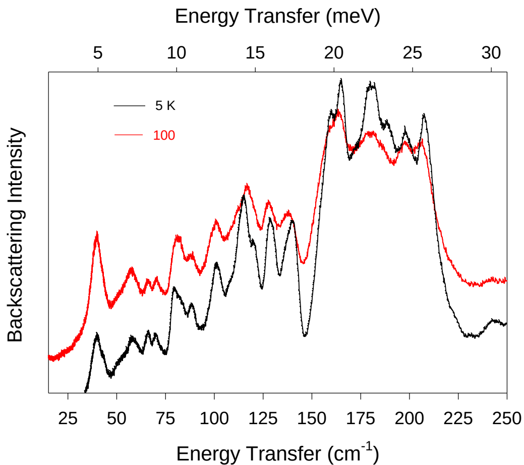
Figure C.5. VISION spectra at 5 and 100 K showing the strongest methyl torsion peak at 164 cm -1 (20.3 meV) in Co(acac) 2 (D 2 O) 2 ( 8-d 4 )..
