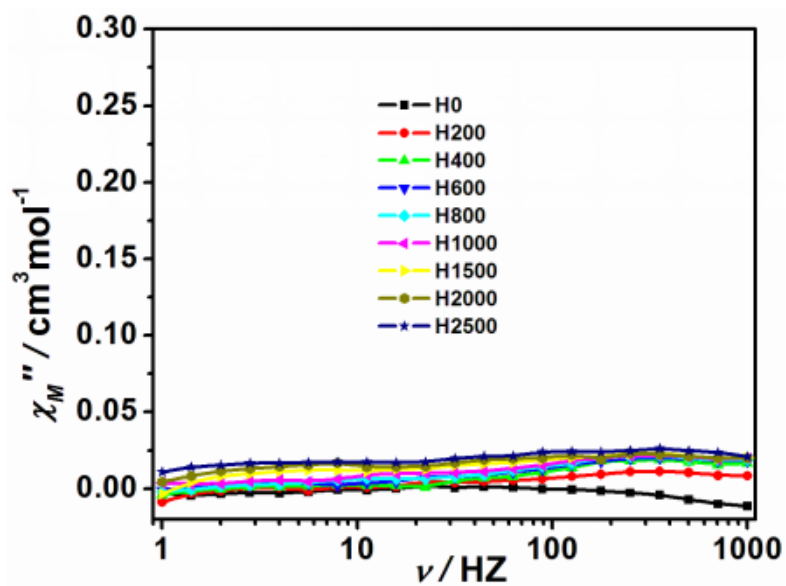
Figure B.14. Frequency dependence of out-of-phase ( \chi_M'' ) AC susceptibility at 1.8 K under the different applied static fields from 0 to 2500 Oe for (\text{AsPh}_4)_2[\text{Co}(\text{NO}_3)_4] ( 6 ). The solid lines are for eye guide.
