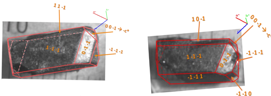
Figure 3.13. Crystals of [\text{Co}(\text{12C4})_2](\text{l}_3)_2(\text{12C4}) (7) that were orientated at TOPAZ with miller indices shown. The c^* axis is indicated. The red lines are an overlay of the predicted crystal faces.
