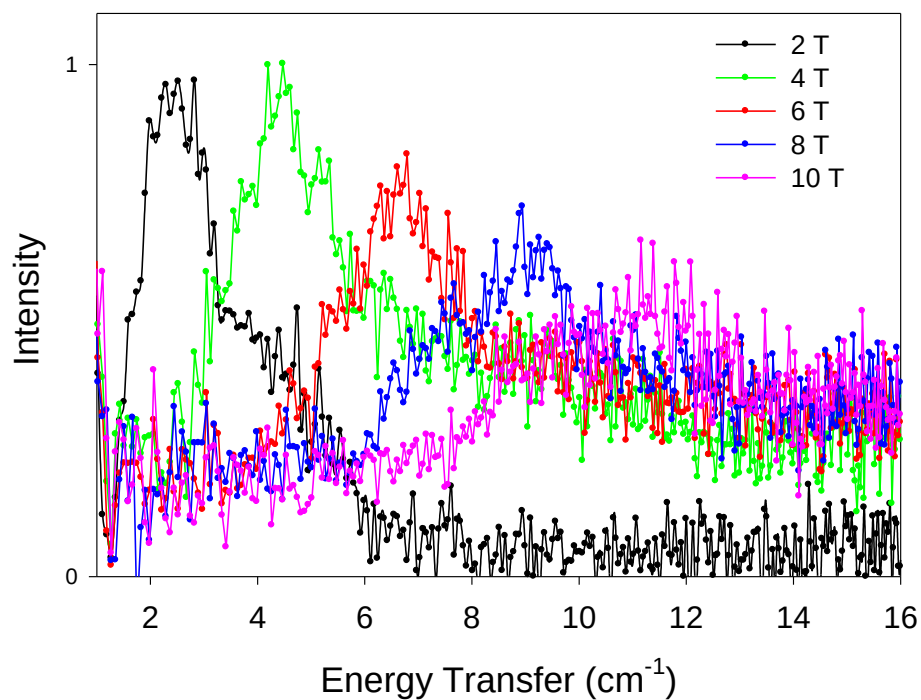
Figure 3.23. Variable-magnetic-field INS of 8-d 18 at DCS, revealing the \phi_1 \rightarrow \phi_2 transition (Figure 3.3b) at 1.7 K.
