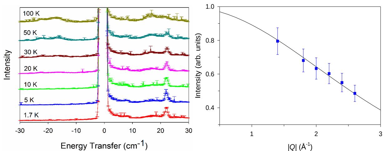
Figure 3.7. (Left) INS spectra of (PPh 4 ) 2 [Co(NO 3 ) 4 ]·CH 2 Cl 2 ( 4 ) with incident neutron energy E_i = 53.7 cm -1 , |Q| = 0.5 -1.3 Å -1 and a step size of 0.081 cm -1 . (Right) Change in intensities of the magnetic peak at 22.5(2) cm -1 vs |Q| at 1.7 K. The solid line represents the calculated intensity of the magnetic excitation.
