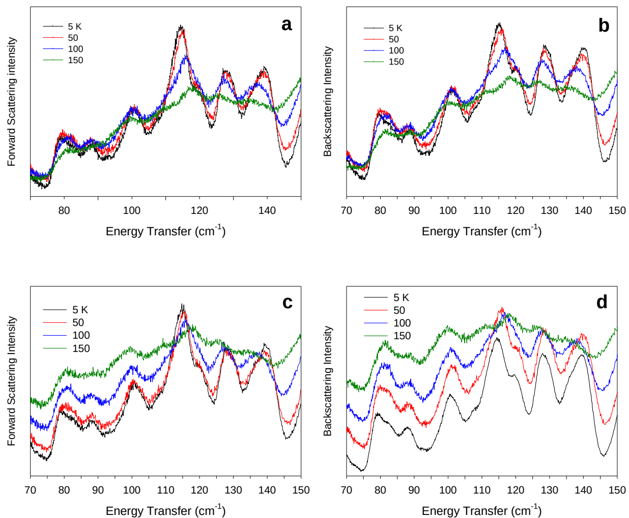
Figure B.17. (a) Forward scattering (low |Q| ), Bose-corrected spectra of \text{Co}(\text{acac})_2(\text{D}_2\text{O})_2 8-d 4 . (b) Backscattering intensity (high |Q| ), Bose-corrected spectra of 8-d 4 . (c) Forward scattering, non-Bose-corrected spectra of 8-d 4 . (d) Backscattering, non-Bose-corrected spectra of 8-d 4 . Spectra collected at VISION.
