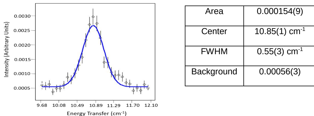
Figure B.3. Typical magnetic peak of (AsPh 4 ) 2 [Co(NO 3 ) 4 ] ( 6 ) used for determination of magnetic transition and calculation of the 2(D^2 + 3E^2)^{1/2} value ( E_i = 24.2 \text{ cm}^{-1} , 10 K).
