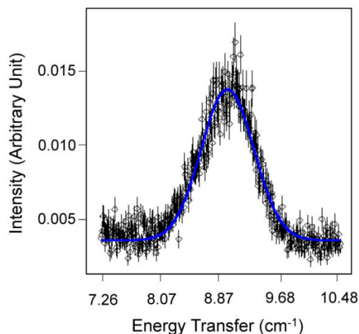
Figure A.5. Typical first magnetic peaks of for Fe(TPP)F ( 1 ) used for calibration of the elastic peak and calculation of the D value ( E_i = 24.17 cm -1 , 10 K). FWHM = Full width at half maximum.
