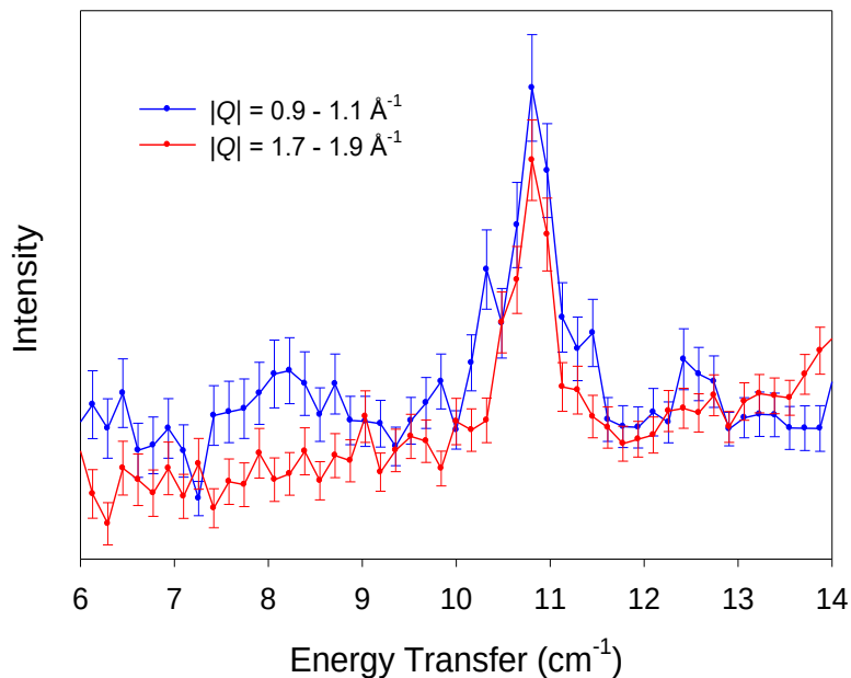
Figure B.7. INS spectra of (\text{AsPh}_4)_2[\text{Co}(\text{NO}_3)_4] ( 6 ) at 1.6 K showing a comparison of the ZFS transition at different |Q| ranges. The baseline of the peak has been corrected.
