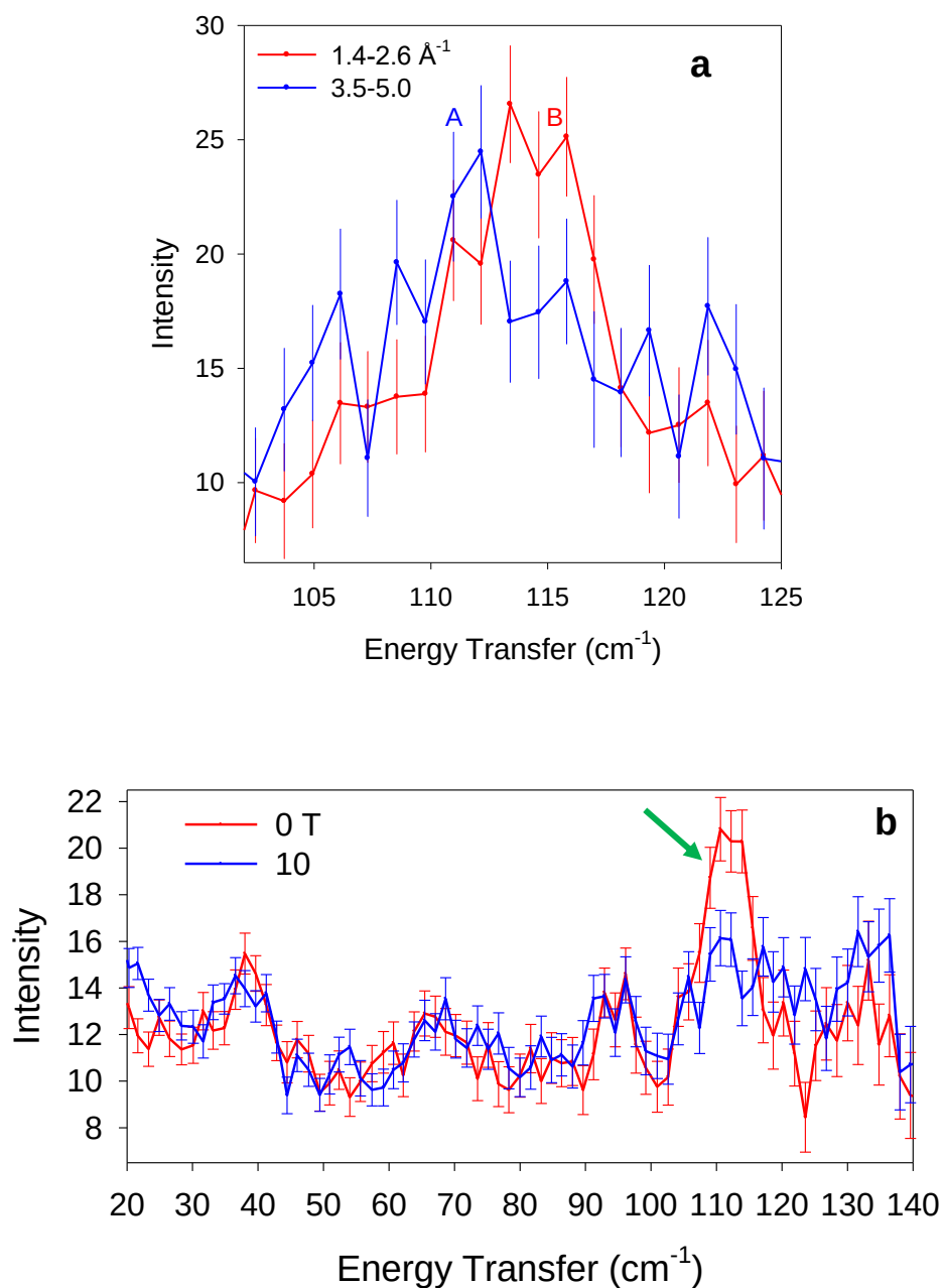
Figure 3.19. (a) 0 T INS spectra at small |Q| (1.4–2.6 \text{\AA}^{-1} ) and large |Q| (3.5–5.0 \text{\AA}^{-1} ). (b) Variable-field INS spectra of 8-d 18 at 0 and 10 T summed over all |Q| . The green arrow represents peaks A and B at 0 T.
