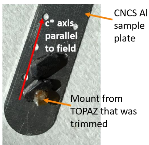
Figure 3.14. Crystals of [\text{Co}(\text{12C4})_2](\text{l}_3)_2(\text{12C4}) (7) that were orientated for the CNCS experiment (prior to wrapping the sample plate with Al wires to keep the crystals in position in the magnetic field). Note the mount from the TOPAZ experiment was glued on the crystal and was not able to be removed for the CNCS experiment.
