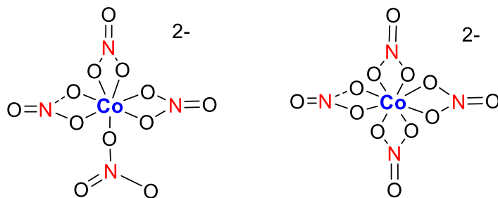
Figure 3.1. Structures of the anions (A) 2 [Co(NO 3 ) 4 ] (left) 4/5 and (right) 6 .
