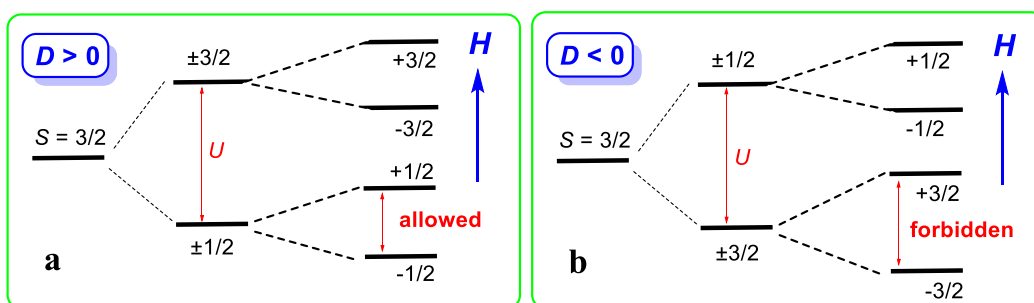
Scheme 3.2. (a) ZFS energy diagram, D > 0 with the application of a magnetic field. (b) ZFS energy diagram, D < 0 with the application of a magnetic field. U = 2(D^2 + 3E^2)^{1/2} .
