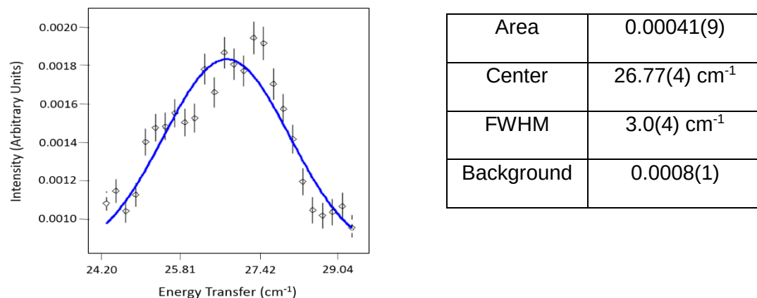
Figure B.2. Typical magnetic peak of (MePPh 3 ) 2 [Co(NO 3 ) 4 ] ( 5 ) used for determination of magnetic transition and calculation of the 2(D^2 + 3E^2)^{1/2} value ( E_i = 40.3 \text{ cm}^{-1} , 1.6 K).
