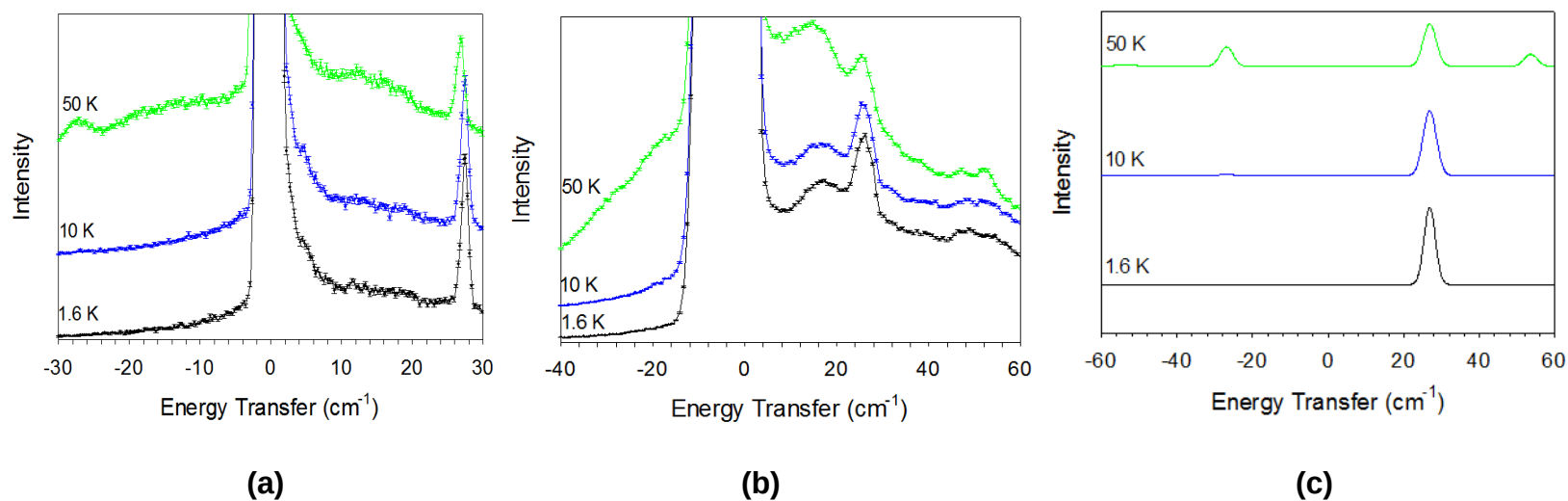
Figure 2.3. (a) INS spectra of Fe(TPP)I (3) with E_i = 40.89 \text{ cm}^{-1} , Q = 0.5\text{-}1.0 \text{ \AA}^{-1} and a step size of 0.024 \text{ cm}^{-1} . (b) INS spectra with E_i = 97.35 \text{ cm}^{-1} , Q = 0.48\text{-}1.8 \text{ \AA}^{-1} and a step size of 0.024 \text{ cm}^{-1} . (c) Theoretical INS spectra of an S = 5/2 spin system with D = 13.4 \text{ cm}^{-1} and E = 0.3 \text{ cm}^{-1} .
