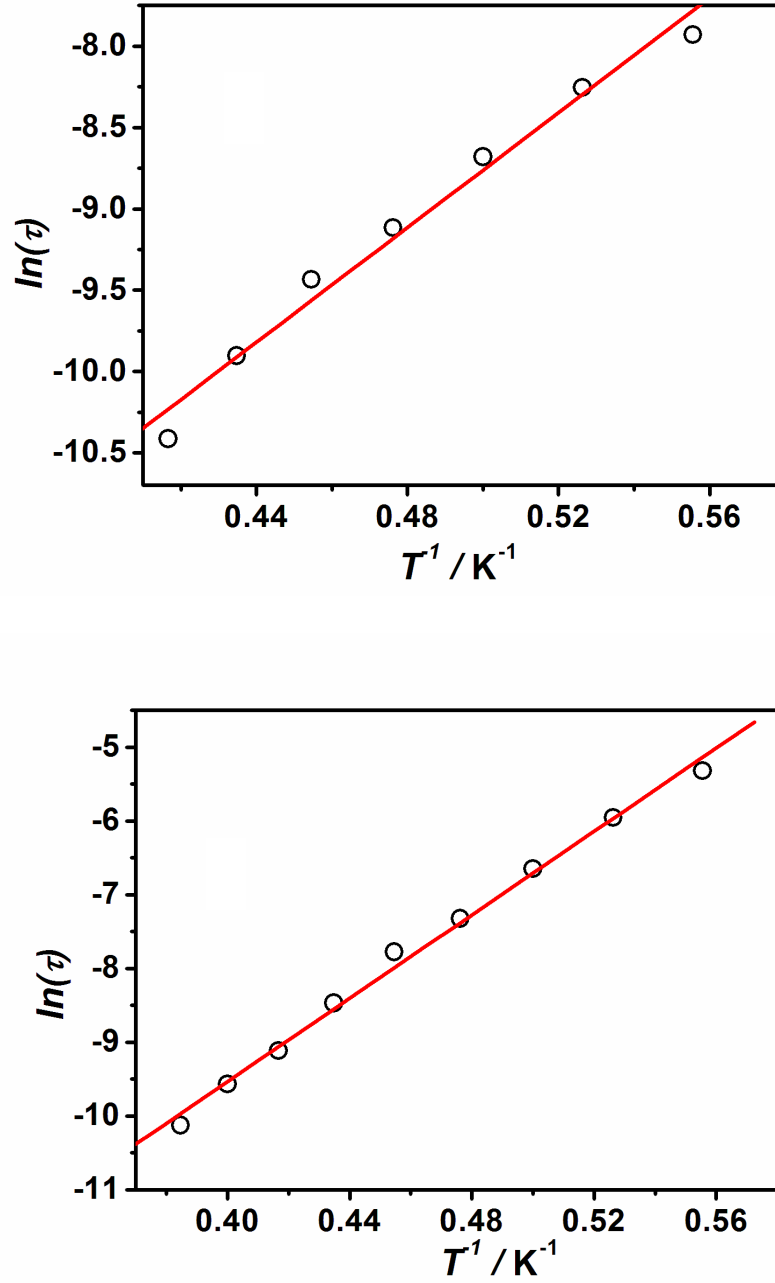
Figure 3.12. Relaxation time of the magnetization \ln(\tau) vs T^{-1} plots for (Top) 4 and (Bottom) 5 . The solid lines represent Arrhenius fits.
