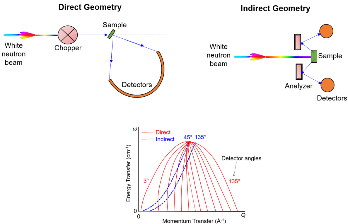
Scheme 3.1. (Top) Depiction of direct (left panel) and indirect geometry (right panel) instrumentation. (Bottom) Representation of trajectories in (Q, \omega) space for a direct geometry spectrometer with detectors at angles between 3^\circ and 135^\circ (red lines). Indirect geometry spectrometer with scattering angles of 45^\circ and 135^\circ , forward scattering and backscattering, respectively (blue dashed lines).
