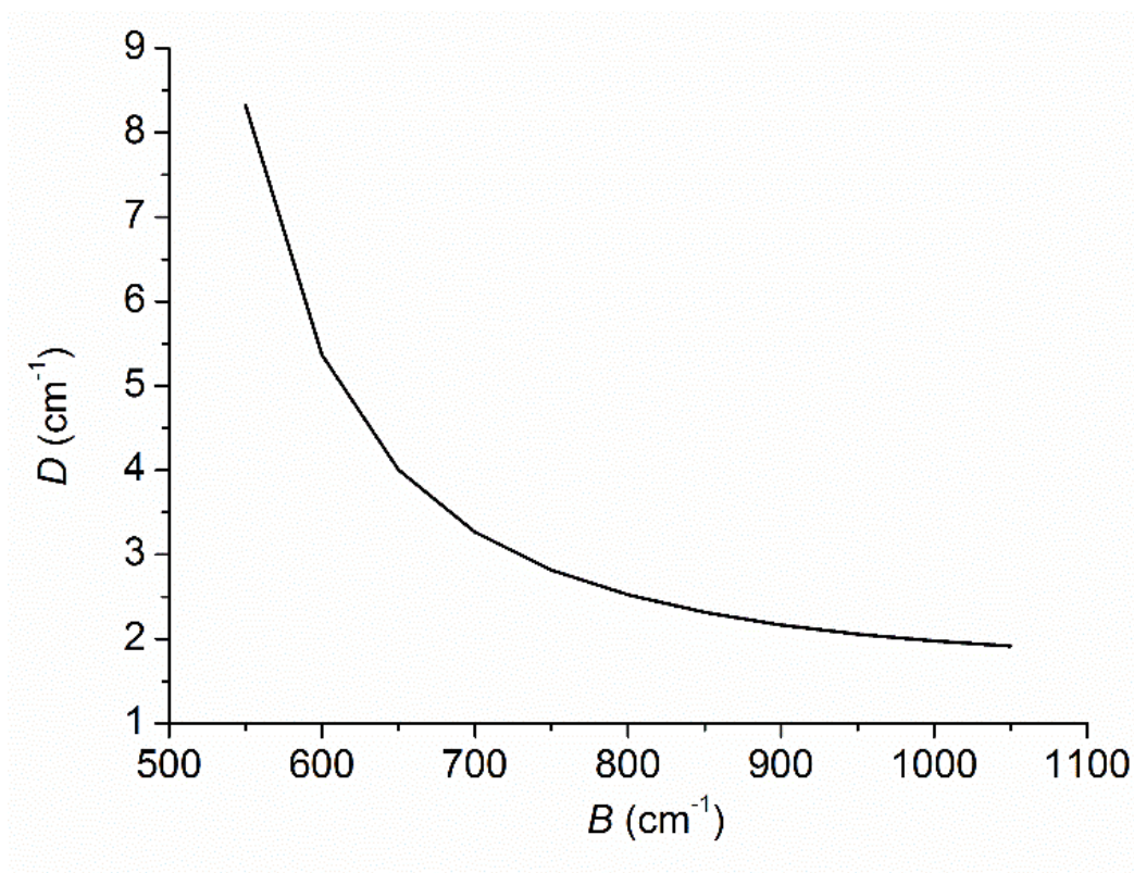
Figure 2.10. Variation of D with B for Fe(TPP)Cl taken as a model example. The figure has been constructed using the AOMX program package with model parameters set (NEVPT2) from Table 2.3. A C/B ratio of 4.63 has been adapted using the same data.
