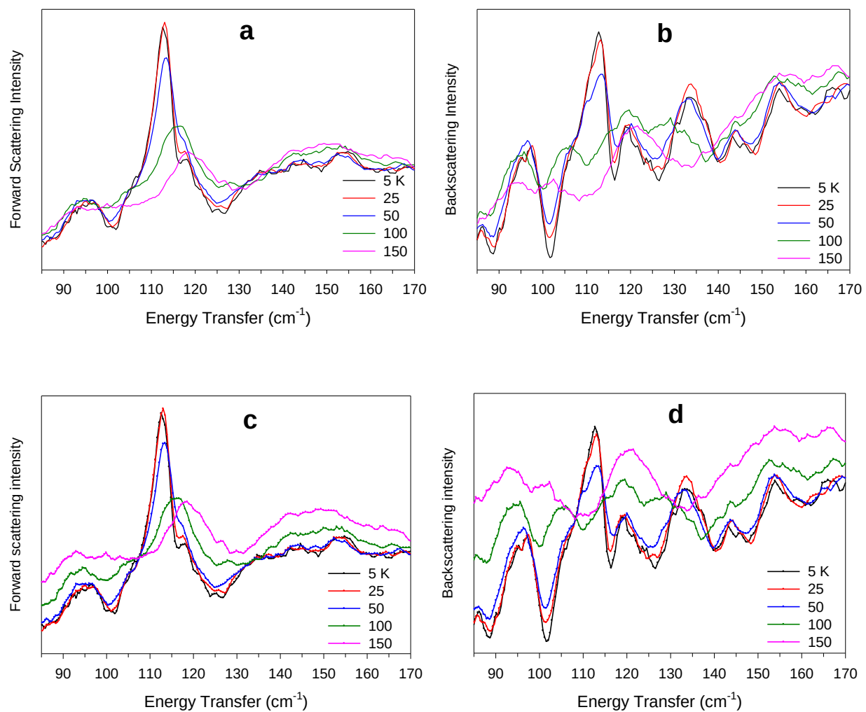
Figure B.16. (a) Forward scattering (low |Q| ), Bose-corrected spectra of Co(acac- d 7 ) 2 (D 2 O) 2 8-d 18 . (b) Backscattering intensity (high |Q| ), Bose-corrected spectra of 8-d 18 . (c) Forward scattering, non-Bose-corrected spectra of 8-d 18 . (d) Backscattering, non-Bose-corrected spectra of 8-d 18 . Spectra collected at VISION.
