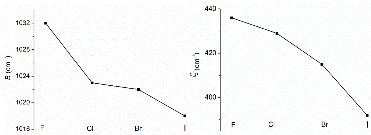
Figure A.20. Non-relativistic (left) and relativistic (right) covalence reduction of the parameters B and \zeta , respectively, from CASSCF/NEVPT2 calculations of the \text{Fe}(\text{TPP})\text{X} [ \text{X} = \text{F} ( 1 ), \text{Cl} , \text{Br} ( 2 ), \text{I} ( 3 )] series. Parameters for the plot are taken from Table 2.3.
