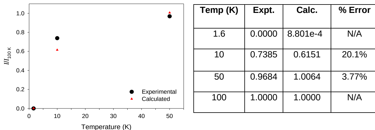
Figure A.8: (Left) Experimental and calculated intensities vs. temperature for the -2D peak in INS spectra of Fe(TPP)F ( 1 ). At 100 K the peak is most intense. Therefore, it was used to scale the rest of the temperatures. (Right) Table of error calculations comparing the intensities.
