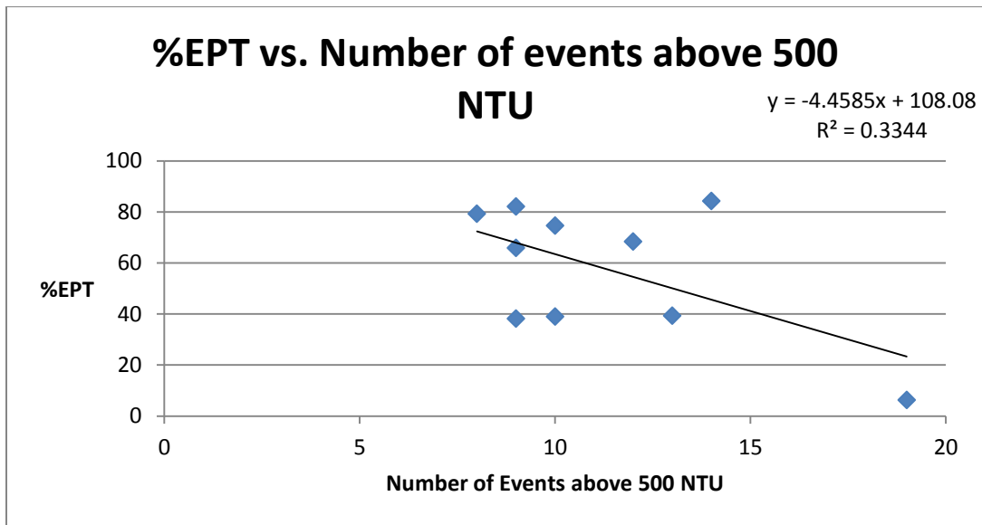
Figure 29: The relationship between the number of events above 500 NTU and the %EPT scores
