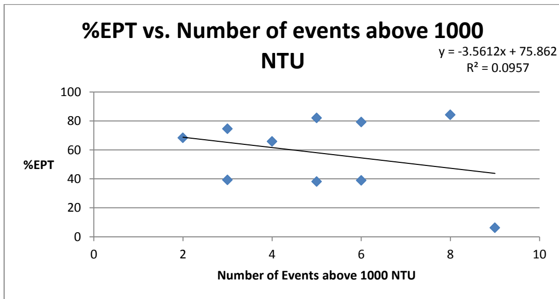
Figure 30: The relationship between the number of events above 1000 NTU and the %EPT scores
