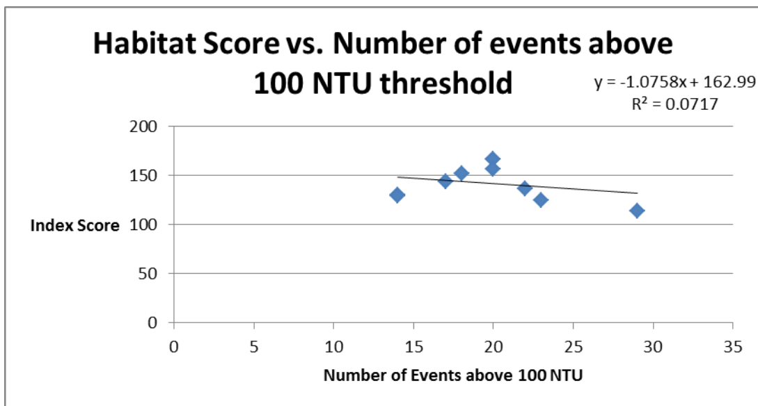
Figure 21: The relationship between the number of events above 100 NTU and the Habitat Scores
