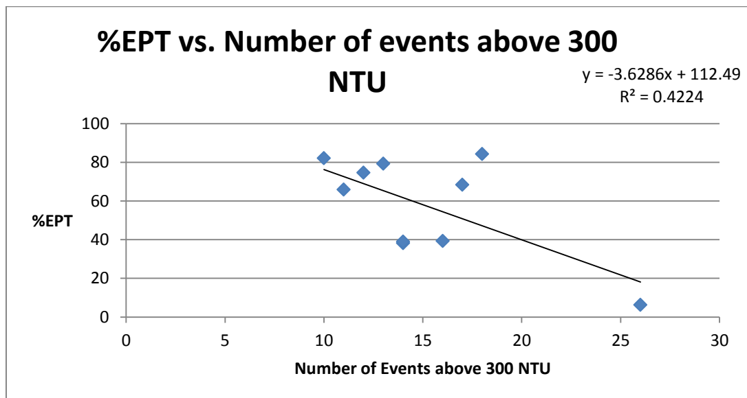
Figure 28: The relationship between the number of events above 300 NTU and the %EPT scores
