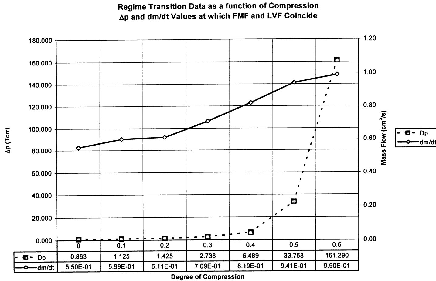
Figure 3.1. Theoretical transition values for mass flow rate, dm/dt , and pressure drop, \Delta p , at various foam compression levels.
