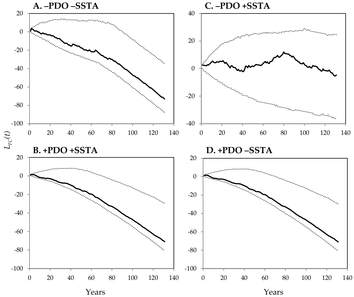
Figure 3.13: Results from the Bivariate Event Analysis testing two-way phase combinations of extreme Pacific Decadal Oscillation years and extreme climate years of the Atlantic sea surface temperature anomaly (SSTA) with large wildfire years (50% scarred class). Dashed lines are the 90% confidence envelopes and the solid black lines are the L_{hat} values.
