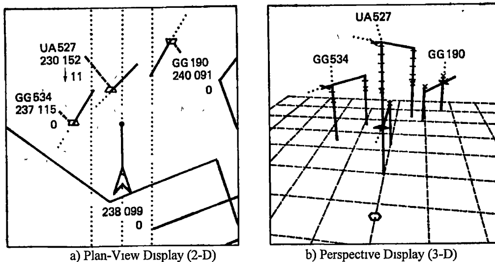
Figure 6. Plan-View and Perspective Display Formats.
