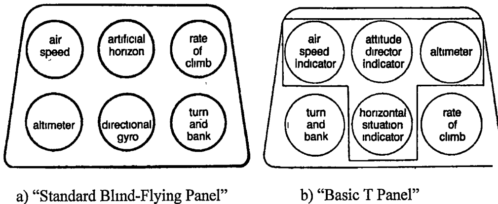
Figure 3. The Pre-War RAF "Standard Blind-Flying Panel" and "Basic T Panel."
