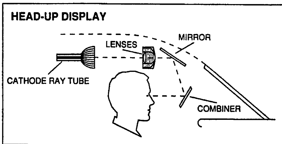
Figure 8. Head-Up Display Components.
