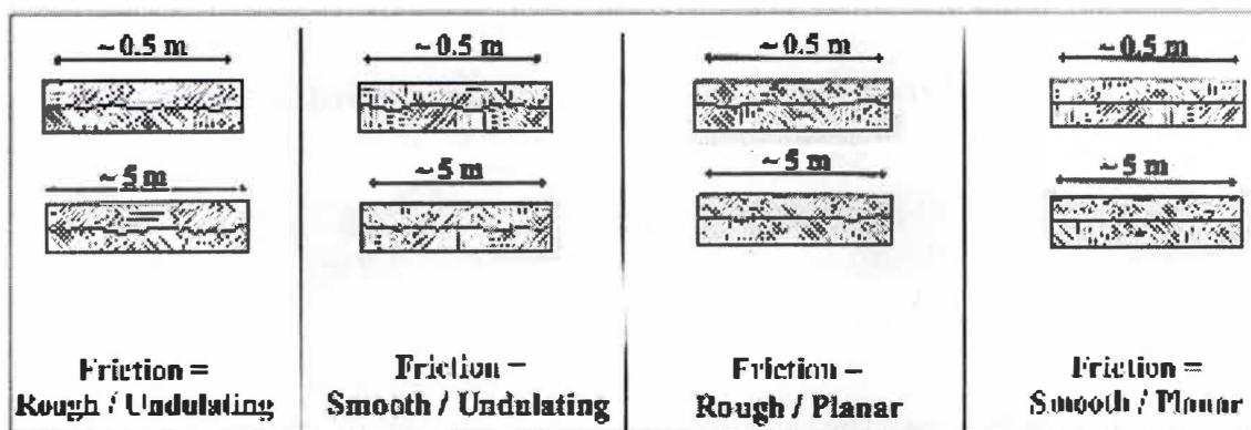
Figure A-1.4. Visual scoring aid for Friction showing micro- and macrofriction profiles.
