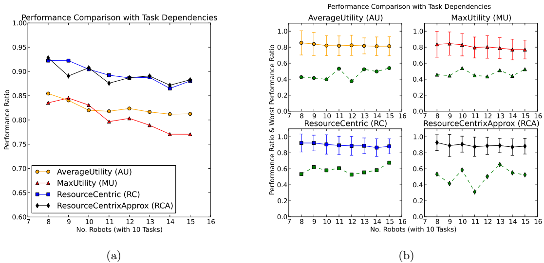
Figure 7.24: Task allocation with task dependencies with random configurations. (a) Average performance ratios. (b) Separate and more detailed average performance ratios with standard deviations. The green data points in each subgraph represent the worst performance ratios for that respective method.
