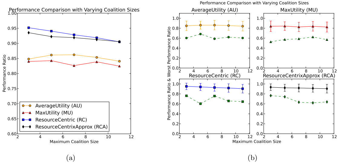
Figure 7.22: Task allocation with varying coalition sizes. (a) Average performance ratios. (b) Separate and more detailed results with standard deviations. The green data points in each subgraph represent the worst performance ratios for that respective method.
