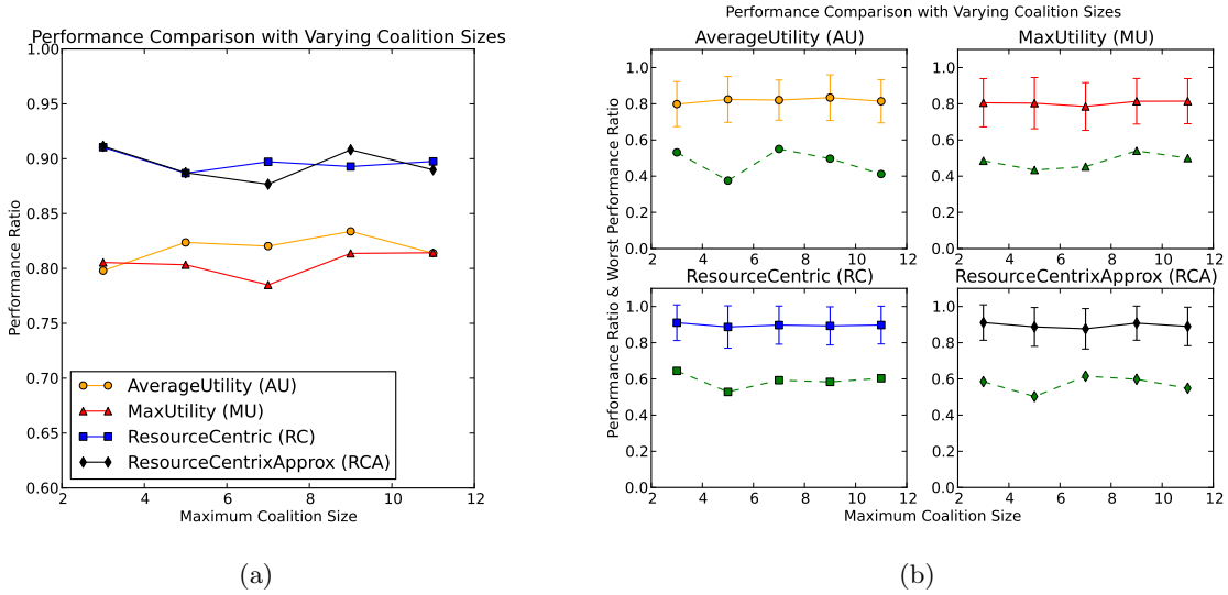
Figure 7.25: Task allocation with task dependences with varying coalition sizes. (a) Average performance ratios. (b) Separate and more detailed average performance ratios with standard deviations. The green data points in each subgraph represent the worst performance ratios for that respective method.
