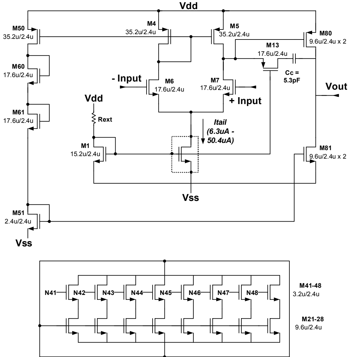
Figure 3.15: Tail-current adjustable slew-rate controlled op-amp
