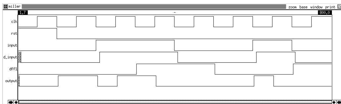
Figure 3.13: Simulation of the Miller encoder block
