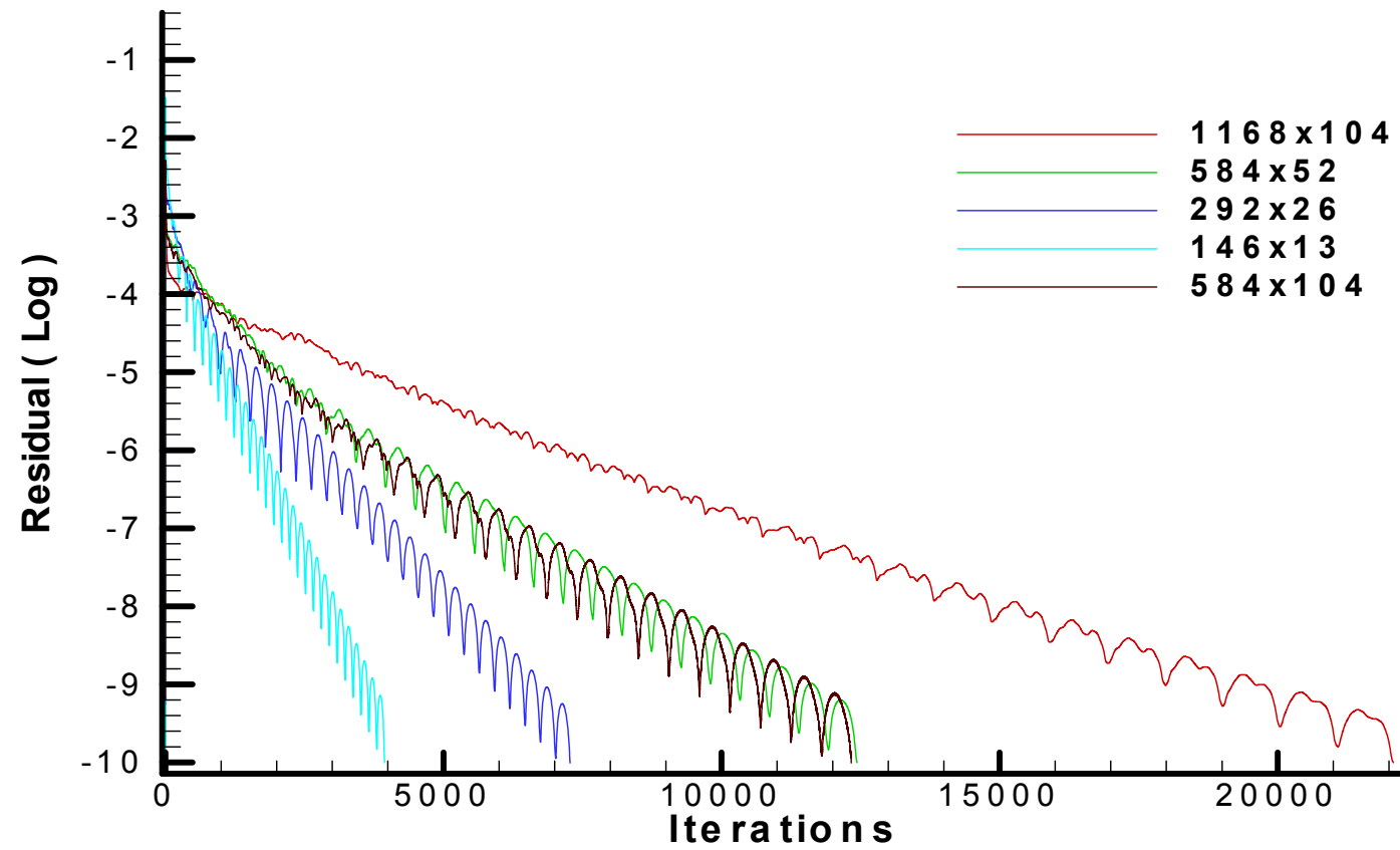
Figure 33: Oxygen Tube Convergence Comparison
