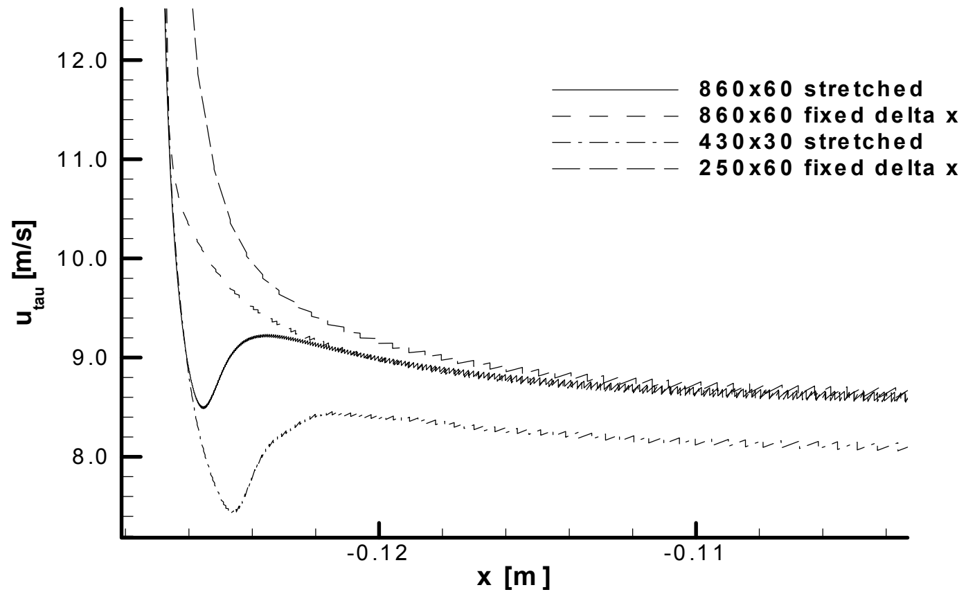
Figure 10: Hydrogen Annulus Friction Velocity Comparison
