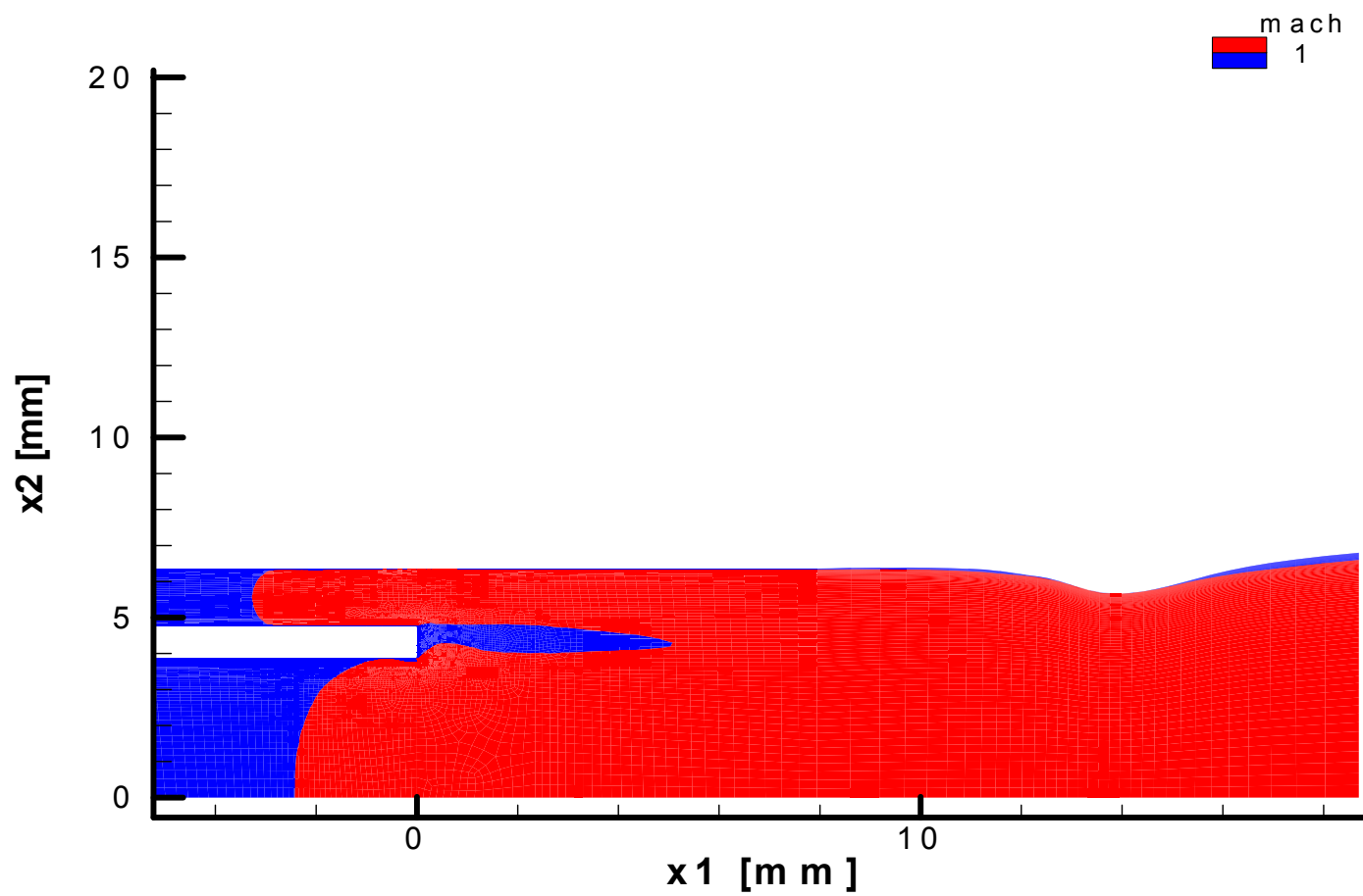
Figure 38: Sonic Line for Cold Flow Case
