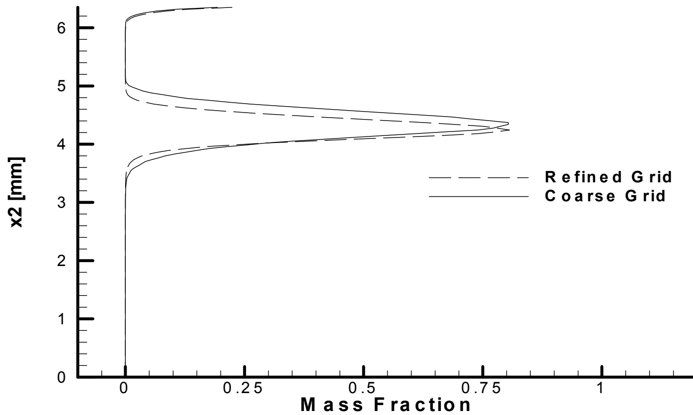
Figure 28: H_2O Profile Comparison in Chamber
