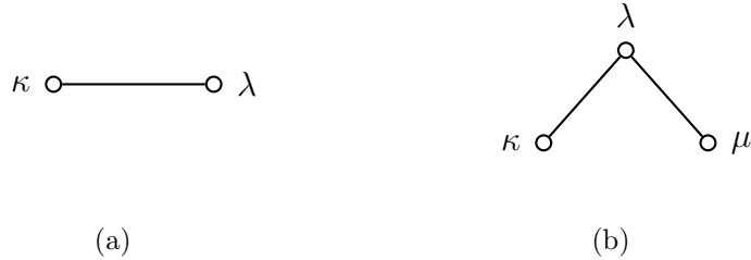
Figure 3.1: Representations of complete bipartite graphs
