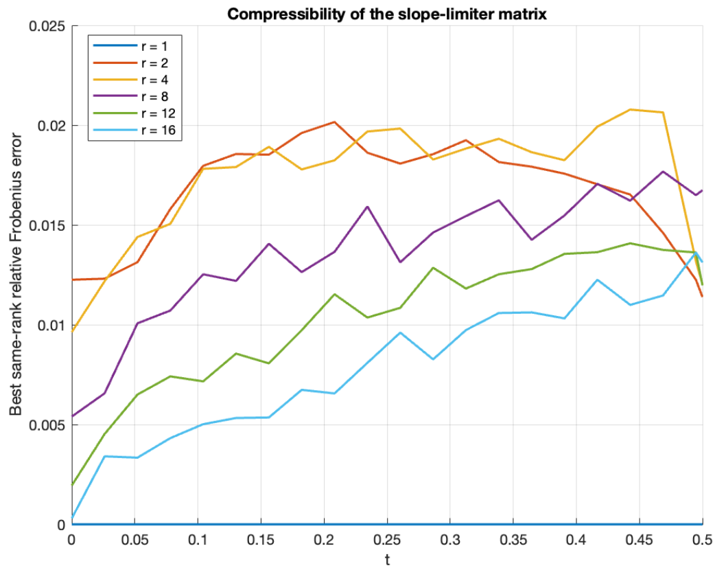
Figure 11.10: Same-rank compression error of the slope-limiter matrix for the smooth rank-two experiment. Each curve shows the best rank- r relative Frobenius approximation error of \Sigma(Y_r(t)) for the corresponding prescribed DLRA rank. Smaller values indicate greater compressibility at the state rank.
