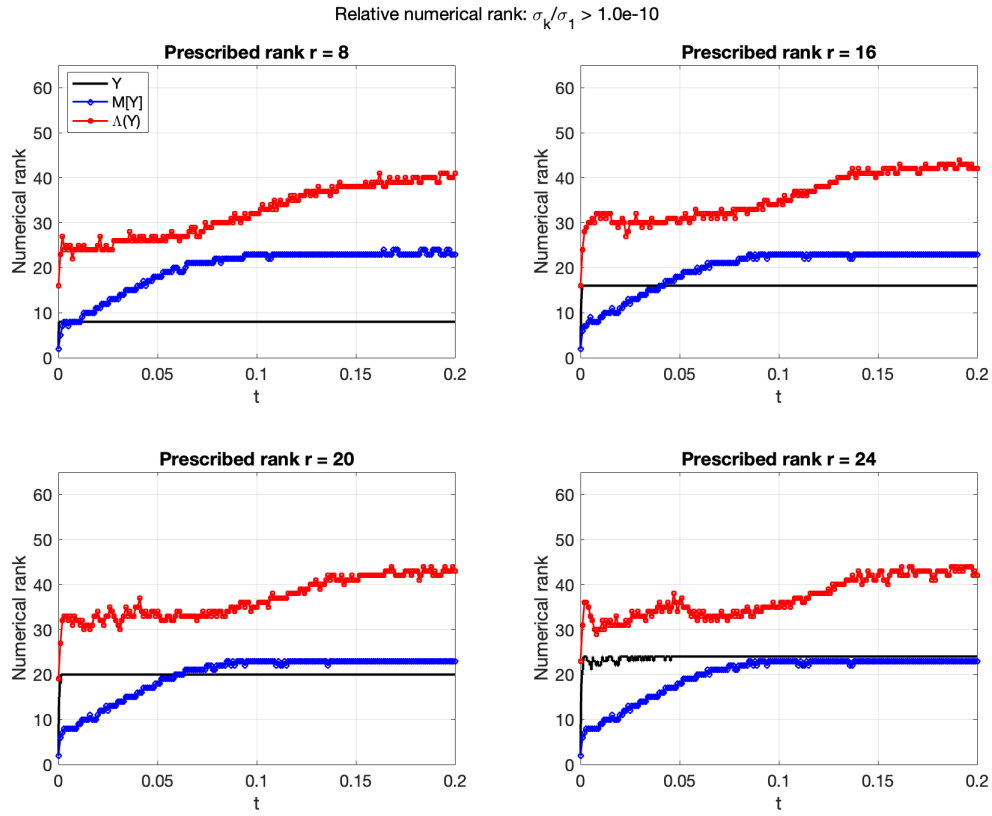
Figure 11.3: Numerical ranks of the DLRA approximation Y , the sampled Maxwellian M[Y] , and the slope-limiter matrix \Lambda[Y] for the Sod experiment with \varepsilon = 10^{-3} . Numerical rank is measured using the relative threshold \sigma_k/\sigma_1 > 10^{-10} .
