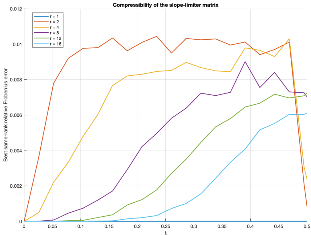
Figure 11.7: Same-rank compression error of the slope-limiter matrix for the smooth rank-one experiment. Each curve shows Equation (11.240) for a different prescribed DLRA rank. Smaller values indicate greater compressibility at the corresponding state rank.
