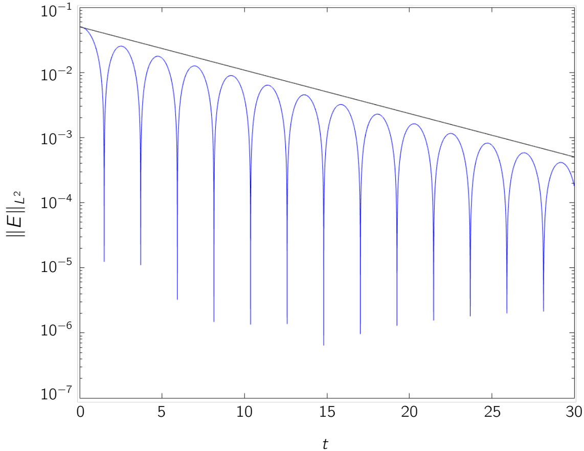
Figure 6.9: Landau damping for \alpha = 0.01 and k = 0.5 : the computed L^2 norm of the electric field follows the reference exponential decay rate -0.1533 over the displayed interval. A regression estimate and fit interval will be reported when the archived output data are regenerated.
