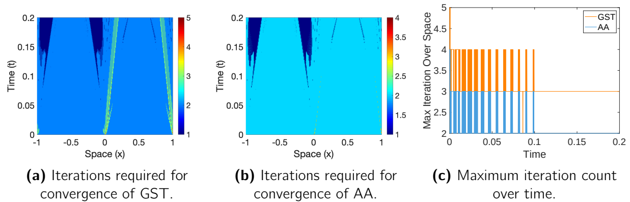
Figure 9.5: The number of iterations required for convergence is decreased by the application of Anderson Acceleration (AA) to the GST algorithm. The maximum iteration number over the spatial grid is strictly greater for the GST algorithm, compared to the Anderson Acceleration approach.
