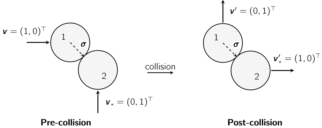
Figure 2.1: An equal-mass binary collision with \sigma = 2^{-1/2}(1, -1)^\top . The components parallel to \sigma are exchanged; in this particular configuration, the two velocity vectors are exchanged completely.
