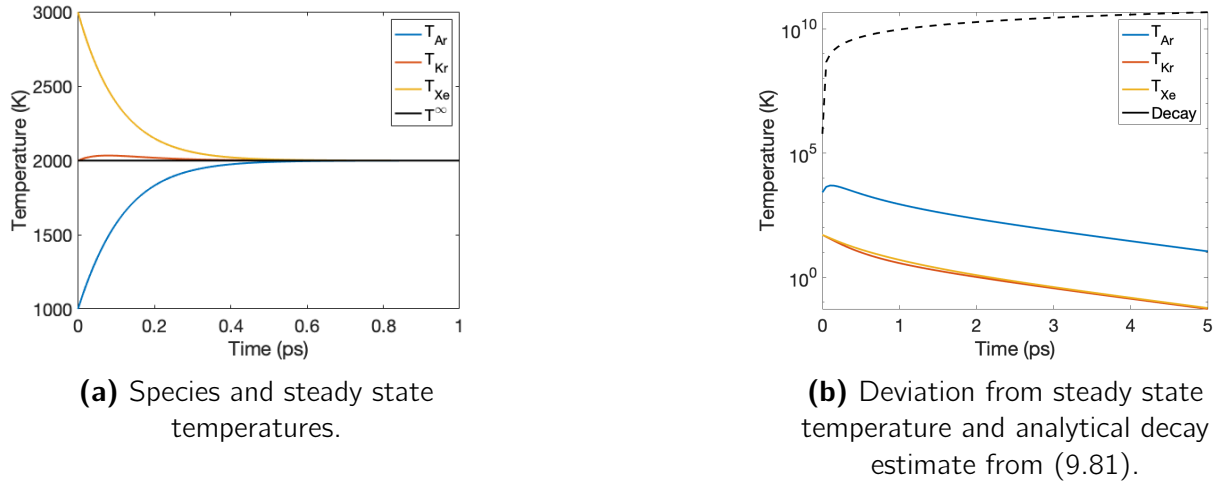
Figure 9.1: Temperature Decay of Ar–Kr–Xe Mixture in Example 1.
