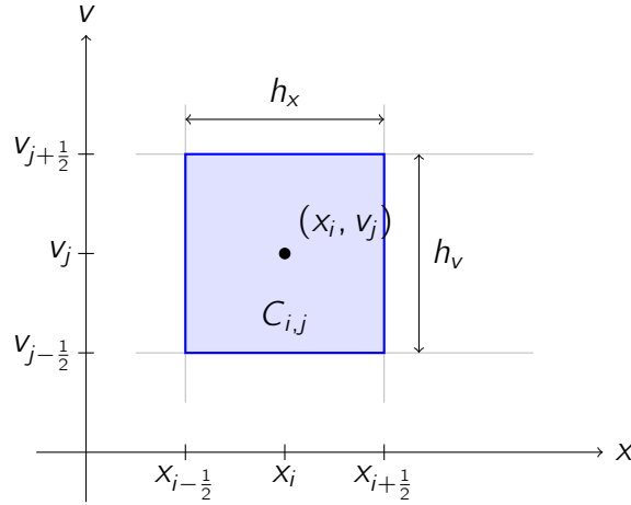
Figure 11.1: A finite-volume cell C_{i,j} in truncated phase space \Omega_x \times \Omega_v .
