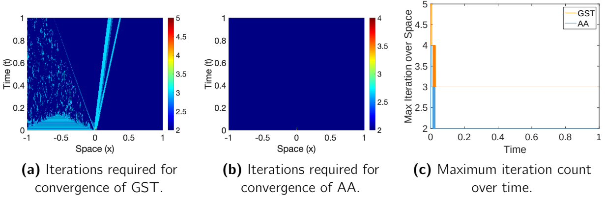
Figure 9.7: The number of iterations required for convergence is decreased by the application of Anderson Acceleration (AA) to the GST algorithm. The maximum iteration number over the spatial grid is strictly greater for the GST algorithm, compared to the Anderson Acceleration approach.
