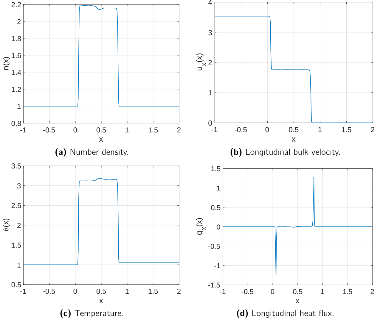
Figure 10.1: Moment profiles for the 1x2v ES–BGK slab problem at t_F = 0.25 with \varepsilon = 10^{-3} .
