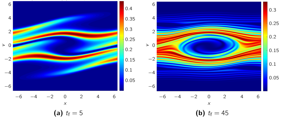
Figure 6.8: Two-Stream instability. The numerical solution is shown at t_f = 5 (left) and t_f = 45 (right). The numerical grid has N_v \times N_x = 800 \times 800 cells on the grid \Omega \times V = [-2\pi, 2\pi] \times [-2\pi, 2\pi] . The fine filamentation of the particle streams is adequately resolved and captured.
