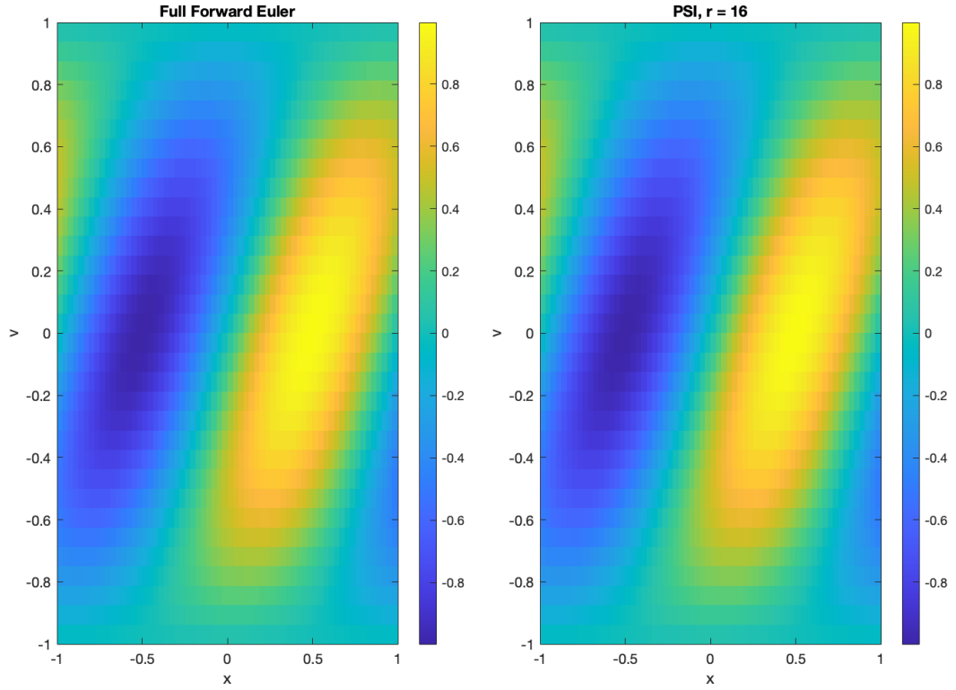
Figure 11.6: Final-time solutions for the smooth rank-one initial condition. The full-matrix Forward Euler solution is shown on the left, and the rank-16 projector-splitting approximation is shown on the right. Both calculations use the same slope-limited finite-volume spatial discretization and timestep.
