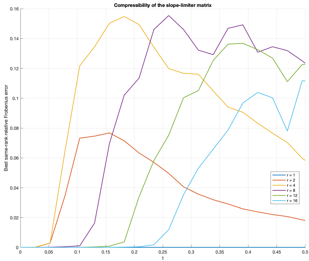
Figure 11.13: Same-rank compression error of the slope-limiter matrix for the discontinuous rank-one experiment. Compared with the smooth experiments, the larger errors show that the slope-limiter matrix is less accurately representable at the prescribed state rank.
