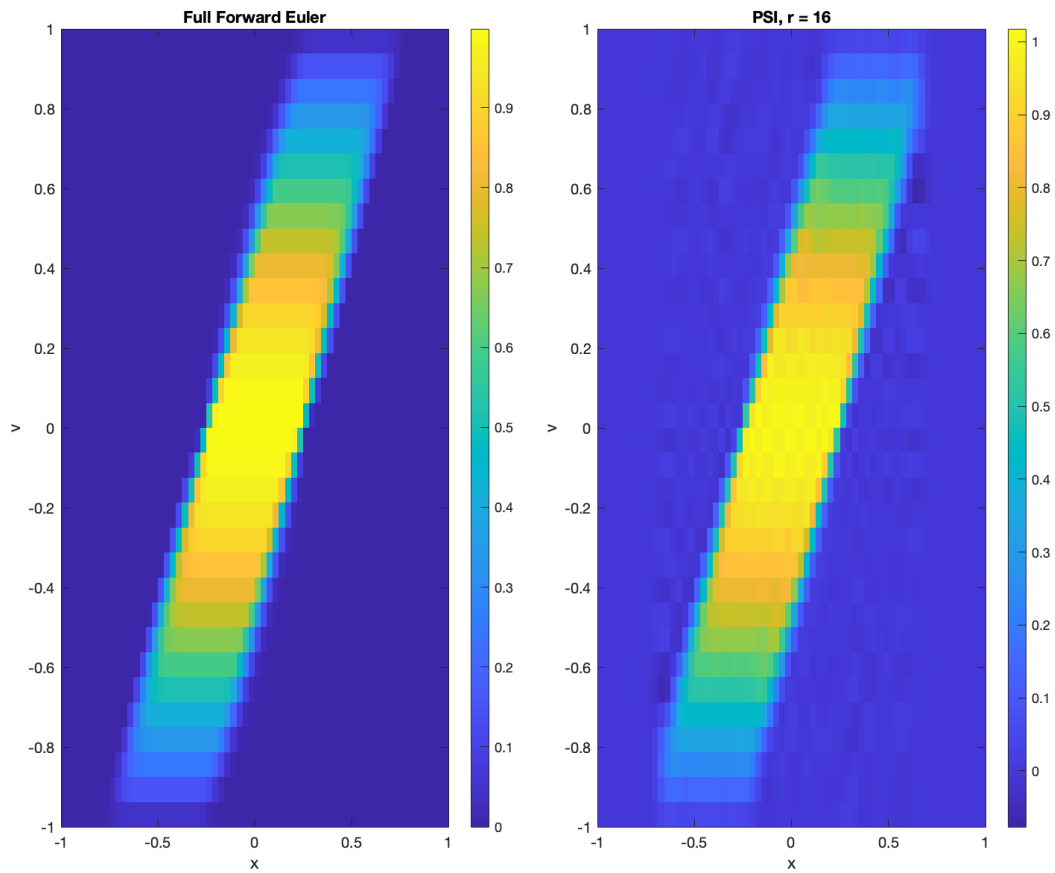
Figure 11.12: Final-time solutions for the discontinuous rank-one initial condition. The full-matrix Forward Euler solution is shown on the left, and the rank-16 projector-splitting approximation is shown on the right. The discontinuity produces considerably greater rank growth and a more demanding low-rank approximation problem than the smooth initial conditions.
