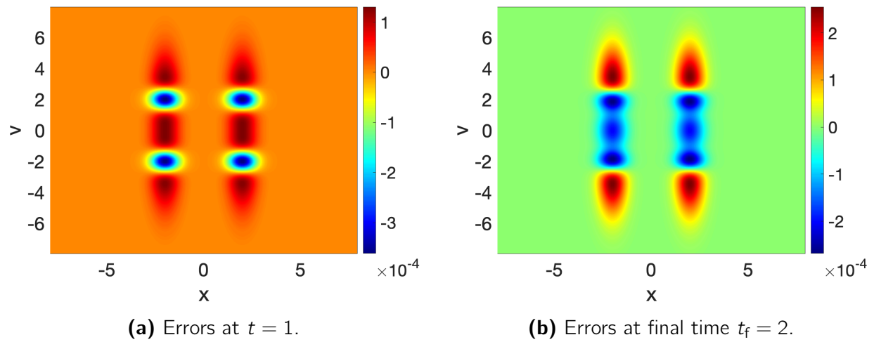
Figure 6.4: Relaxation Test 2: signed pointwise errors f_{\text{exact}} - f_{\text{num}} at t = 1 and t = 2 for \lambda = 1 and the four-Gaussian initial data (6.48).
