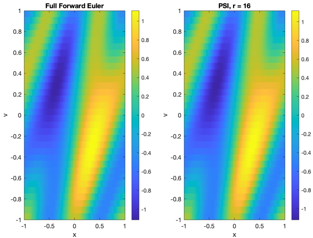
Figure 11.9: Final-time solutions for the smooth rank-two initial condition. The full-matrix Forward Euler solution is shown on the left, and the rank-16 projector-splitting approximation is shown on the right. Both calculations use the same slope-limited finite-volume spatial discretization and timestep.
