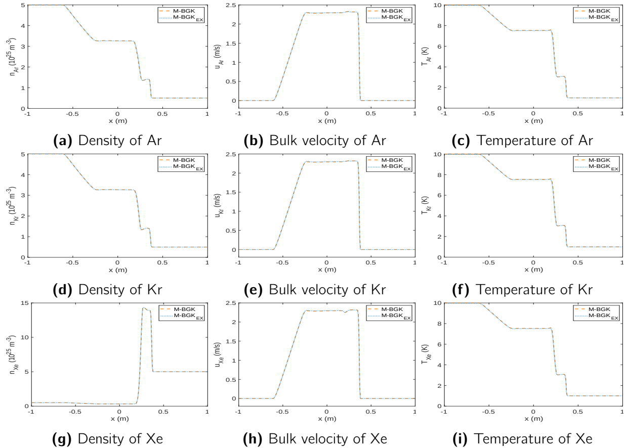
Figure 9.6: Noble gas mixture of Ar, Kr, and Xe: Moment plots of species number density, bulk velocity, and temperature, are given at t_f = 1 \mu\text{s} , for a mixture with \varepsilon \approx 0.00103 . M-BGK uses the GST algorithm for the moment solve. M-BGK EX uses a fully explicit method.
