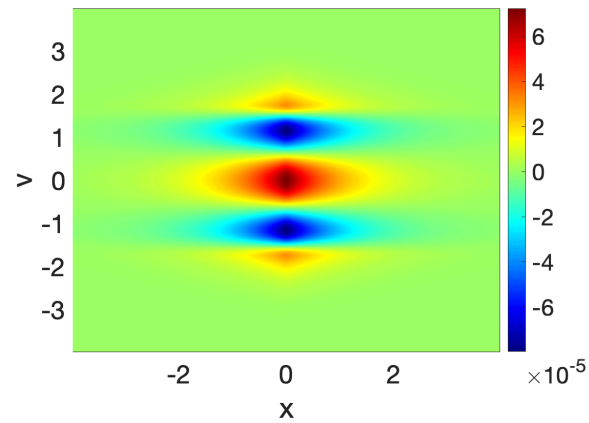
Figure 6.2: Relaxation Test 1: signed pointwise error f_{\text{exact}} - f_{\text{num}} at t_f = 1 for \lambda = 1 and N_x = N_v = 128 . The displayed error has magnitude \mathcal{O}(10^{-5}) .
