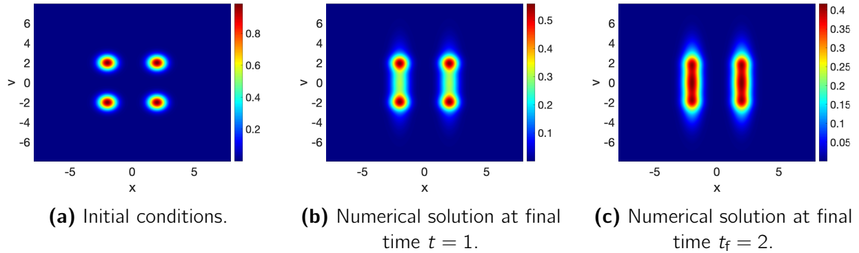
Figure 6.3: Relaxation Test 2 for the space-homogeneous BGK model (5.24): four-Gaussian initial data (6.48) and numerical solutions at t = 1 and t = 2 . Here \lambda = 1 , and the initial moments are evaluated with the trapezoidal rule.
