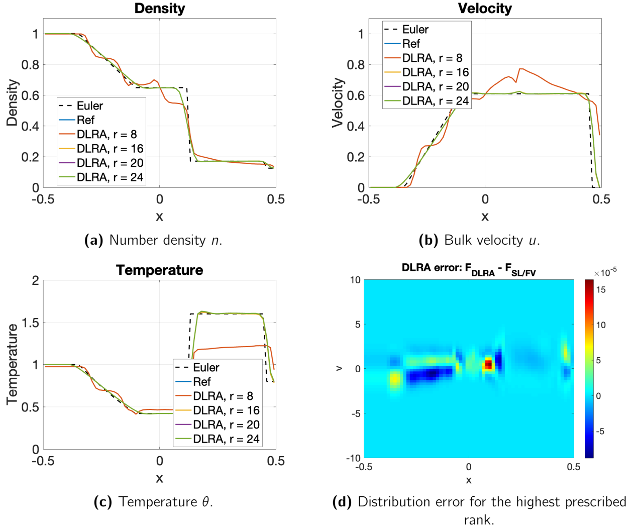
Figure 11.4: Macroscopic quantities and distribution error for the one-dimensional Sod experiment with \varepsilon = 10^{-4} . The DLRA results are compared with the slope-limited full finite-volume reference solution.
