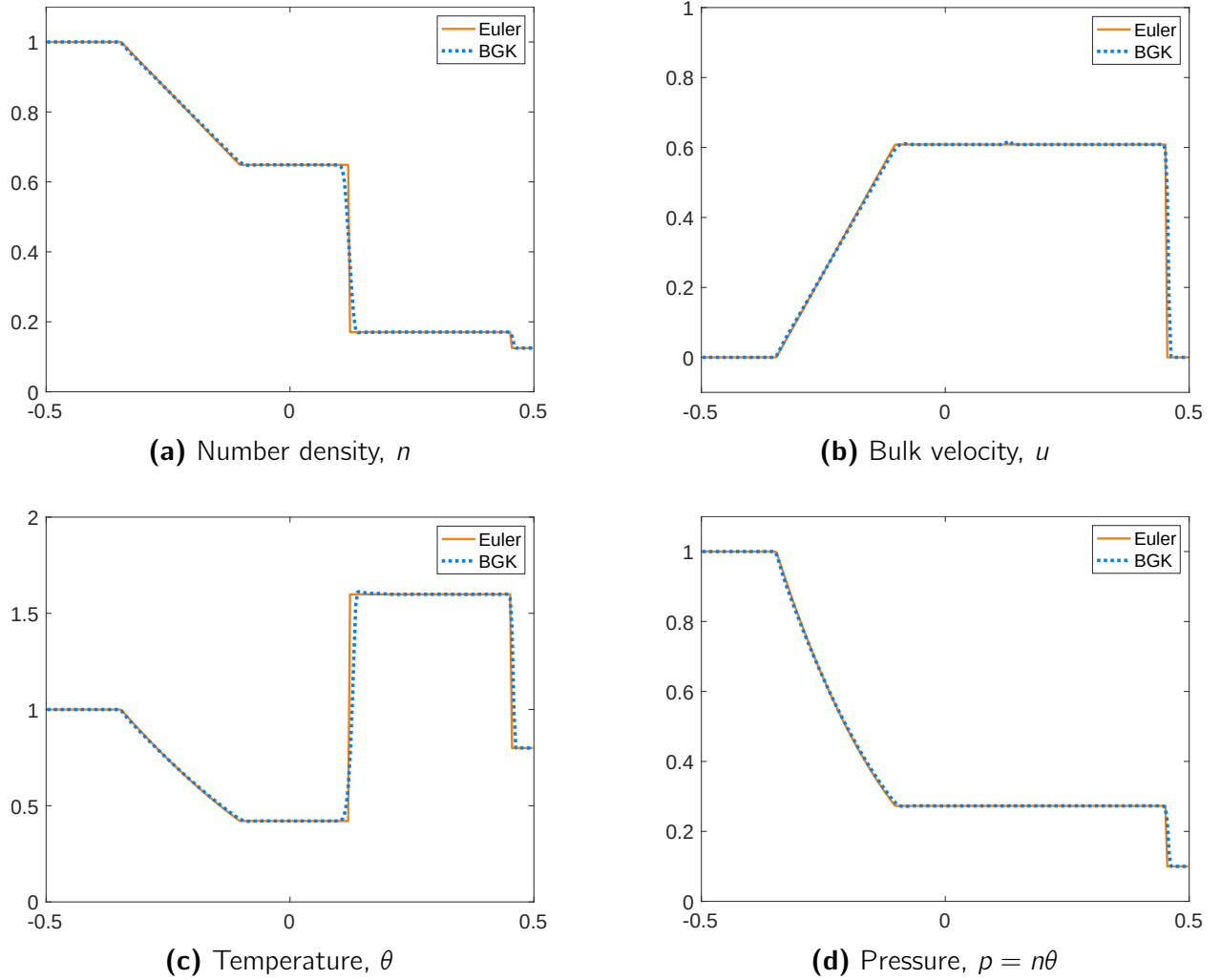
Figure 6.6: Sod shock tube at t_f = 0.2 with \tau = 10^{-4} : BGK moments (number density, bulk velocity, temperature, and pressure) compared with the exact Euler Riemann solution. The agreement tests the highly collisional Euler limit; a norm-based mesh study is reserved for the code-verification pass described in Table 6.1.
