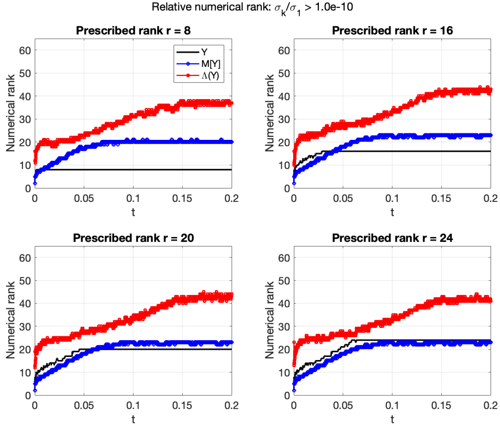
Figure 11.5: Numerical ranks of the DLRA approximation Y , the sampled Maxwellian M[Y] , and the slope-limiter matrix \Lambda[Y] for the Sod experiment with \varepsilon = 10^{-4} . Numerical rank is measured using the relative threshold \sigma_k/\sigma_1 > 10^{-10} .
