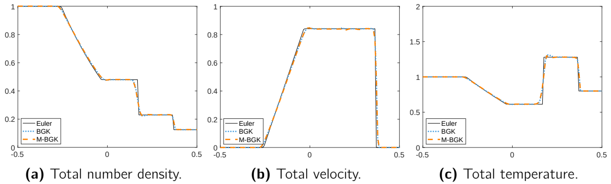
Figure 9.4: The total density, total bulk velocity, and total temperature moments are compared to the solution of the Euler equations at time t = 0.2 , with \varepsilon = 10^{-4} .
