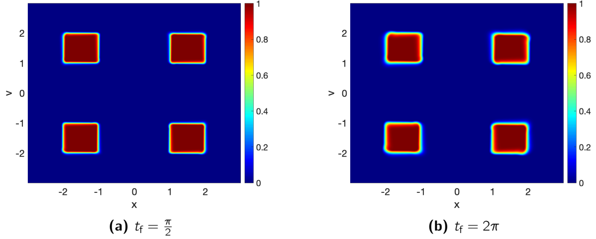
Figure 6.7: Rotation Problem: \frac{\partial}{\partial t} f + v \frac{\partial}{\partial x} f - x \frac{\partial}{\partial v} f = 0 . Grid: N_v = N_x = 400 .
