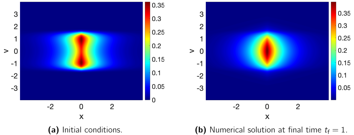
Figure 6.1: Relaxation Test 1 for the space-homogeneous BGK model (5.24): initial data (6.47) (left) and the numerical solution at t_f = 1 (right). Here \lambda = 1 and N_x = N_v = 128 .
