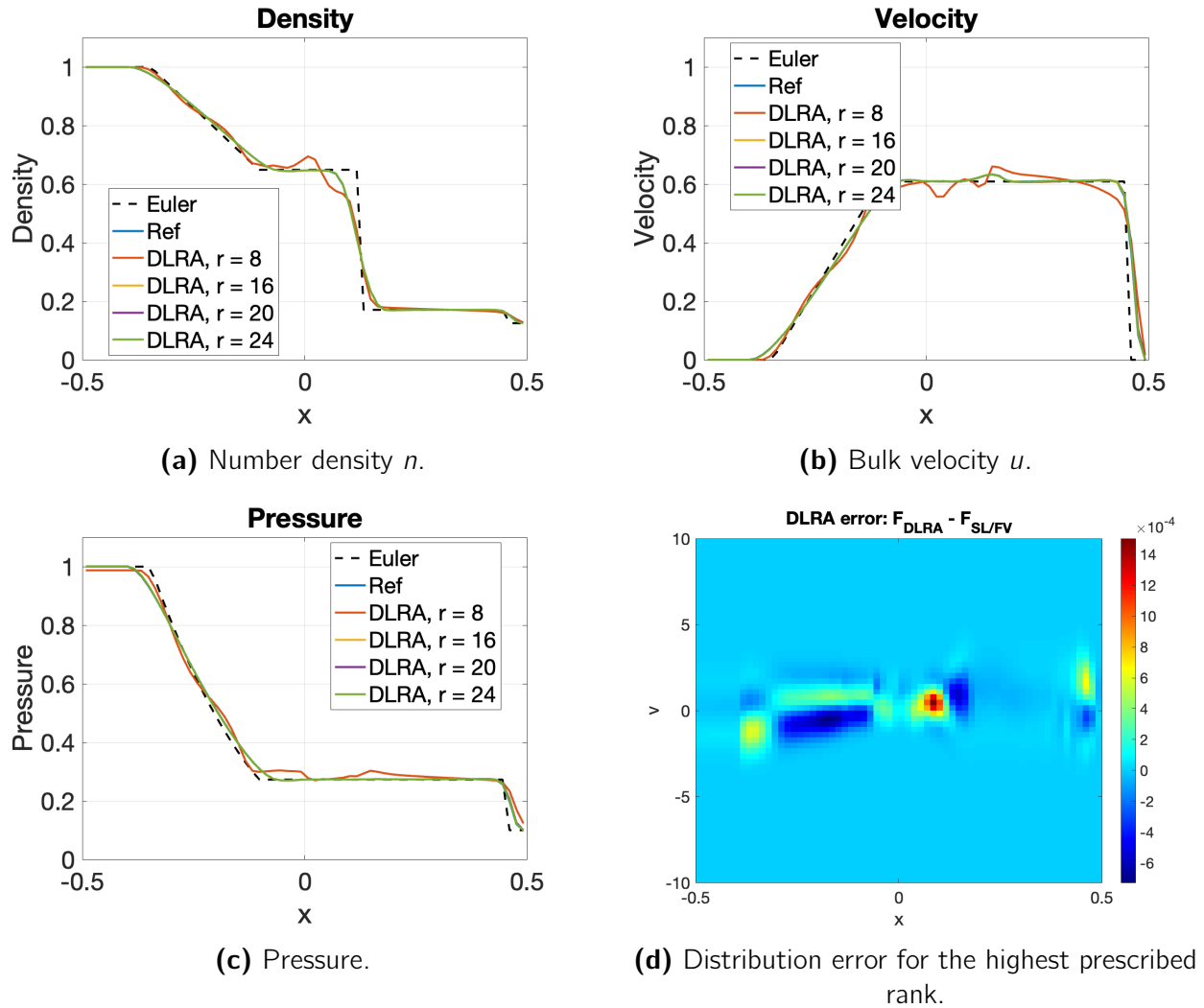
Figure 11.2: Macroscopic quantities and distribution error for the one-dimensional Sod experiment with \varepsilon = 10^{-3} . The DLRA results are compared with the slope-limited full finite-volume reference solution.
