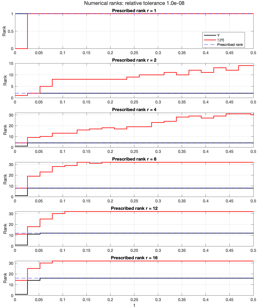
Figure 11.14: Numerical-rank histories for the state matrix Y_r(t) and the slope-limiter matrix \Sigma(Y_r(t)) in the discontinuous rank-one experiment. Numerical ranks are computed using the relative criterion \sigma_k/\sigma_1 > 10^{-8} . The numerical rank of the limiter matrix grows rapidly, particularly for the higher-rank state approximations.
