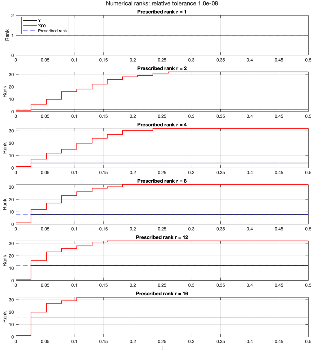
Figure 11.8: Numerical-rank histories for the state matrix Y_r(t) and the corresponding slope-limiter matrix \Sigma(Y_r(t)) in the smooth rank-one experiment. Numerical ranks are computed using the relative criterion \sigma_k/\sigma_1 > 10^{-8} . Although the projector-splitting approximation maintains the prescribed state rank, the entrywise minmod operation generally produces a slope-limiter matrix of substantially higher numerical rank.
