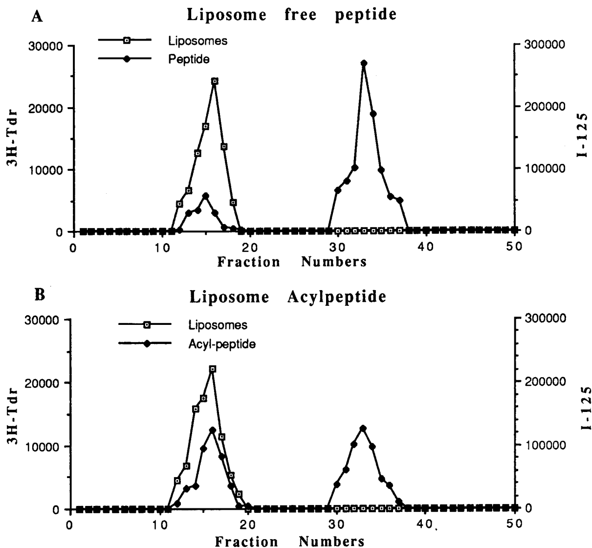
Figure 1: INCORPORATION OF FREE AND ACYLPEPTIDE INTO LIPOSOMES
