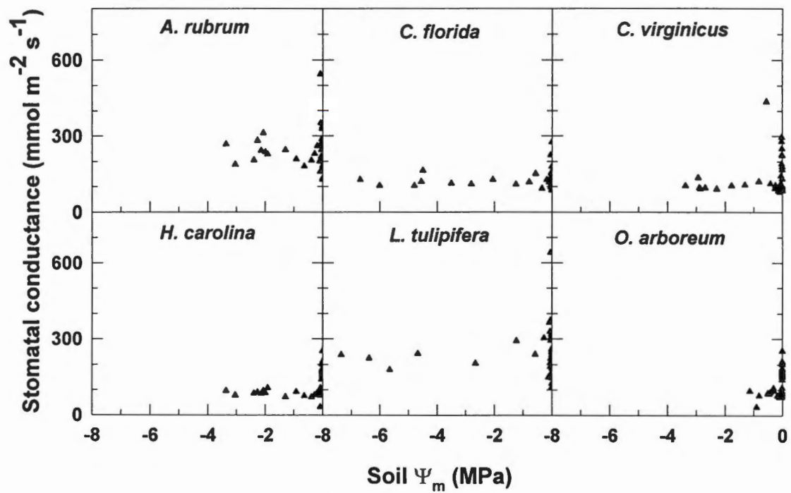
Figure 3-9. Stomatal conductance of WD saplings as soil \Psi_m declined to lowest values reached during the drying period. Points represent daily means ( n = 8 ).
