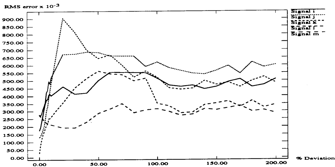
Figure 3.11: Avg. RMS error vs. % Deviation from Ideal v_k (nonperiodic)
