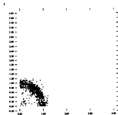
Figure 3.19: Normalization of 784 points with RBFs of size 0.125
