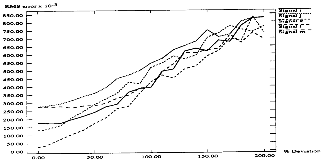
Figure 3.10: Avg. RMS error vs. % Deviation from Ideal c_k (nonperiodic)
