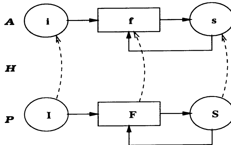
Figure 1.1: Physical Realization of an Abstract Process
