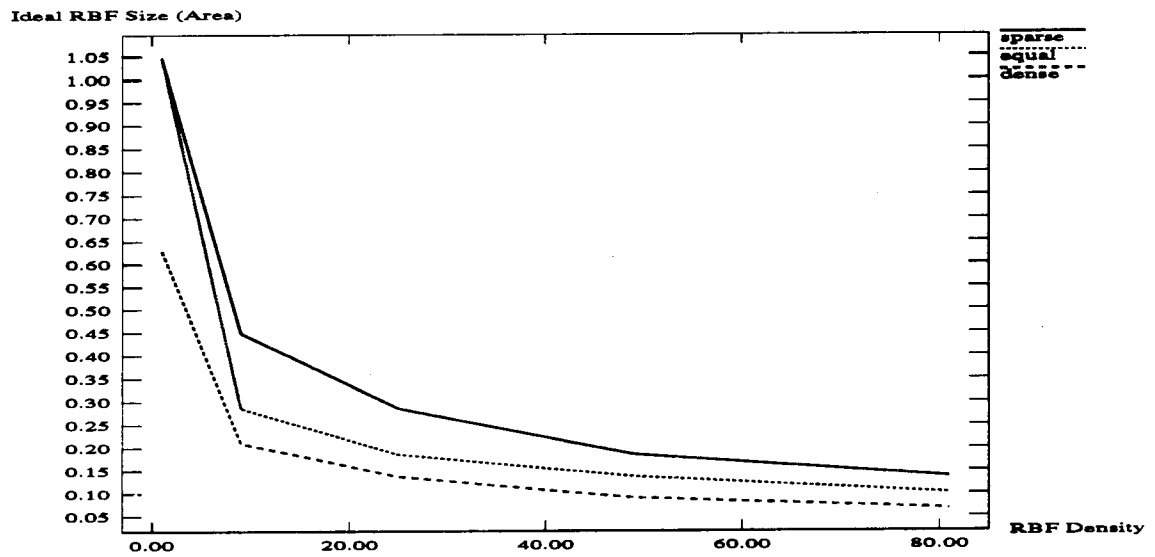
Figure A.4: Ideal RBF Size vs. RBF Density, varying data density (LN)
