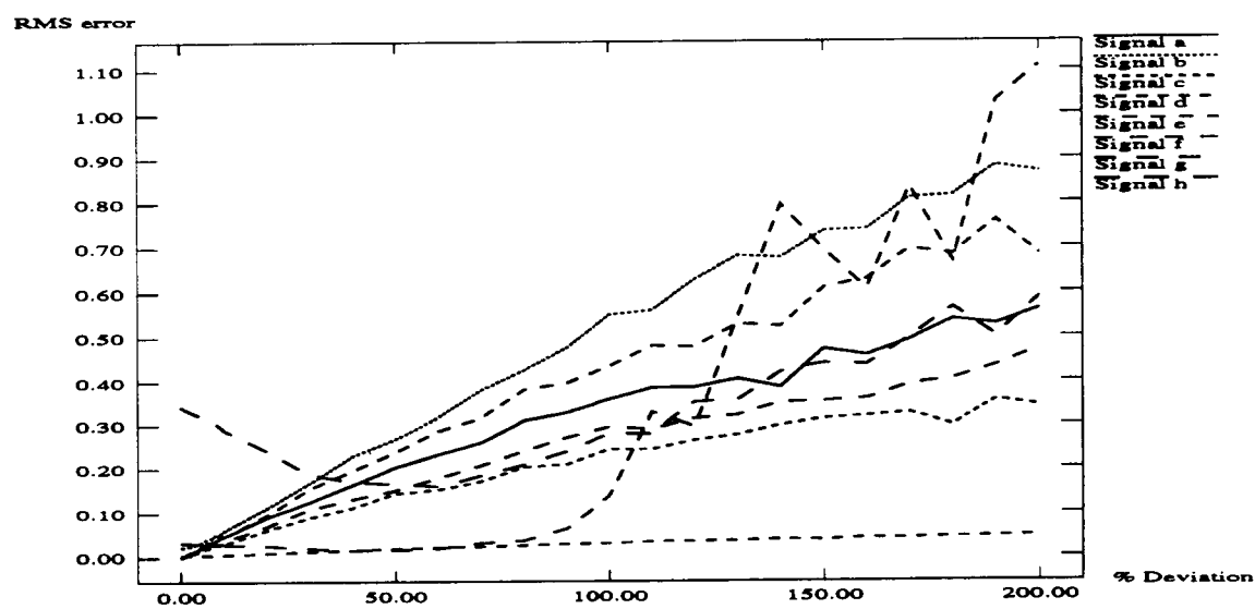
Figure 3.4: Avg. RMS error vs. % Deviation from Ideal c_k
