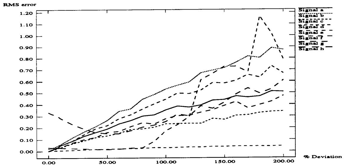
Figure 3.16: Avg. RMS error vs. % Deviation from Final c_k
