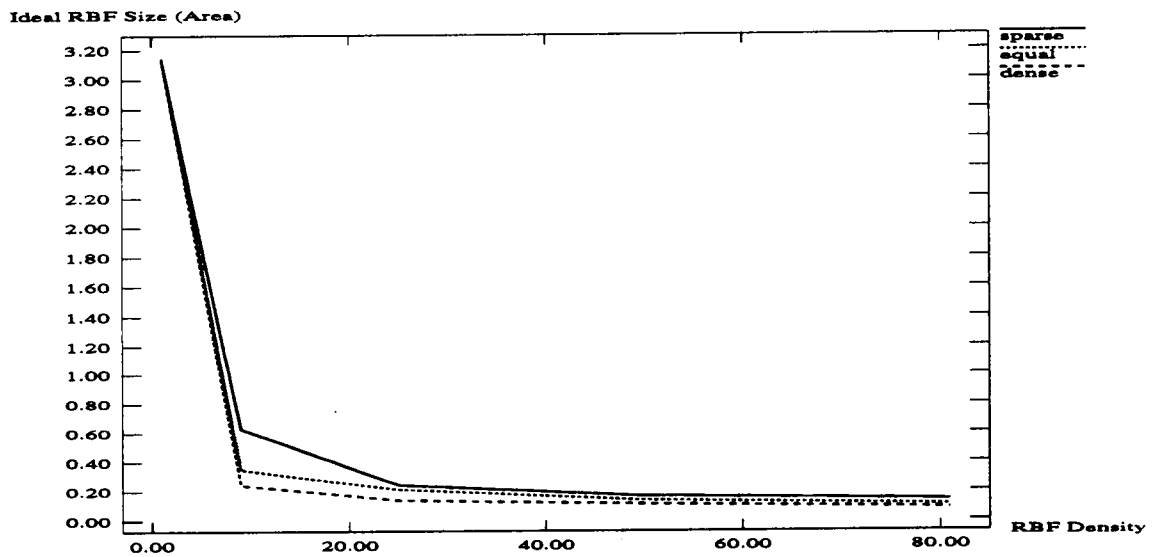
Figure A.2: Ideal RBF Size vs. RBF Density, varying data density (GD)
