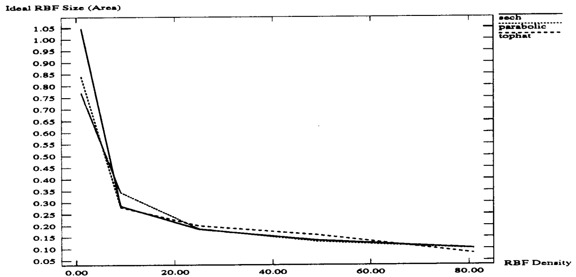
Figure A.3: Ideal RBF Size vs. RBF Density, varying RBF type (LN)
