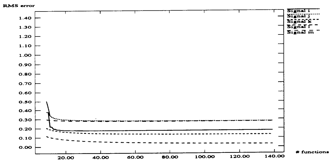
Figure 3.9: Avg. RMS error vs. #Basis Functions (nonperiodic)
