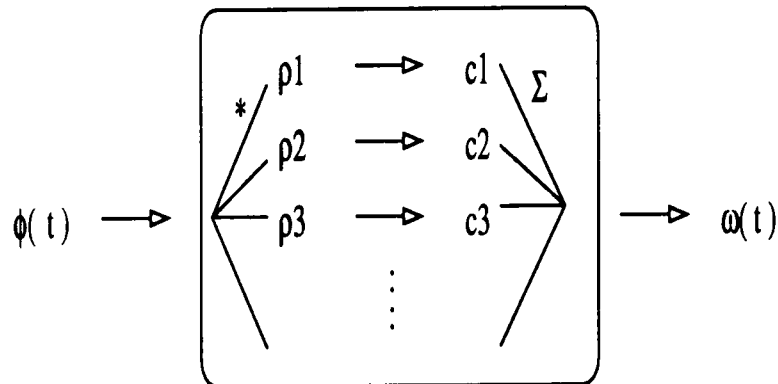
Figure 2.4: Schematic of Matched Filter System
