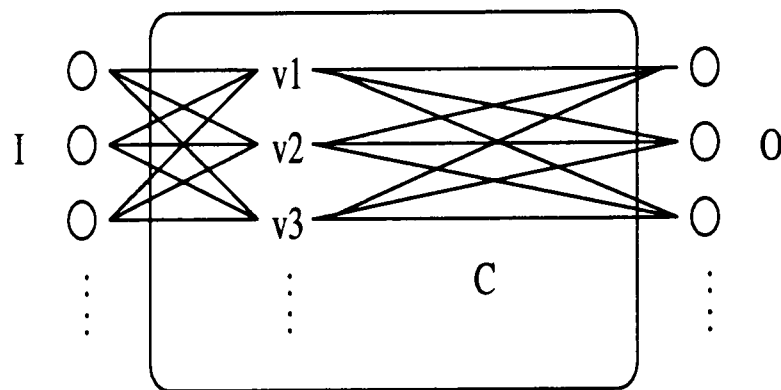
Figure 2.8: Schematic of Layered Correlational System
