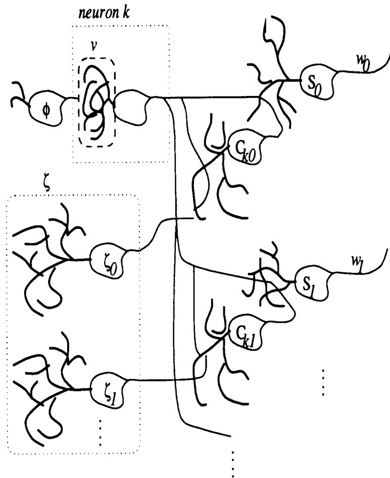
Figure 2.9: Possible Neural Implementation of Layered Correlational System
