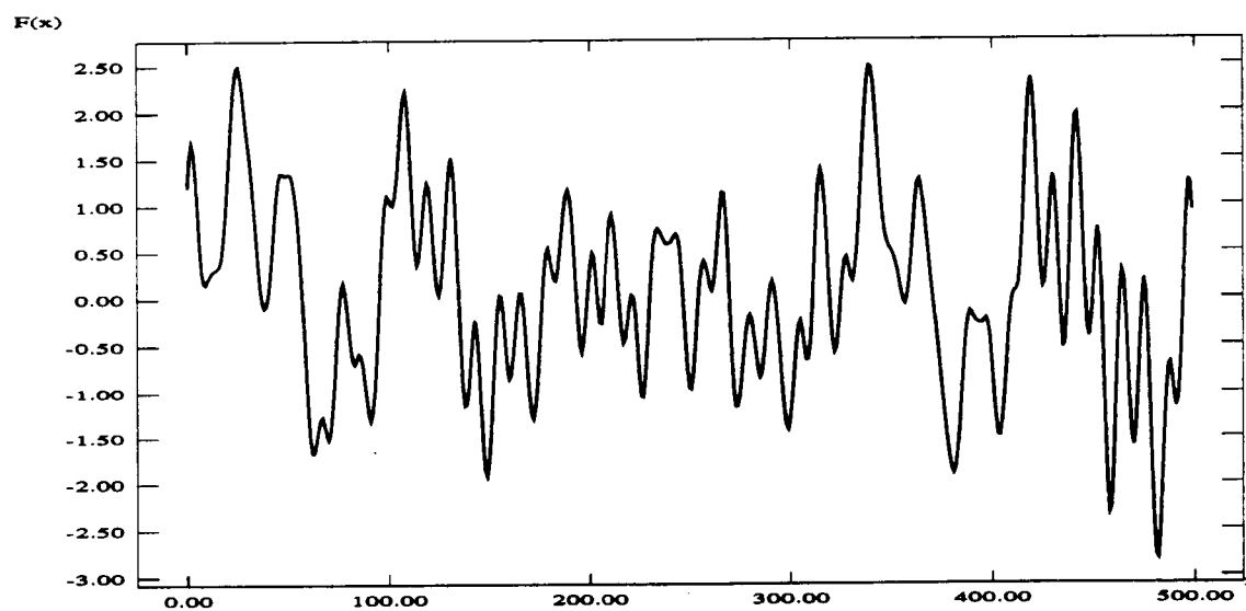
Figure 3.13: Learned b(x) with Deviation from v_k of 10%
