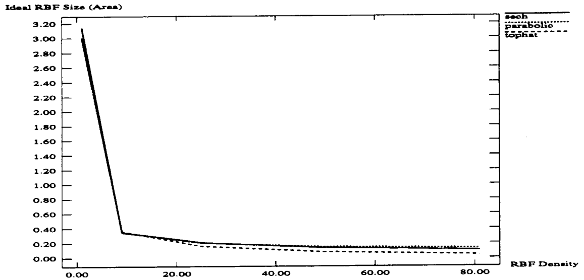
Figure A.1: Ideal RBF Size vs. RBF Density, varying RBF type (GD)
