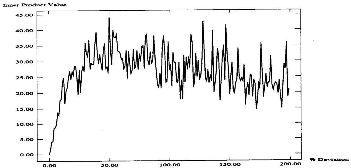
Figure 3.14: Avg. Inner Product between Basis Pairs vs. \%v_k deviation
