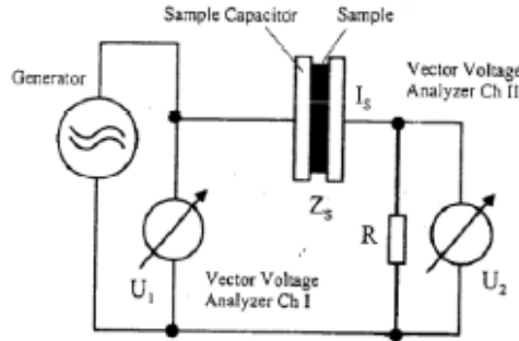
Figure 3.4. Schematic for the measurements of the complex dielectric permittivity of liquid samples using the Novocontrol Concept 80 system. 119
