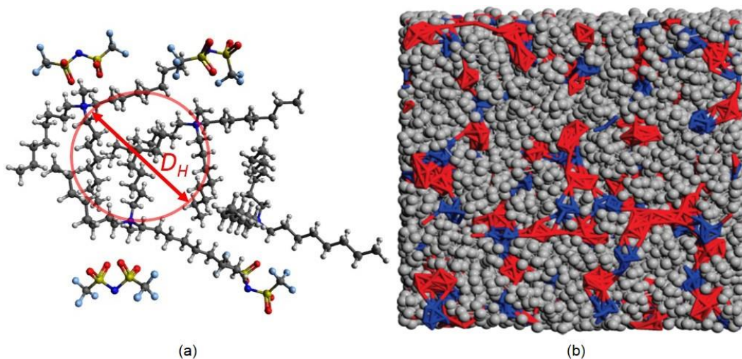
Figure 5.7. (a) A classical, energy-minimized chemical model of four ion pairs of [N8881][NTF 2 ] is shown with the corresponding hydrodynamic diameter calculated using the Debye-Stokes-Einstein relation. (b) Classical, atomistic MD simulation snapshots of 150 ions of [N8881][NTF 2 ]. The segregation of alkyl domains (grey spheres) from the charge rich domains (red (-) and blue (+)) is clearly observed. 110
