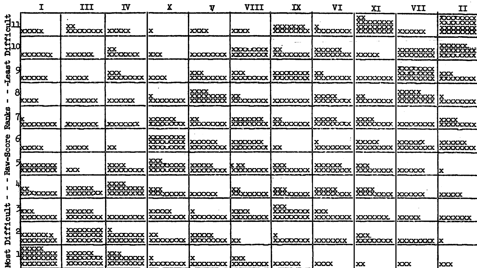
Figure 2. Raw-Score Ranks of 11 Problem Areas as Perceived by 117 Data Processing Administrators: Total Population (Scattergram)
