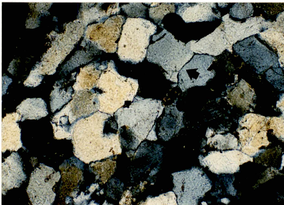
Figure 5.7. Thin-section photomicrograph, under cross-polarized light, of sample FG-1 from Flat Gap, TN (Locality FG in Figure 1.2) illustrating pressure-solution features such as concave/convex grain boundaries (arrow) and quartz overgrowths. Such features are common to the FGB variant and in the associated pebble lags. Field of view is 2.3 mm in the long dimension.
