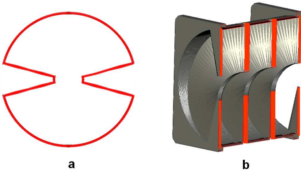
Figure 2.4: A longitudinal helical analog to the disk-loaded slow-wave structure. (a) shows the transverse cross section, while (b) shows a cutaway view of the 3D twisted structure.
