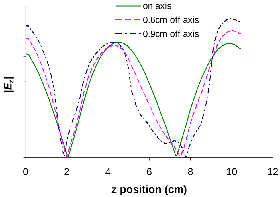
Figure 5.5: Magnitude of \mathbf{E}_z for on-axis and off-axis particles: CST simulation
