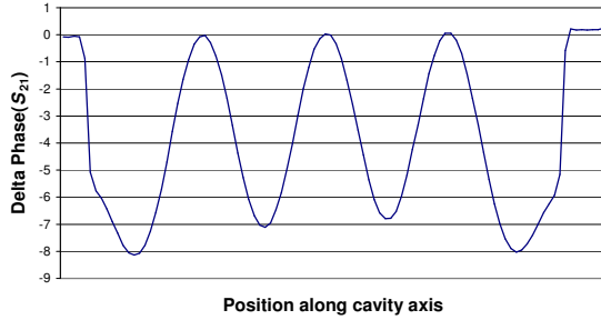
Fig. 10. Bead pull measurement of a 2.8 GHz TM mode of the “keyhole” twisted structure
