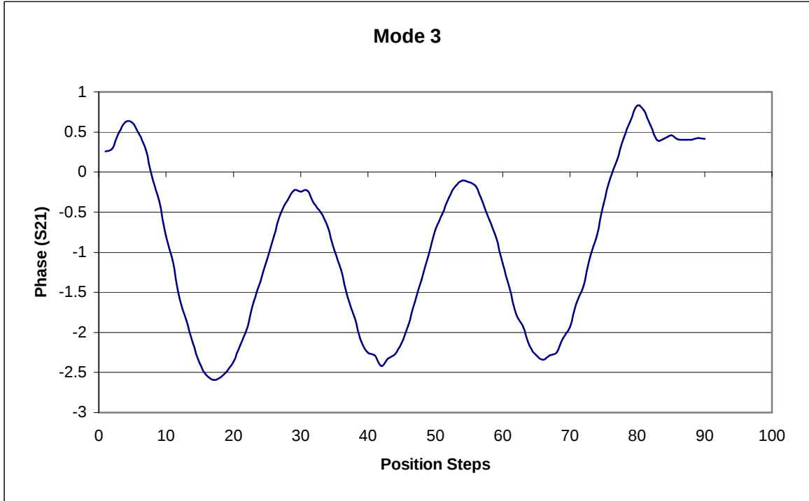
Figure 6.5: Bead pull measurement of the large twisted rectangular prototype for third mode. Measurements for other modes were similar, except with different number of cycles.
