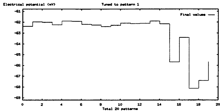
Figure D.4: Final values of the dendritic net tuned to pattern 1 for all input patterns
