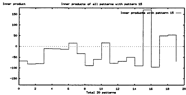
Figure D.31: Cross inner products of all patterns with pattern 15
