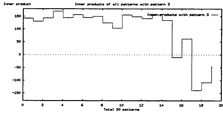
Figure D.7: Cross inner products of all patterns with pattern 3
